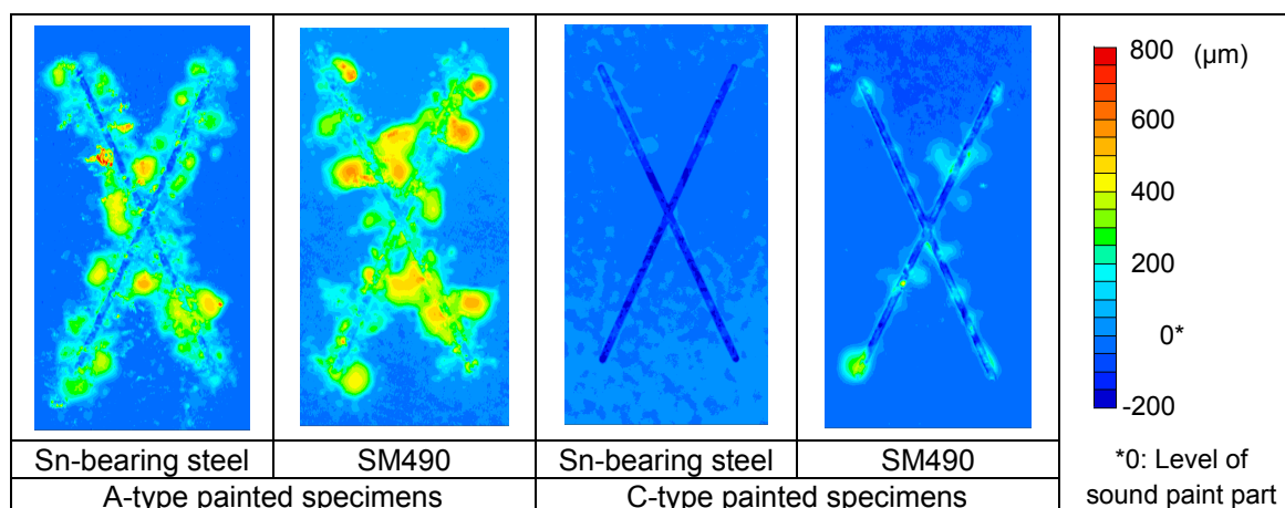
Figure 4: Blister around cross scribe regions (after the test of 1200 cycles)
