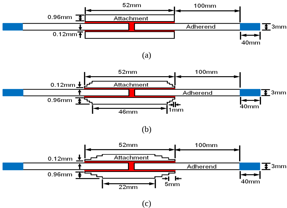
Fig. 1 Design of double lap joint ((a) conventional joint (DLJ), (b) stepwise patch joint (SDLJ-1) (c) stepwise patch joint (SDLJ-2)
