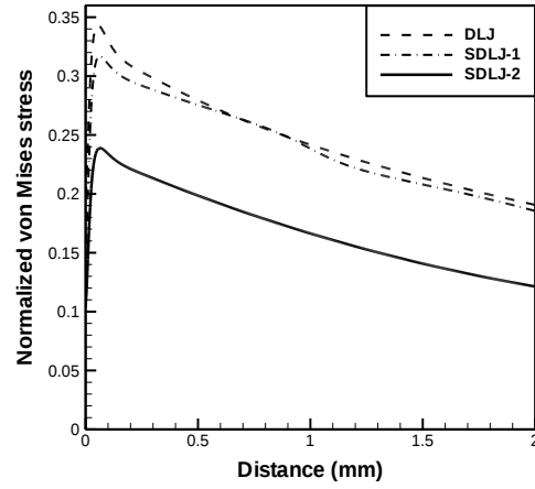
Fig. 7 Normalized von Mises stress distribution in the adhesive layer
