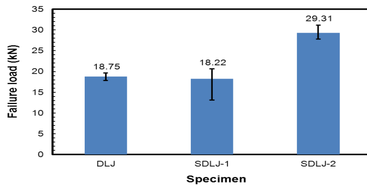
Fig. 3 Failure loads of the double lap joints.
