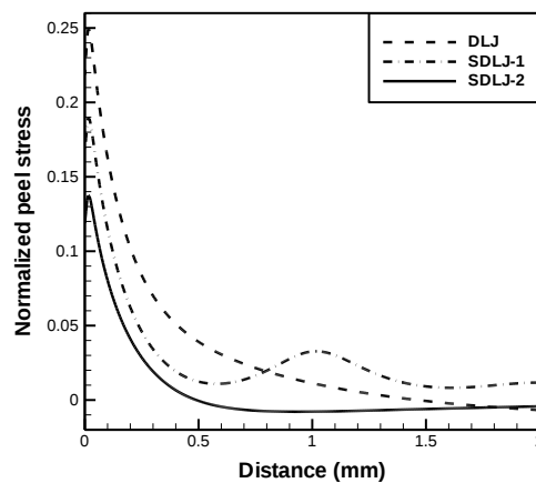
Fig. 5 Normalized peel stress distribution in the adhesive layer
