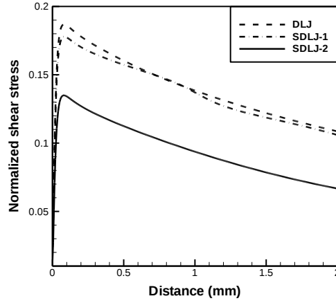
Fig. 6 Normalized shear stress distribution in the adhesive layer
