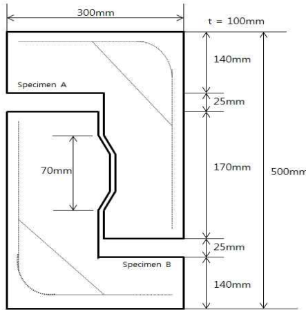
Figure 1: Details of specimen.
