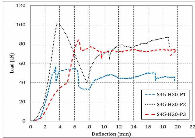
Figure 3: Load-deflection curve (S45-H20 series).
