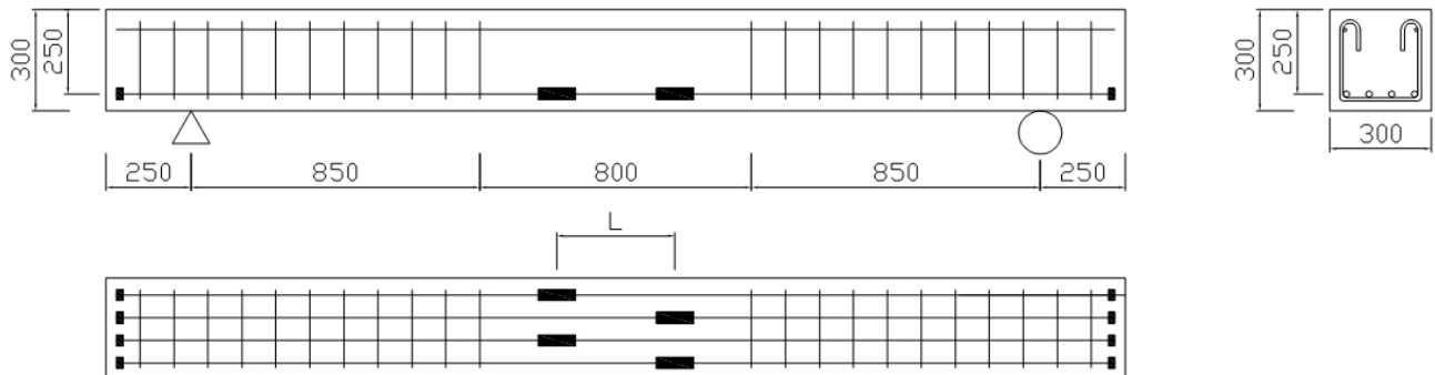
Figure 4: Beam dimensions (in mm)
