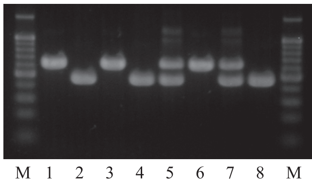
Fig. 1. Electrophoretic profiles of the Pg118 codominant marker in adzuki bean accessions/cultivars and segregants in the cross between 'Symari' and 'Buchishoryukei-1'. M: 100 bp ladder size marker, 1: Syumari, 2: Buchishoryukei-1, 3: Kitano-otome, 4: Erimoshozu, 5: heterozygous genotype, 6: resistant genotype, 7: heterozygous genotype, 8: susceptible genotype.
