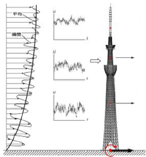
Figure 5: Time history response analysis with an artificial wind fluctuation data
