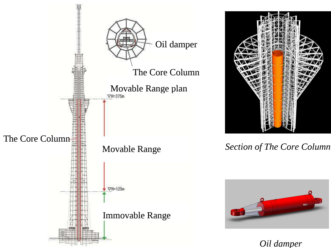
Figure 7: Notion of the response control system with The Core Column
