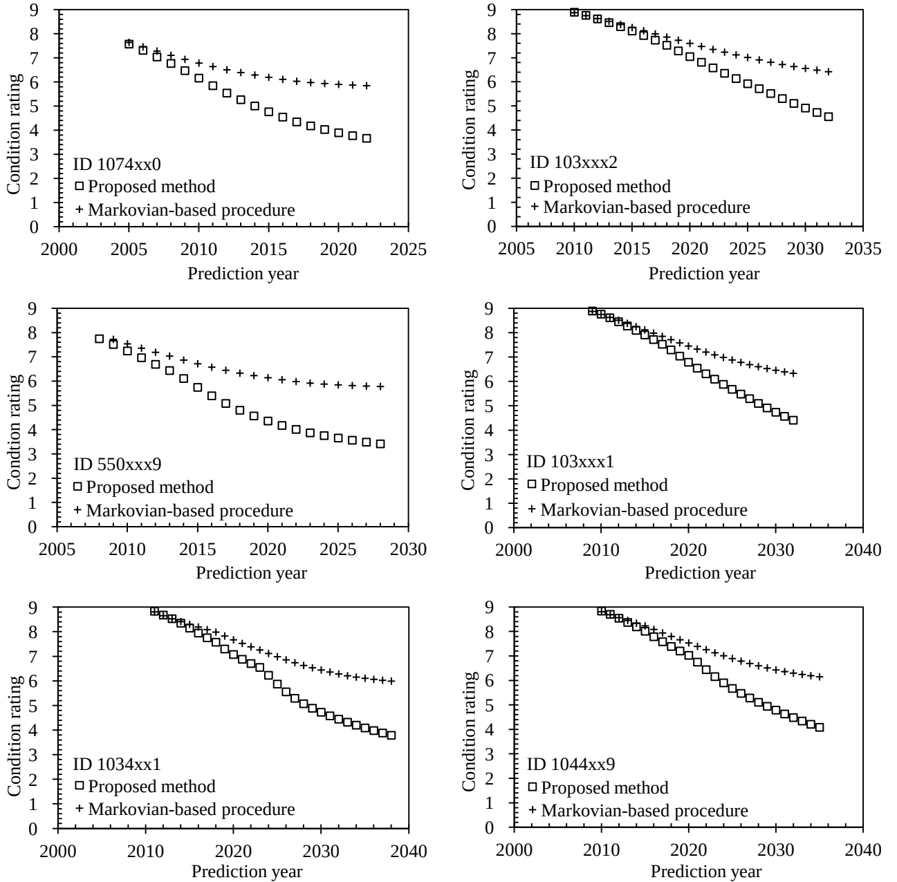
Figure 3. Comparisons of long-term deterioration predictions
