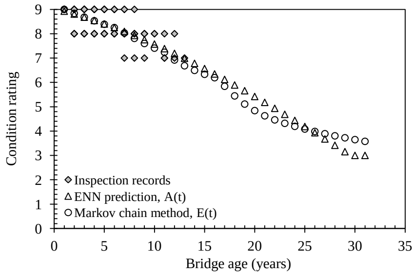
Figure 1: Data distribution and bridge performance curves for freeway network of the 1991-2010 construction era
