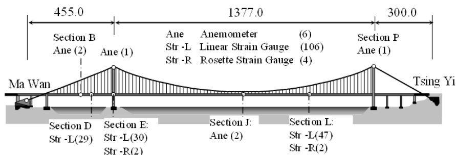
Figure 2: Distribution of dynamic strain gauges and anemometers in Tsing Ma Bridge
