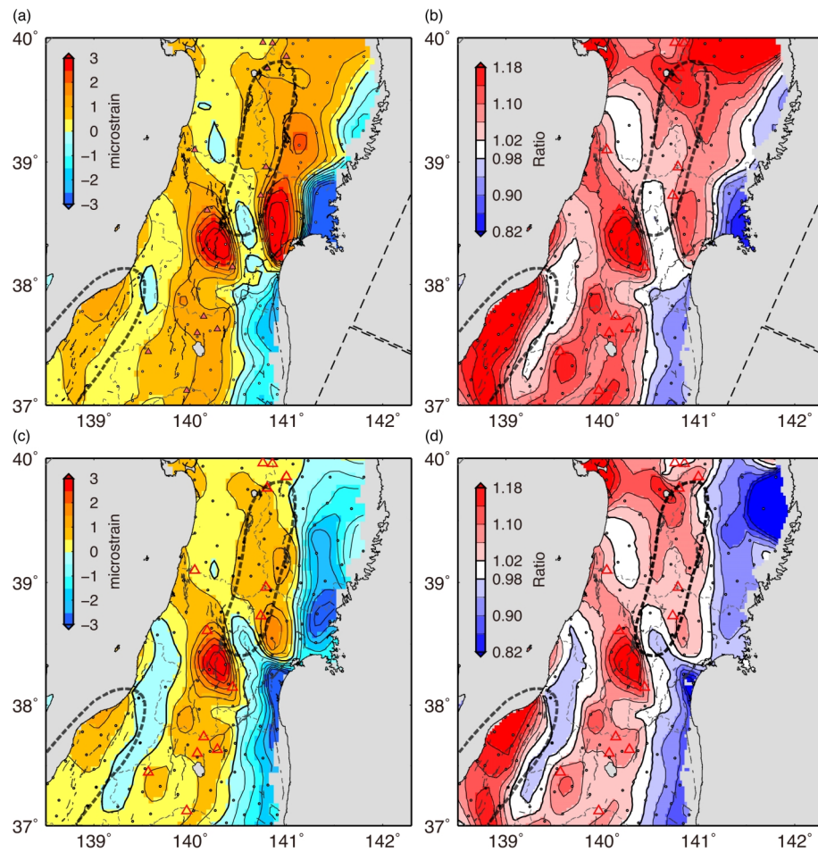
Fig. 7. (a) and (b) same as Fig. 5(a) and Fig. 5(d), respectively, but the estimation is obtained from a fault model based on Nishimura et al. (2011). (c) and (d) same as Fig. 5(a) and Fig. 5(d), respectively, but the estimation is obtained from the fault model of Iinuma et al. (2011), under the assumption of an inhomogeneous coseismic slip distribution.
