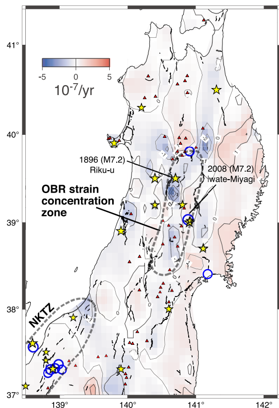
Fig. 1. EW strain rate calculated from the GPS velocity field for the period from 1997 to 2001 (after figure 6(b) in Miura et al. , 2004). The effect of interplate coupling is eliminated from a predicted model (Suwa et al. , 2006). Blue and red areas denote contraction and extension, respectively. The effect of interplate coupling is eliminated. Solid lines represent traces of the inland active fault (Nakata and Imaizumi, 2002). Red triangles indicate Quaternary active volcanoes. Gray dashed lines encircle strain concentration zones of the Ou-backbone Range (OBR) and the northeastern part of the Niigata-Kobe Tectonic Zone (NKTZ). Stars represent the epicenters of damaging earthquakes since 1896. Blue circles represent the epicenters of inland earthquakes (larger than M_w 6) from October 1997 to March 10, 2011.
