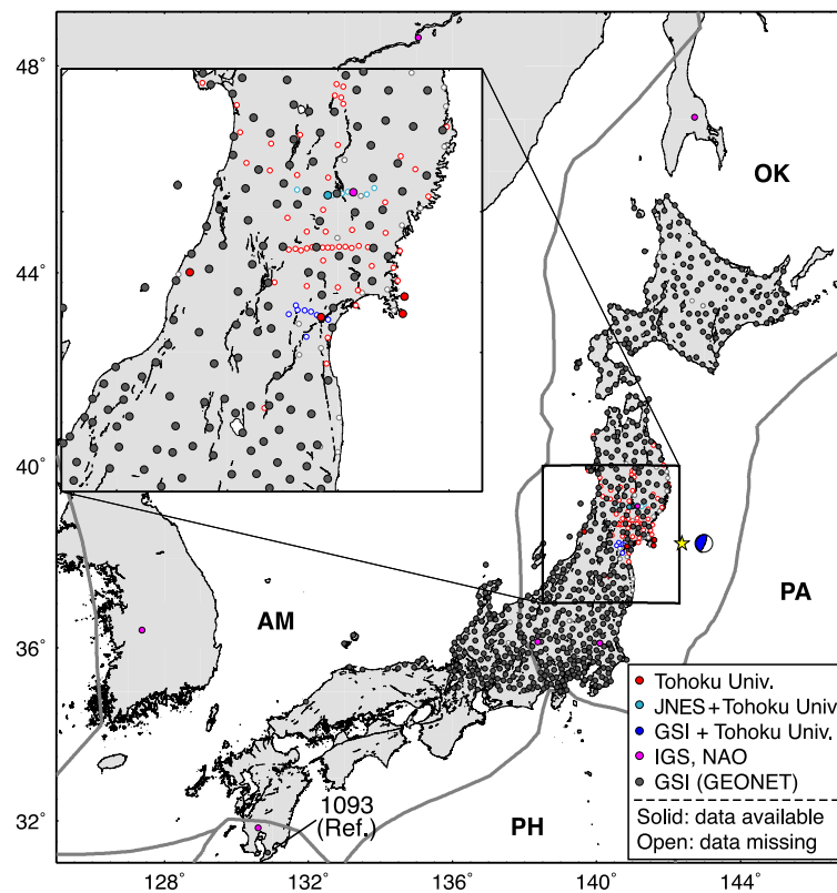
Fig. 3. Distribution of continuous GPS sites. Each symbol denotes an installed institution or laboratory (red: Tohoku University; light blue: collaboration of JNES and Tohoku university; blue: collaboration of GSI and Tohoku university; pink: IGS (MIZU), and NAO; gray: GSI (GEONET)). Coseismic displacements were obtained at the colored sites at the sites indicated by solid circles.
