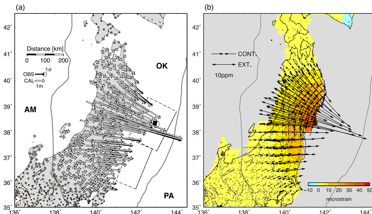
Fig. 4. (a) Horizontal displacement induced by the 2011 Tohoku earthquake. The reference site is a GEONET site, 1093. Black and white arrows represent observed and calculated horizontal displacement vectors from the simple fault model, respectively. The two rectangles with a solid line indicating an upper fault edge represent the surface projection of the estimated fault model. The focal mechanism solution of the mainshock provided by a W-phase analysis ( http://earthquake.usgs.gov/earthquakes/eqinthenews/2011/usc0001xgp/neic_c0001xgp_wmt.php ) is shown at the epicenter. Solid gray lines indicate plate boundaries after Bird (2003). PA, OK, and AM are abbreviations for the Pacific, Okhotsk, and Amurian plates, respectively. (b) Dilatation strain (color, positive value means expansion) and principal strain axis (vectors) calculated from coseismic displacement.
