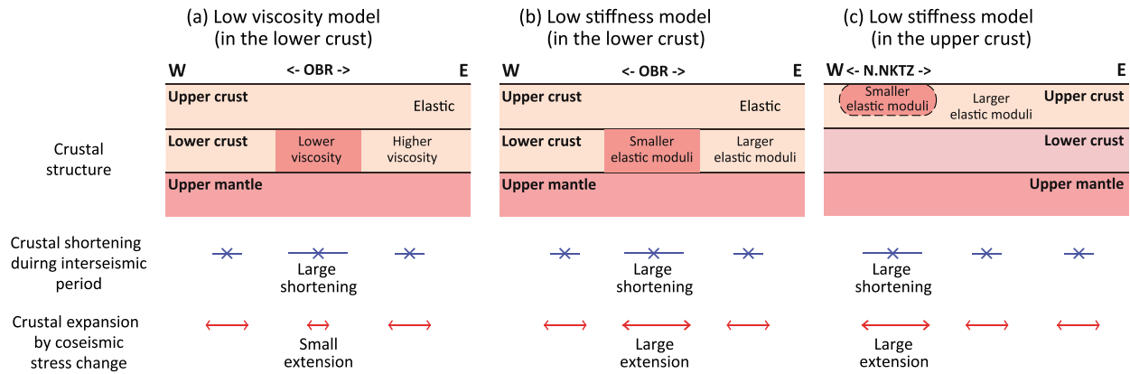
Fig. 2. Schematic images of surface strain, which depends on the crustal structure, around the two strain concentration zones, the OBR and the northern part of the NKTZ in the Tohoku region. The assumed crustal structure and their surface strain pattern during the interseismic period and the coseismic period are shown. (a) Low viscosity model in the lower crust. The viscosity in the lower crust beneath the OBR is assumed to be lower than in the other fields. (b) Low elastic modulus model in the lower crust. The elastic modulus in the lower crust beneath the OBR is assumed to be lower than in the other fields. (c) Low elastic modulus model in the upper crust. The elastic modulus in the upper crust beneath the NKTZ is assumed to be lower than in the other fields due to the existence of thick sediments.
