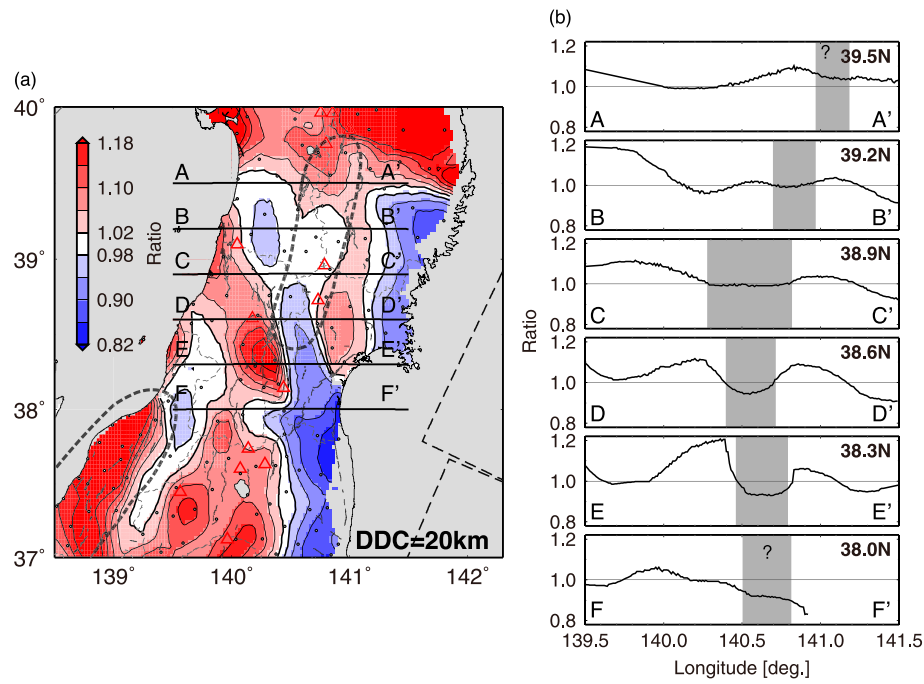
Fig. 6. SC-ratio profiles. (a) Same as Fig. 5(b). Six lines crossing east to west are the profile line of (b). (b) SC-ratio profile between 139.5°E and 141.5°E crossing 39.5°N (A–A'), 39.2°N (B–B'), 38.9°N (C–C'), 38.6°N (D–D'), 38.3°N (E–E'), and 38.0°N (F–F'). Shadow areas correspond to the OBR strain concentration zone.
