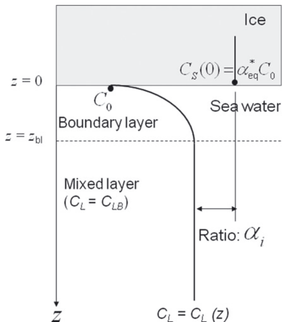
Fig. 5. Schematic of the stagnant boundary-layer (SBL) model. z=0 is set at the bottom of the sea ice and z_{bl} is assumed to be constant. The effective fractionation coefficient of ice ( \epsilon_{\text{eff}, i} ) is calculated from \epsilon_{\text{eff}, i} = (\alpha_i - 1) \cdot 1000 (‰).
