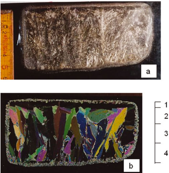
Fig. 2. One example of the textural structure of sea ice grown at a room temperature of -15^{\circ}\text{C} . (a) Thick section ( 5\text{ mm} thick); (b) thin section ( 1\text{ mm} thick). 1. Vertical c -axis layer ( 0.0\text{--}0.5\text{ cm} depth); 2. transition layer ( 0.5\text{--}2.0\text{ cm} ); 3. inner columnar layer ( 2.0\text{--}3.5\text{ cm} ); 4. bottom columnar layer ( 3.5\text{--}5.0\text{ cm} ).
