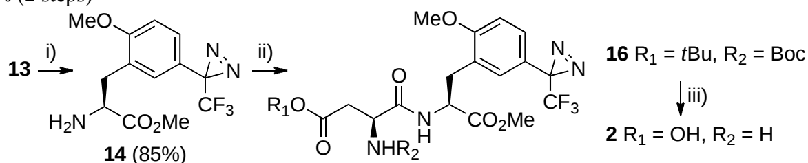
Scheme 3. Synthesis of diazirinyl L-phenylalanine derivatives ( 13 ). i) \text{SOCl}_2 , MeOH, rt, 8 h, 85%, ii) N\text{-Boc-L-Asp(OTBu)OSu} ( 15 ), (i\text{-Pr})_2\text{NEt} , THF, rt, 8 h, 86%, iii) TFA, 0^\circ\text{C} , 3 h, 97%.
