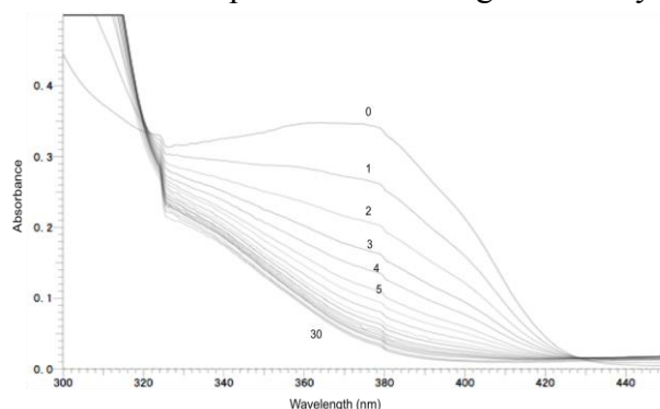
Scheme 4. Photolysis of photoreactive aspartame ( 2 ) in methanol (1 mM) with black light (100W). UV spectra of the photolysis reaction were recorded every 1 min until 15 min, then every 5min until 30 min.
