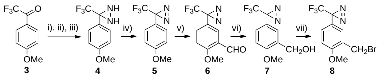
Scheme 1. Synthesis of diazirinyl benzyl bromide derivatives ( 8 ). i) \text{NH}_2\text{OH} \cdot \text{HCl} , pyridine, 80^\circ\text{C} , 3 h, ii) \text{TsCl} , TEA, acetone, 0^\circ\text{C} , 1 h, iii) \text{NH}_3 (l), ether, rt, 8 h, 85% (3 steps), iv) \text{MnO}_2 , ether, rt, 6 h, 93%, v) \text{Cl}_2\text{CHCHO} , \text{TiCl}_4 , 0^\circ\text{C} , 1 h, 98%, vi) \text{NaBH}_4 , EtOH, rt, 4 h, 92%, vii) \text{CBr}_4 , \text{Ph}_3\text{P} , rt, 4 h, 95%
