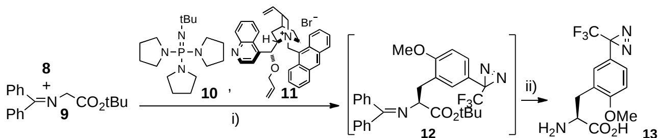
Scheme 2. Synthesis of diazirinyl L-phenylalanine derivative ( 13 ). i) \text{CH}_2\text{Cl}_2 , -78^\circ\text{C} , 8 h, ii) TFA, 0^\circ\text{C} , 2 h, 65% (2 steps)
