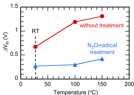
FIG. 12. Negative-gate-bias-induced V_{th} shifts of the MOS-HEMTs without and with the N 2 O-radical treatment measured at RT, 100 °C, and 150 °C.
