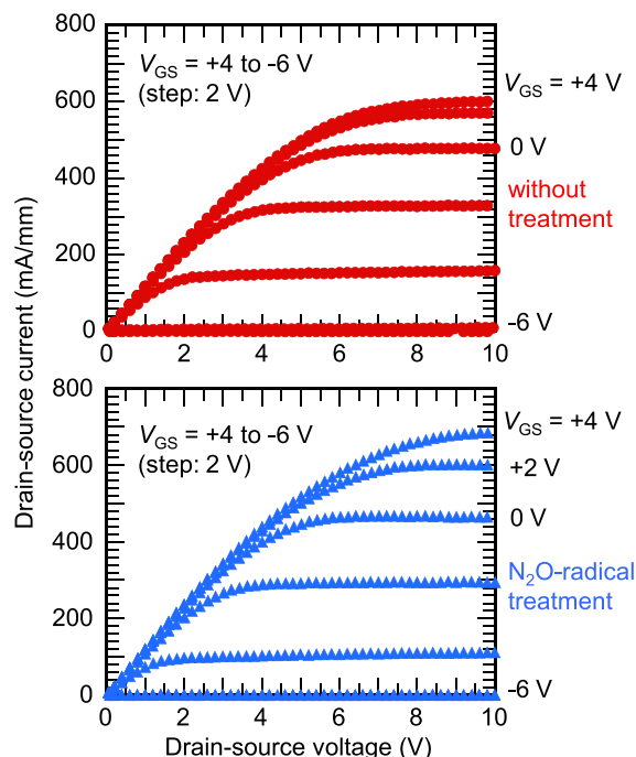
FIG. 9. I_{\text{DS}}\text{-}V_{\text{DS}} characteristics of the \text{Al}_2\text{O}_3/\text{AlGaN}/\text{GaN} MOS-HEMTs without and with the \text{N}_2\text{O} -radical treatment pulsed from “no-stress” bias condition.
