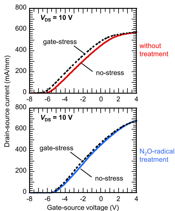
FIG. 10. Transfer characteristics of the \text{Al}_2\text{O}_3/\text{AlGaN}/\text{GaN} MOS-HEMTs without and with the \text{N}_2\text{O} -radical treatment pulsed from “no-stress” (solid lines) and “gate-stress” (broken lines) bias conditions.
