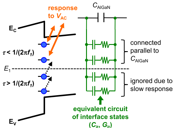
FIG. 5. Equivalent circuit of the interface states in \text{Al}_2\text{O}_3/\text{AlGaIn}/\text{GaIn} structures during the C - V measurement.
