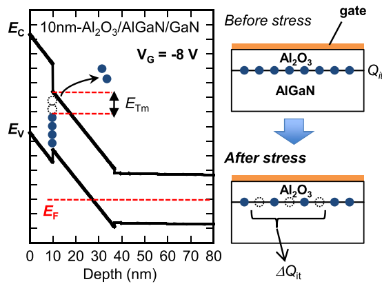
FIG. 11. Calculated potential profile of the Al 2 O 3 /AlGaIn/GaN at V_{GS} = -8 V and schematic illustration of the possible mechanism for the negative-gate-bias-induced V_{th} shifts.
