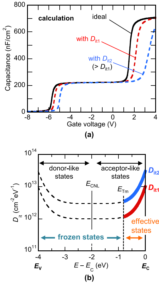
FIG. 3. (a) Calculated C - V characteristics of the \text{Al}_2\text{O}_3/\text{AlGaIn}/\text{GaN} structures. (b) \text{Al}_2\text{O}_3/\text{AlGaIn} interface density distributions assumed in the calculation.
