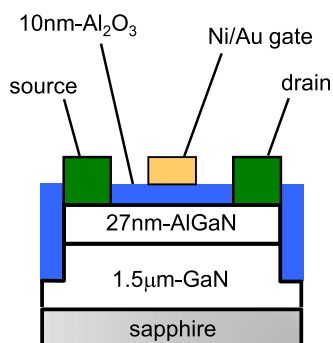
FIG. 1. Schematic cross-sectional view of the \text{Al}_2\text{O}_3/\text{AlGaIn}/\text{GaIn} MOS-HEMT structure.
