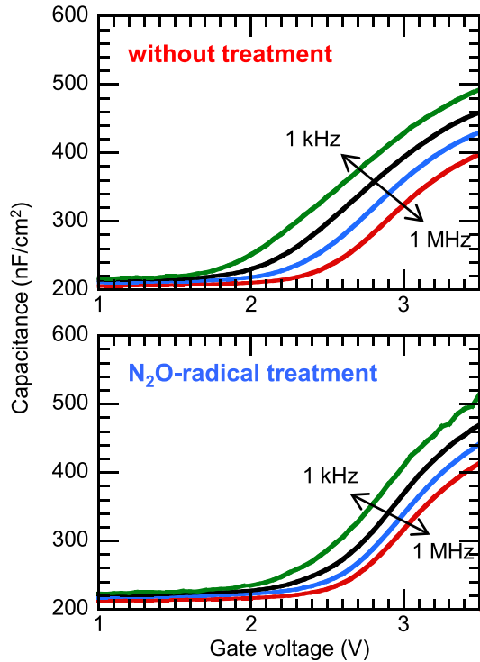
FIG. 4. Frequency dispersion of the C - V characteristics of the \text{Al}_2\text{O}_3/\text{AlGaIn}/\text{GaIn} MOS diode structures without and with the \text{N}_2\text{O} -radical treatment in the positive bias range.
