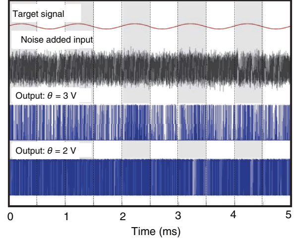
FIG. 6. (Color online) Measured input and output wave forms of the threshold device when the threshold was optimized ( \theta = 3 V) and not optimized ( \theta = 2 V). Gray hatched regions indicate the periods in which the target signal had a positive amplitude. When \theta = 3 V, the pulse density was high in the gray region, indicating that the information in the target signal reflects the output.
