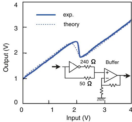
FIG. 2. (Color online) Theoretical and experimental transfer curves of the optimized nonlinear function for the mixed noise. Inset shows the electronic circuit for implementation of the function.
