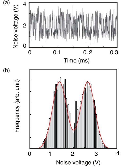
FIG. 1. (Color online) Generated mixed noise: (a) wave form and (b) histogram. Solid curve shows the theoretical probability density function.
