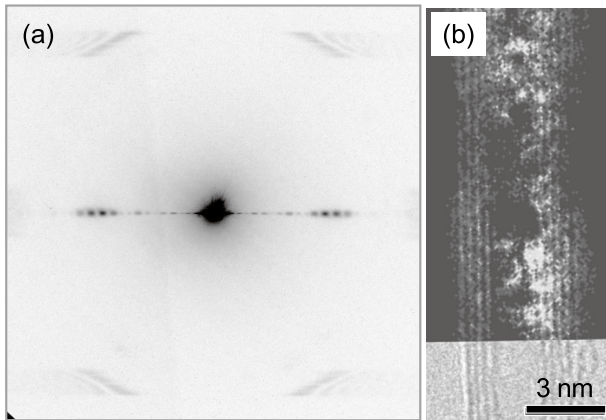
図3 多層カーボンナノチューブの回折パターン（白黒反転：照射エネルギー 20 keV）と再構成像。（Reversed diffraction pattern (a) and reconstructed pattern of MWCNT by prototype microscope (b). TEM image of the SWCNT was inserted in (b).）
