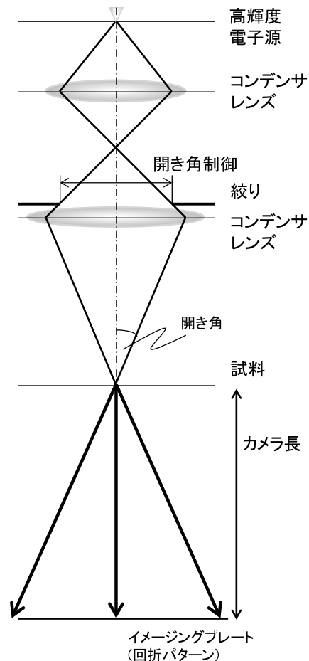
図5 光学系概略図。（Schematic diagram of optics in diffraction recording.）
