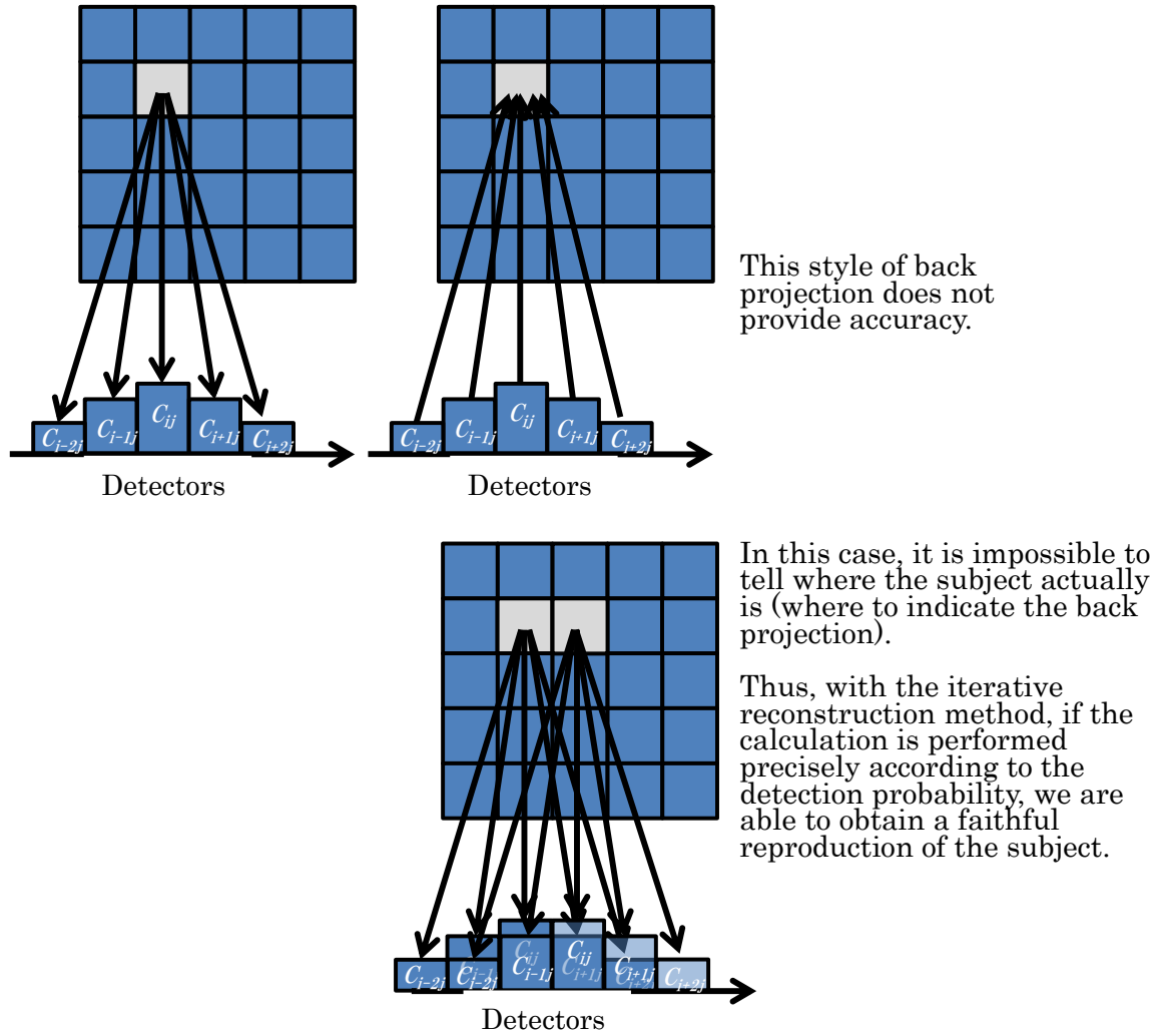
Figure 2 Explanation of why the easily comprehensible method of successive approximation for correcting blur lacks accuracy. Example of two neighboring pixels: Direction of back projection cannot be identified (lower right).
