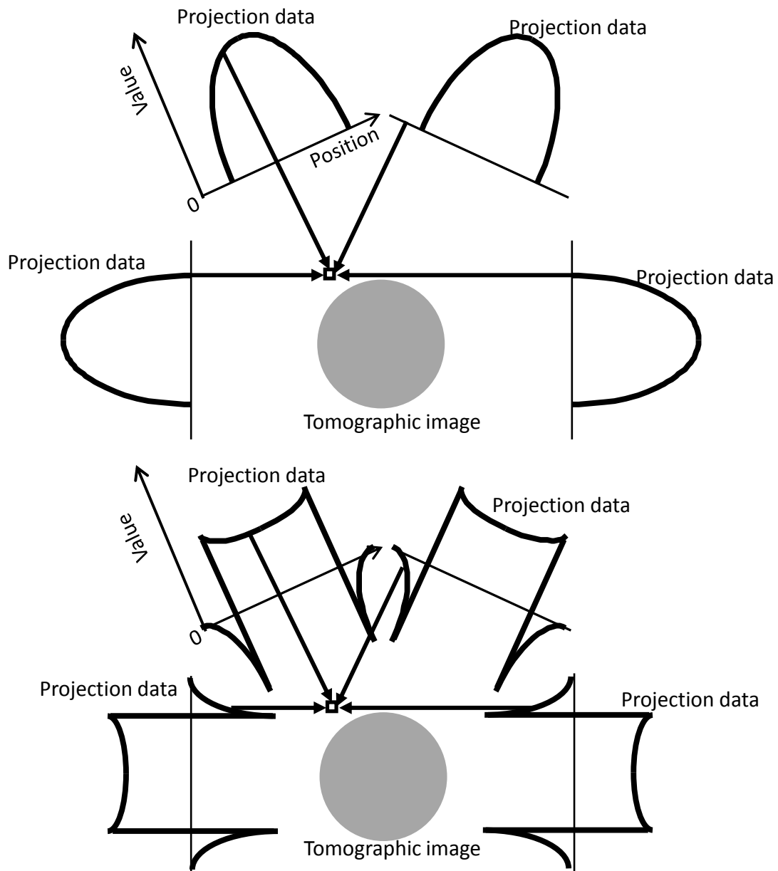
Figure 1 Simple back projection (upper portion), filtered back projection (lower portion)
