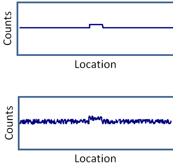
Figure 4 Pattern diagrams illustrating how low-contrast regions can become hard to distinguish due to statistical noise. Examples show a no-noise case (upper) and a case with statistical noise (lower)
