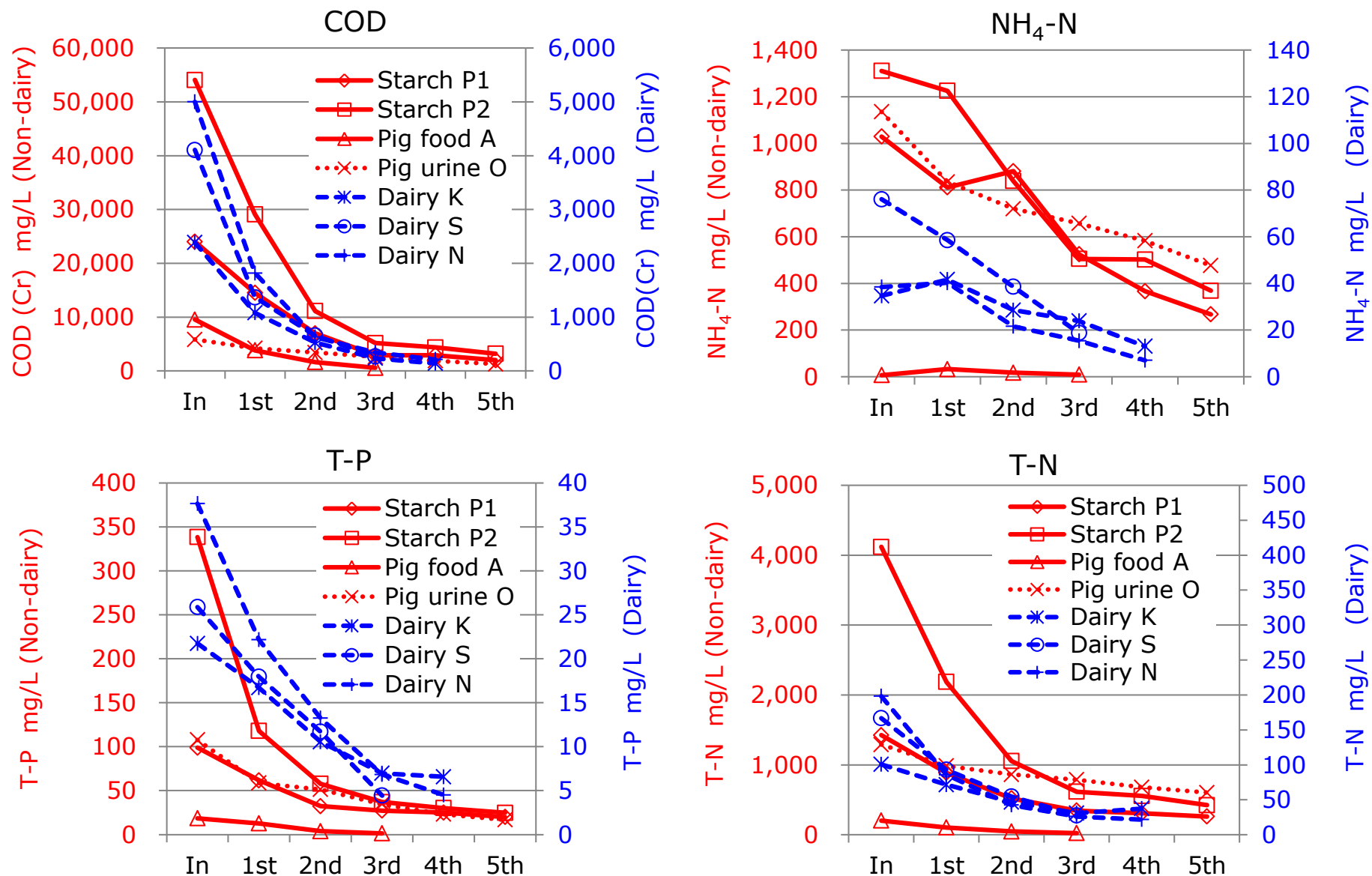
Fig.4 Average pollutant concentrations in the inter-stage data
