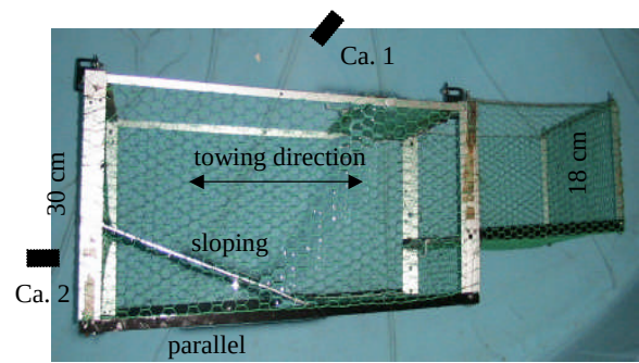
Side view showing the panel or grid orientation, net depth dimensions and the camera positions; Ca. 1 and Ca. 2
