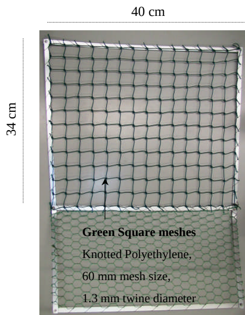
Top view showing net frame dimensions and the square mesh panel in the parallel orientation
