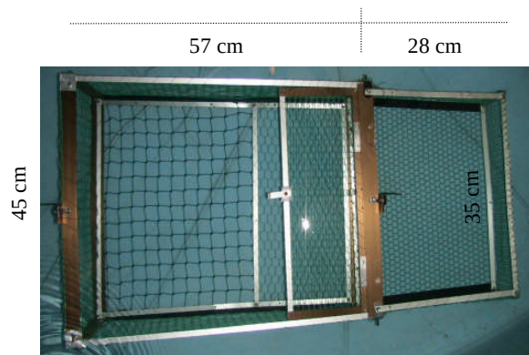
Top view showing net frame dimensions and the square mesh panel in the parallel orientation
