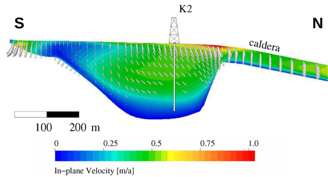
Fig. 2. Velocity field (absolute values as texture and direction vectors) simulated with Elmer/Ice in a north–south transect of the Gorshkov crater glacier through the K2 drillsite.
