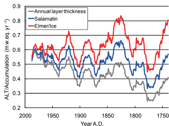
Fig. 6. Reconstructed 20 yr mean accumulation rates and annual layer thickness (ALT) profiles.
