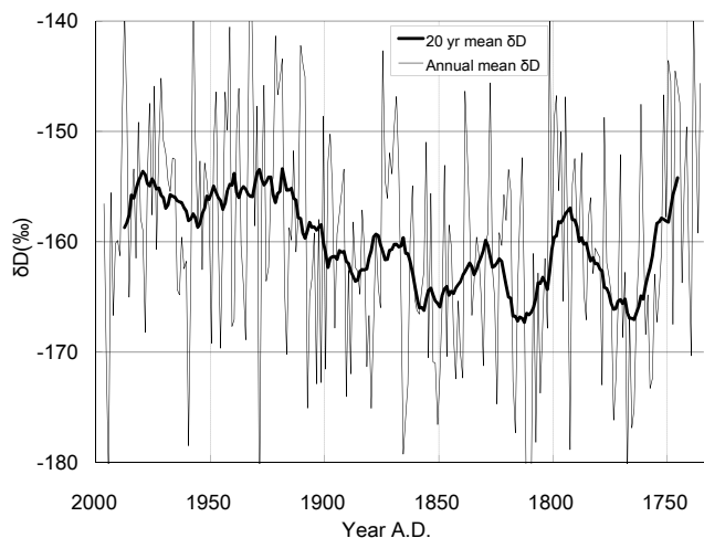
Fig. 4. Annual mean (thin line) and 20 yr mean (thick line) \delta\text{D} profiles. Note that the average isotope ratio increases from the late 19th to the early 20th century.
