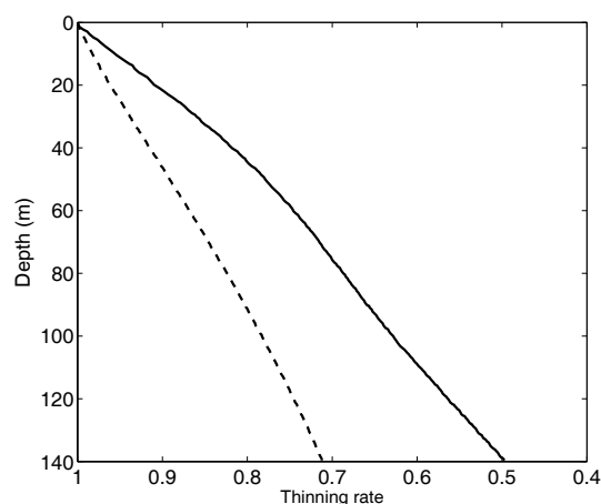
Fig. 5. Thinning rates calculated by the Salamatin (dotted line) and Elmer/Ice (solid line) models.
