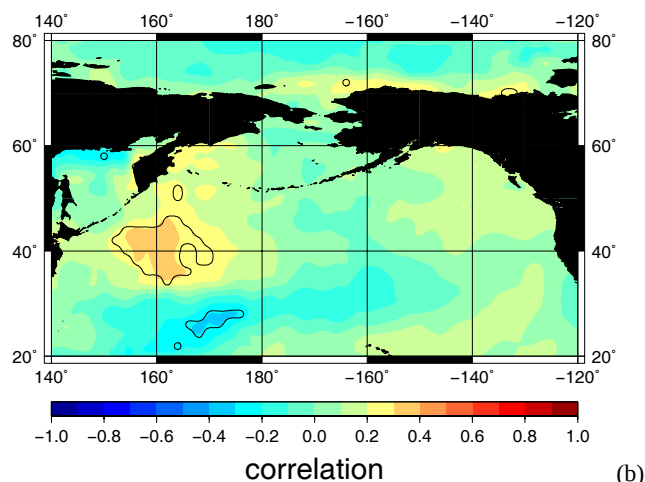
Fig. 10. (a) Correlation map of reconstructed accumulation rates (Elmer/Ice) with ERA-40 3 yr mean surface (2 m) temperature for 1958–1996 (39 yr). Black contours indicate the land-water margin and the 90 % confidence level. (b) Correlation map of reconstructed accumulation rates (Elmer/Ice) with ERSST 3 yr mean sea surface temperature for 1854–1995 (142 yr). Black contours indicate the land-water margin and the 90 % confidence level.
