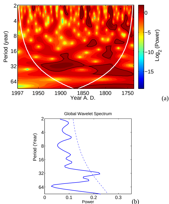
Fig. 8. a) Wavelet plot for reconstructed accumulation rates (Elmer/Ice): binary logarithm of the power (absolute square of the wavelet transform) in m^2 a^{-2} . Black contours represent the 95 % confidence level against red noise (Torrence and Compo, 1998). Areas outside the cone of influence (indicated by the thick white line) are to be discarded. (b) Global wavelet spectrum for reconstructed accumulation rates (Elmer/Ice). The thin dashed line indicates the the 95 % confidence level against red noise.
