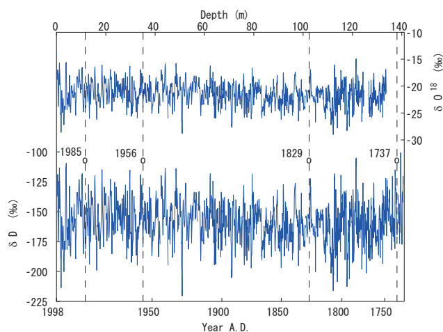
Fig. 3. Measured water isotope profiles with dating results. Upper line: \delta^{18}\text{O} , lower line: \delta\text{D} . Dotted lines with year number indicate dated volcanic ash layers (Murav'yev et al., 2007).
