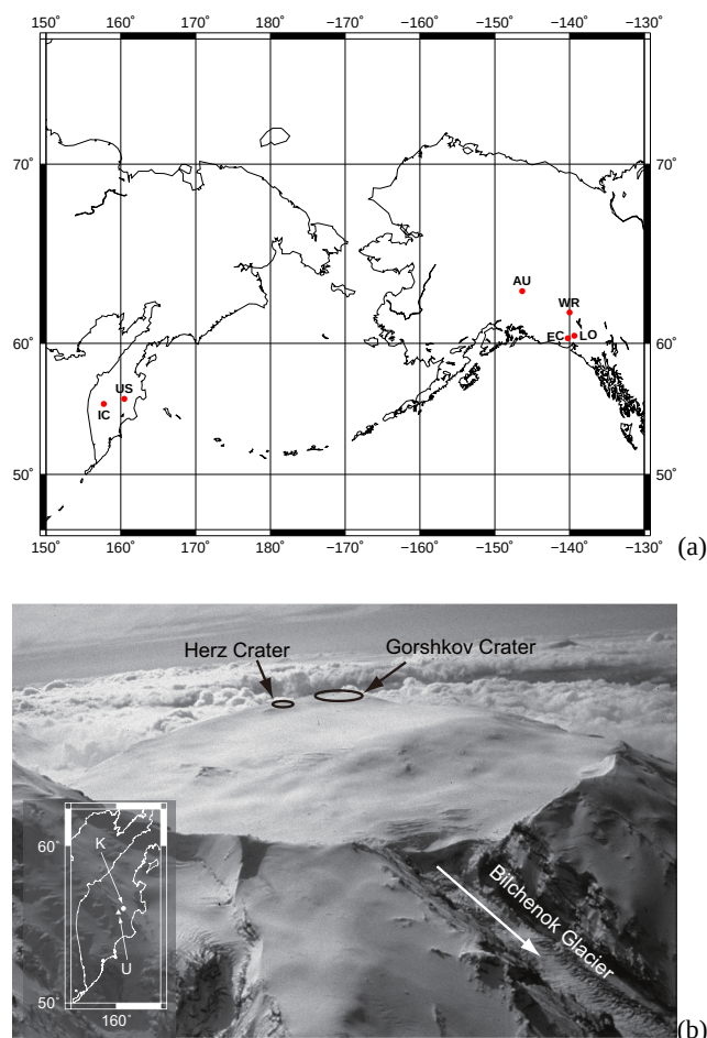
Fig. 1. (a) Deep ice core sites around the subpolar Pacific. US: Ushkovsky (Shiraiwa et al., 2001), IC: Ichinsky (Matoba et al., 2011), LO: Logan (Holdsworth et al., 1989; Shiraiwa et al., 2003; Fisher et al., 2004), EC: Logan Eclipse (Wake et al., 2002), WR: Wrangell (Yasunari et al., 2007), AU: Aurora Peak (Fukuda et al., 2011). (b) The north face of Ushkovsky volcano and the summit craters. Bilchenok Glacier is the main outlet from the summit ice cap. Inset the location of Ushkovsky volcano (U) and the nearby weather station, Kljuchi (K).
