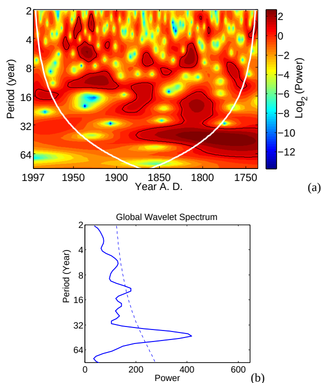
Fig. 7. (a) Wavelet plot for \delta D : binary logarithm of the power (absolute square of the wavelet transform) in \%^2 . Black contours represent the 95 % confidence level against red noise (Torrence and Compo, 1998). Areas outside the cone of influence (indicated by the thick white line) are to be discarded. (b) Global wavelet spectrum for \delta D . The thin dashed line indicates the 95 % confidence level against red noise.
