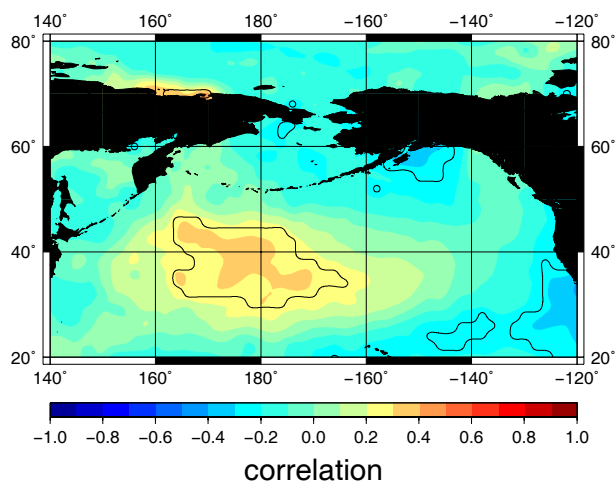
Fig. 9. (a) Correlation map of the ice core \delta D with ERA-40 3 yr mean surface (2 m) temperature for 1958–1996 (39 yr). Black contours indicate the land-water margin and the 90 % confidence level. (b) Correlation map of the ice core \delta D with ERSST 3 yr mean sea surface temperature for 1854–1995 (142 yr). Black contours indicate the land-water margin and the 90 % confidence level.
