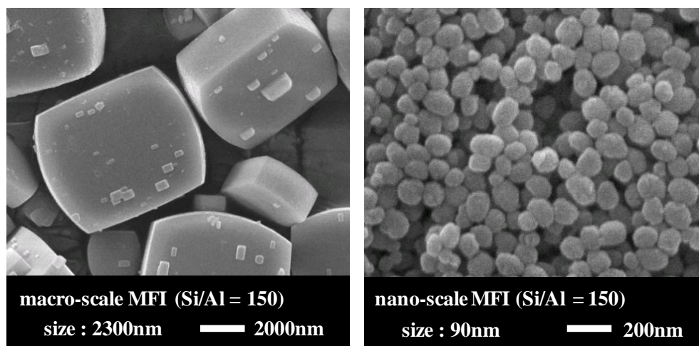
Fig. 3.3 SEM micrographs of macro- and nano-scale zeolites
