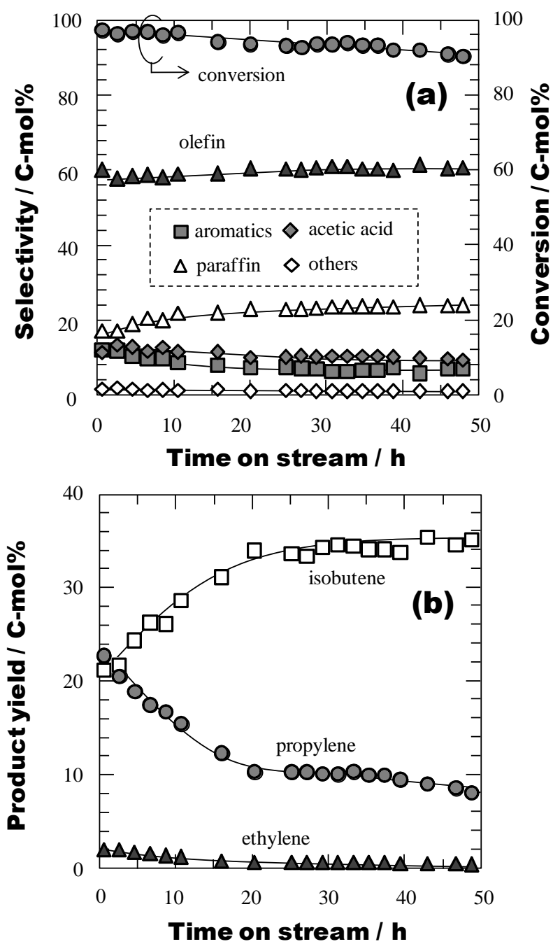
Fig. 5.14 Changes in (a)acetone conversion, product selectivities and (b) light olefins yield with time over PS-treated nano-scale MFI-type zeolite (Reaction conditions: T = 723\text{K} , W/F = 0.5\text{h} )
