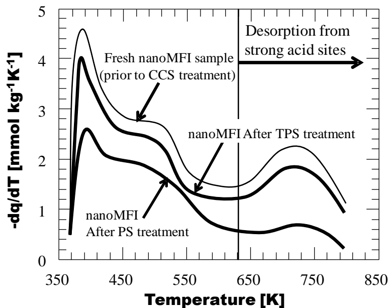
Fig. 5.10 \text{NH}_3 -TPD profiles of nano-MFI before/after CCS treatment.
