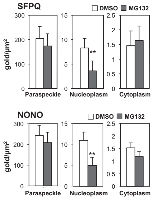
FIGURE 4: MG132 affects SFQ and NONO nuclear distribution, resulting in depleted nucleoplasmic levels of the proteins. SFQ or NONO density was determined by I-EM as gold particles/μm 2 within paraspeckles, the surrounding nucleoplasm, and the cytoplasm of DMSO- and MG132-treated (5 μM, 17 h) HeLa cells. Although the proteins occur at different density values in the three locations (note the different values on the y axes), only the nucleoplasmic pool of SFQ and NONO was specifically depleted with MG132, in parallel with paraspeckle enlargement under this condition. Densities were calculated on 120 and 140 μm 2 of cytoplasm, 93 and 92 μm 2 of nucleoplasm, and 33 and 51 paraspeckles in DMSO and MG132 cells, respectively, for SFQ. Corresponding values for NONO are 76 and 75, 108 and 92, and 25 and 45.
