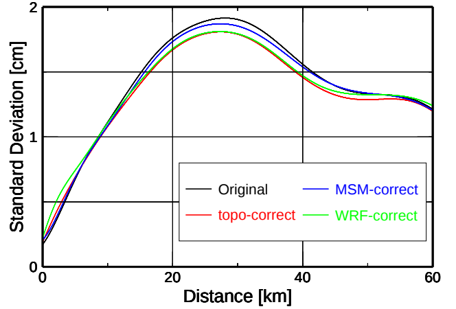
Fig. 5 Variograms of four original and corrected interferograms for all (54) data pairs.
