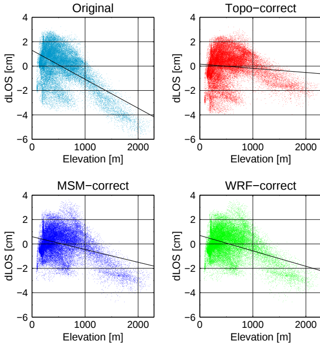
Fig. 6 Variation of the phase with elevation of the surface and the approximated line (black line) in D2 (see Table S1). (Upper left) Scatter plot of the original interferogram. (Upper right) That of the DEM-based corrected interferogram. (Bottom left) That of the MSM-based corrected interferogram. (Bottom right) That of the WRF-based corrected interferogram.
