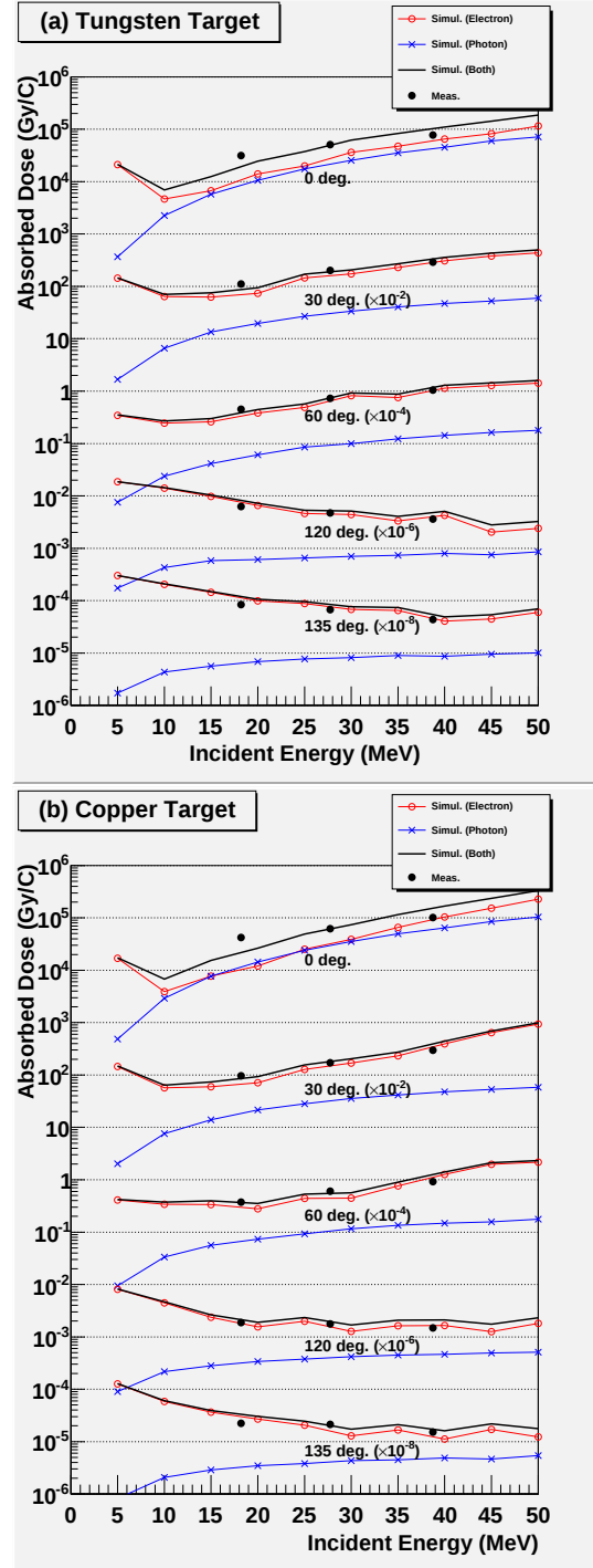
Figure 18. Measured and simulated absorbed-dose distributions at 0 to 135 degrees as a function of incident electron energy bombarding (a) tungsten and (b) copper targets. The others are the same as in Fig. 17.
