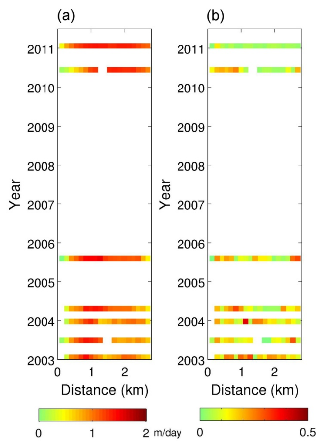
Figure S6: (a) Temporal evolution of the velocity profile A-B in Figure S5. (b) Estimated errors of the velocity profile at each epoch.
