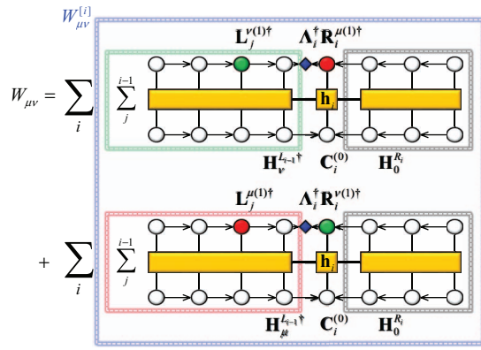
FIG. 5. Graphical representation for computation of W_{\mu\nu}^{[i]} .
