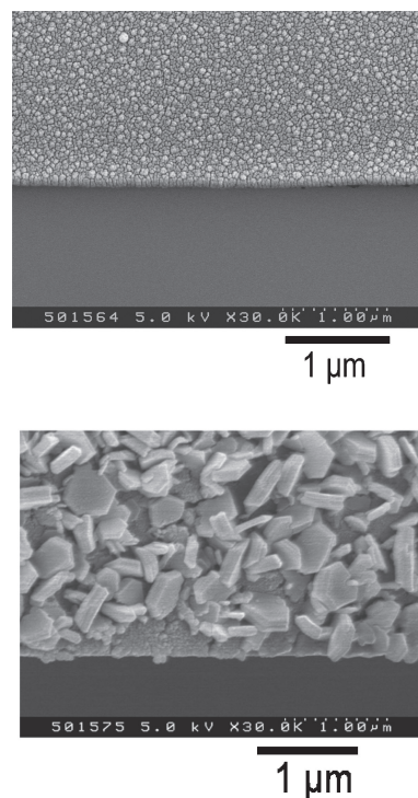
Fig. 5. FE-SEM image of the surface of the \text{Al}_2\text{O}_3 -ZnO films, heat-treated at 400^\circ\text{C} and immersed in hot water for 15 min.
