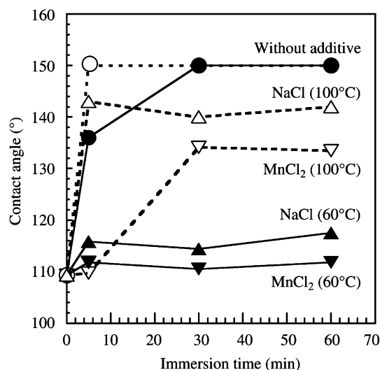
Fig. 4. Immersion-time dependence of the contact angle for water on FAS-coated alumina gel films immersed in hot water with 0.2 M NaCl and \text{MnCl}_2 .
