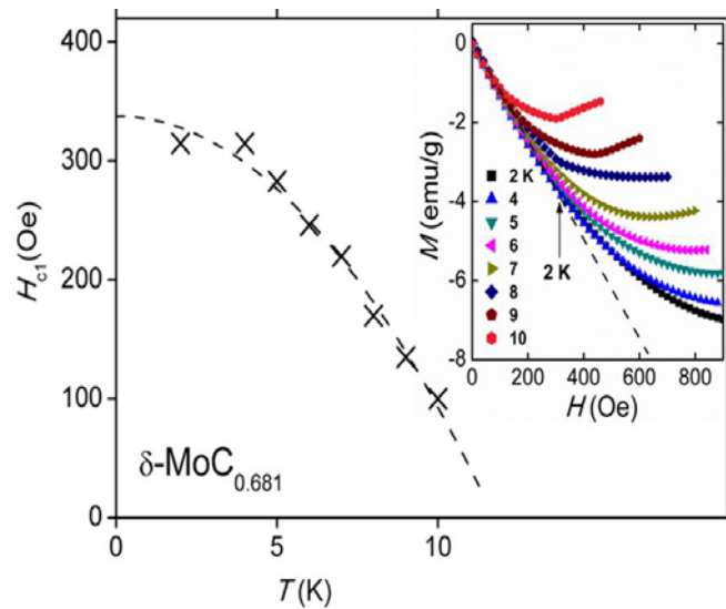
Fig.3.1.12. T dependence of H_{c1} for \delta\text{-MoC}_{0.681} determined by magnetization measurements as shown in the inset. The broken curve best fits the data by a function (see the text).
