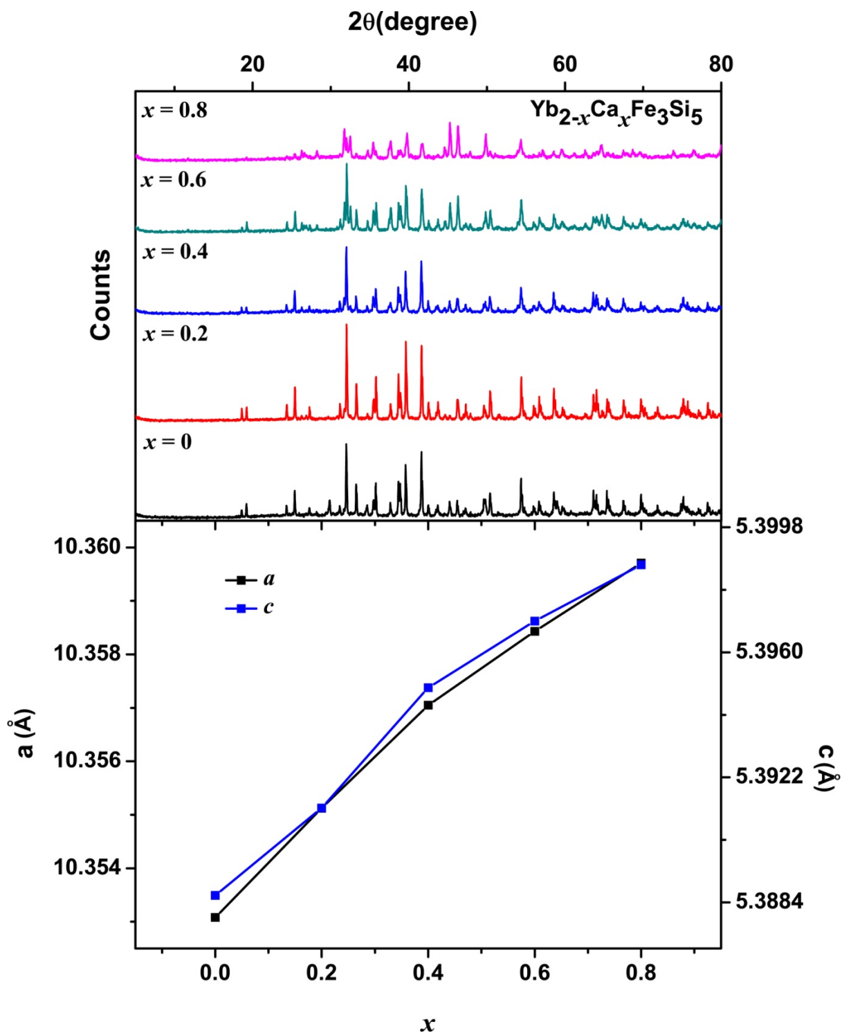
Fig.5.1. (a) Powder XRD patterns of \text{Yb}_{2-x}\text{Ca}_x\text{Fe}_3\text{Si}_5 ( x = 0\text{--}0.8 ). (b) Lattice parameters vs. nominal Ca- concentration.
