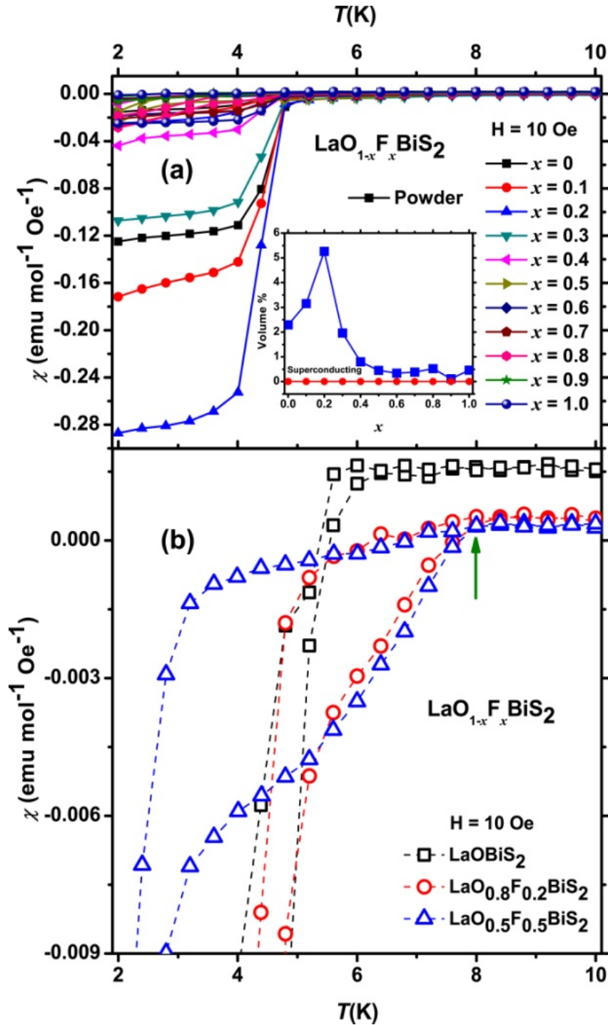
Fig.4.2.4 (a) T dependence of \chi for \text{LaO}_{1-x}\text{F}_x\text{BiS}_2 samples. The set of curves for each compound includes the ZFC and FC curves measured under a magnetic field of 10 Oe. Inset of (a) shows the superconducting shielding fraction calculated for \text{LaO}_{1-x}\text{F}_x\text{BiS}_2 samples. (b) shows the enlarged view for the selected samples of \text{LaO}_{1-x}\text{F}_x\text{BiS}_2 and arrow indicates the temperature at which it starts to drop.
