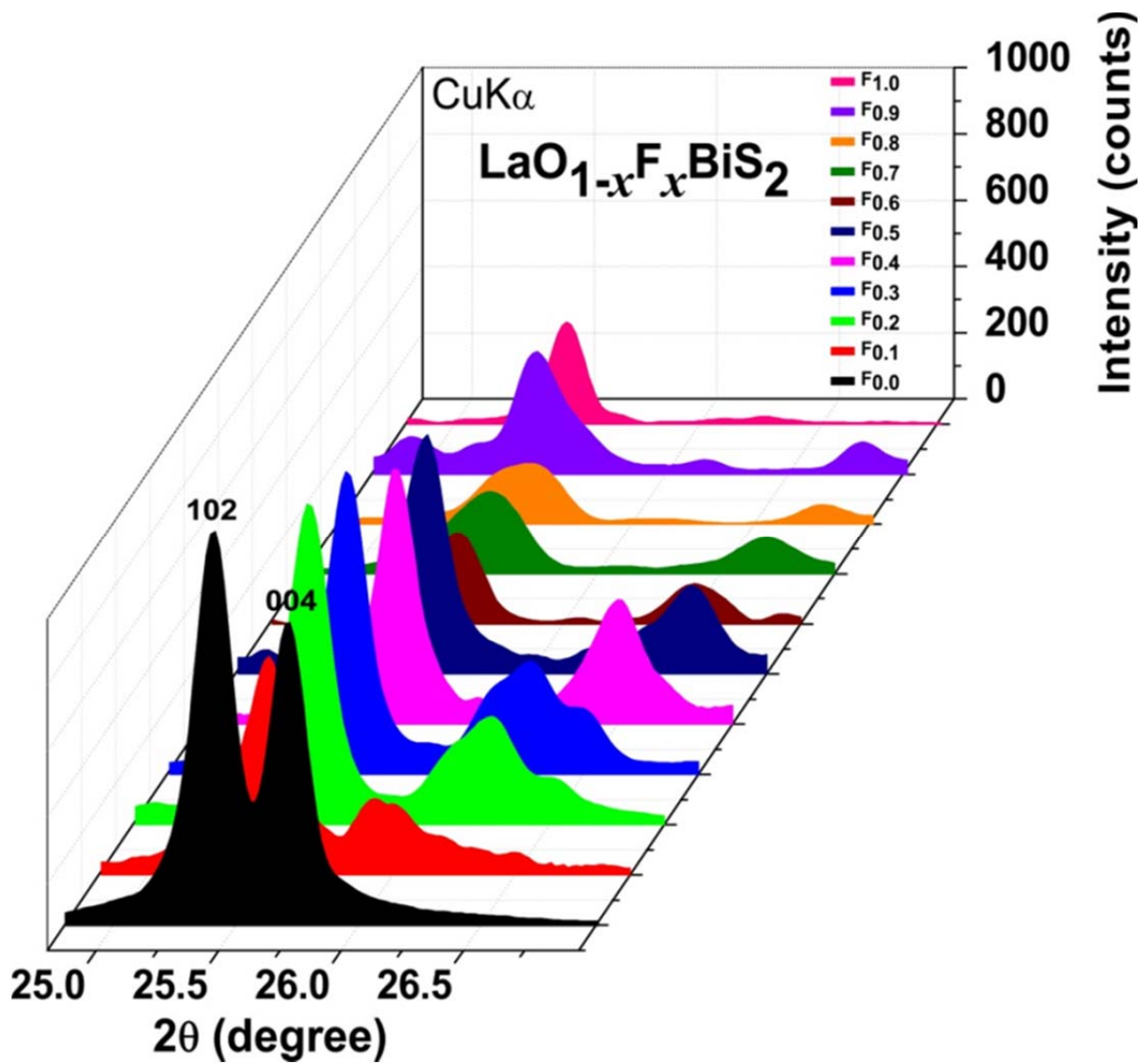
Fig.4.2.2. (c) extrapolation of 102 and 004 peak showing shifting of peaks by substitution of Fluorine.
