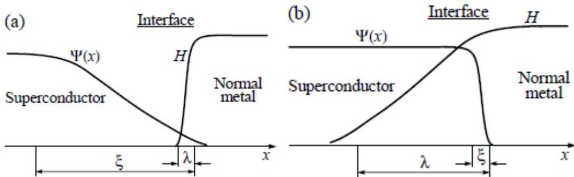
Fig.1.4.3. Order parameter \Psi and magnetic field H in the area of superconductor-normal metal boundary at (a) k \ll 1 and (b) k \gg 1 (extracted from Ref.157).
