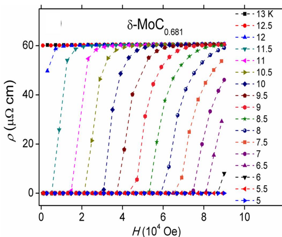
Fig.3.1.10. T variation of the \rho vs. H curves for a polycrystalline dense pellet of \delta\text{-MoC}_{0.681} .
