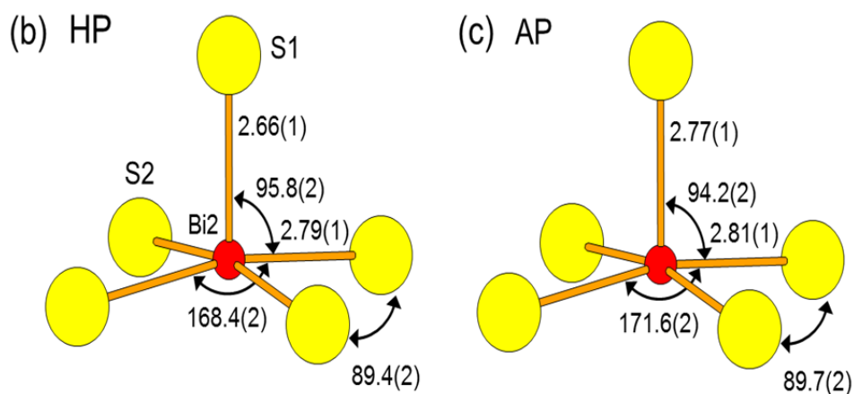
Fig.4.1.2. (b) Local structure coordination of Bi in the BiS 2 layer, drawn based on the present refinement results. The numbers inside are bond distances in Å and angles in degree. (c) Corresponding local structure view for Bi 4 O 4 S 3 synthesized by a normal method for a comparison. The structure data are taken from Ref. [1].
