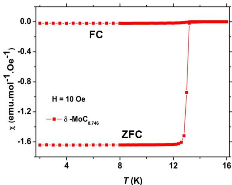
Fig.3.2.2. Temperature dependence of Magnetic susceptibility \delta\text{-MoC}_{0.746} sample measured in a magnetic field of 10 Oe in ZFC and FC mode.
