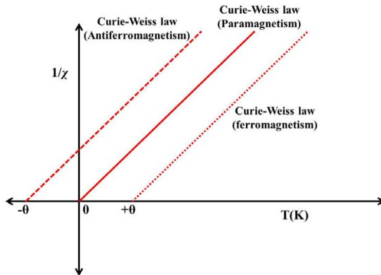
Fig.1.5.4. 1/\chi vs. T of different magnetism (extracted from Ref.163).
