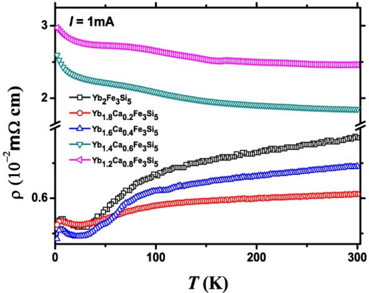
Fig.5.4. T dependence of \rho for \text{Yb}_{2-x}\text{Ca}_x\text{Fe}_3\text{Si}_5 ( x = 0-0.8 ).
