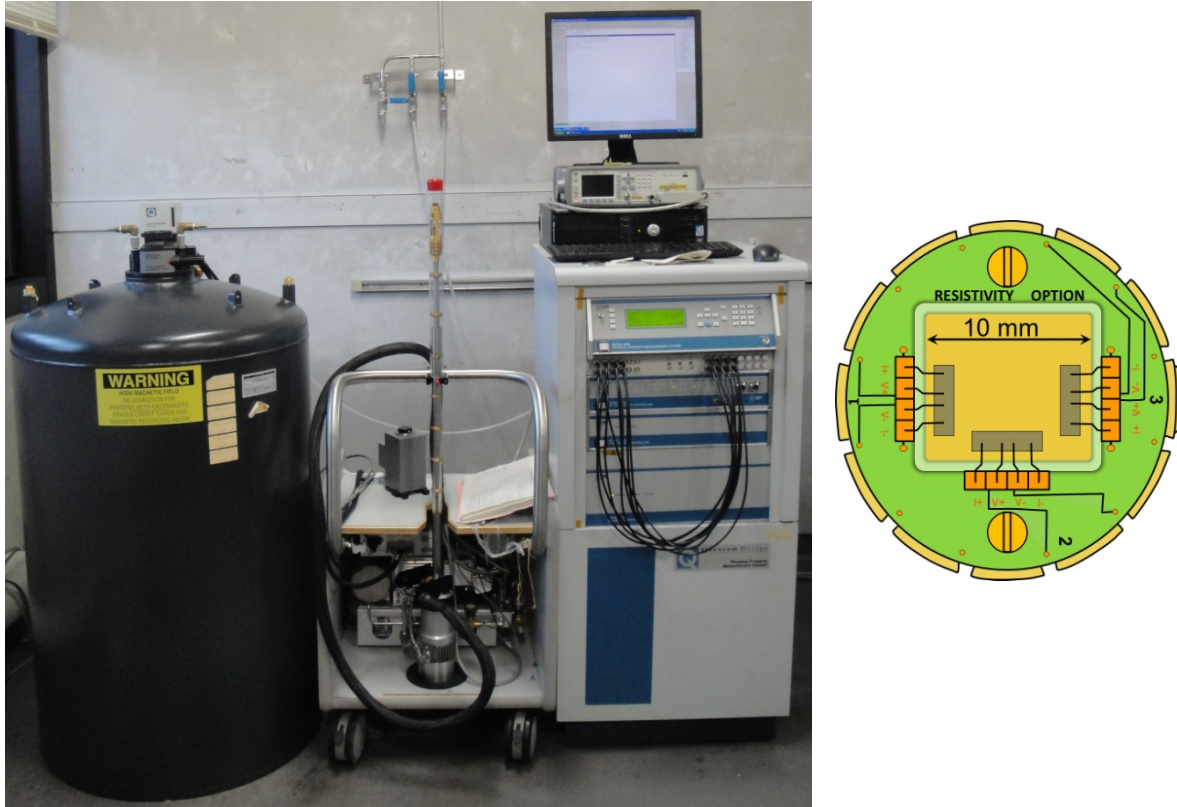
Fig.2.3.2. PPMS 9 tesla from Quantum design and schematic view of designated DC resistivity puck with three samples for concurrent measurements
