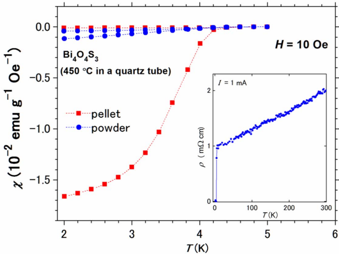
Fig.4.1.3. T dependence of \chi for Bi 4 O 4 S 3 prepared under AP. For comparison, measurements were performed on an as-made pellet and gently ground powder. The largest shielding fraction of approximately 126% was observed for the pellet. Insets show the T dependence of \rho for the as-made pellet of Bi 4 O 4 S 3 (AP).
