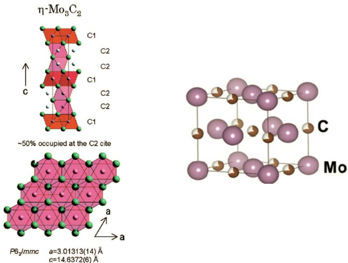
Fig.1.3.2. Pictorial view of \text{Mo}_3\text{C}_2 phase and MoC (extracted from Ref.79 & 80).
