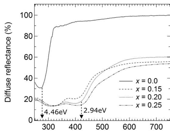
Fig. 3 Diffuse reflectance spectra of \text{Gd}_{1+x}\text{Ca}_{1-x}\text{AlO}_{4-x}\text{N}_x .
