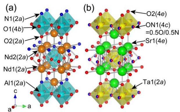
Fig. 1 Crystal structures of K 2 NiF 4 -type oxynitrides: (a) Nd 2 AlO 3 N ( I4mm ) and (b) Sr 2 TaO 3 N ( I4/mmm ).
