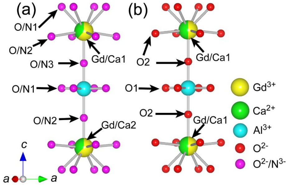
Fig. 5 Atomic arrangement around Al and Gd/Ca sites in (a) \text{Gd}_{1.2}\text{Ca}_{0.8}\text{AlO}_{3.8}\text{N}_{0.2} ( I4mm ) and (b) \text{GdCaAlO}_4 ( I4/mmm ). The schematic structure of \text{GdCaAlO}_4 was drawn using the reported structural parameters [26].
