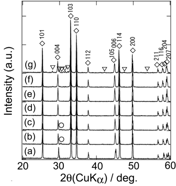
Fig. 2 XRD patterns of products obtained from starting mixtures with AlN only as the aluminum source for \text{Gd}_{1+x}\text{Ca}_{1-x}\text{AlO}_{4-x}\text{N}_x at x = (a) 0, (b) 0.05, (c) 0.1, (d) 0.15, (e) 0.20, (f) 0.25, and (g) 0.30. The product obtained for x = 0 ( \text{GdCaAlO}_4 , (a)) was prepared using \gamma\text{-Al}_2\text{O}_3 as the aluminum source. Diffraction lines marked with diamonds, triangles and circles indicate the \text{K}_2\text{NiF}_4 -type \text{Gd}_{1+x}\text{Ca}_{1-x}\text{AlO}_{4-x}\text{N}_x , \text{Gd}_2\text{O}_3 , and \text{CaAl}_2\text{O}_4 phases, respectively.
