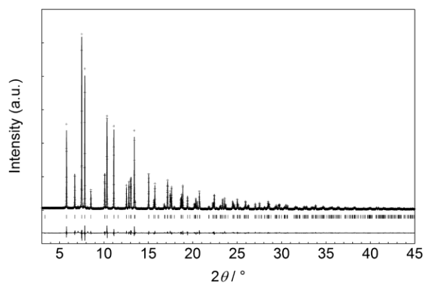
Fig. 4 Observed (+), calculated (solid line) and difference synchrotron XRD profiles for \text{K}_2\text{NiF}_4 -type \text{Gd}_{1.2}\text{Ca}_{0.8}\text{AlO}_{3.8}\text{N}_{0.2} . Vertical bars indicate the positions of Bragg reflections.
