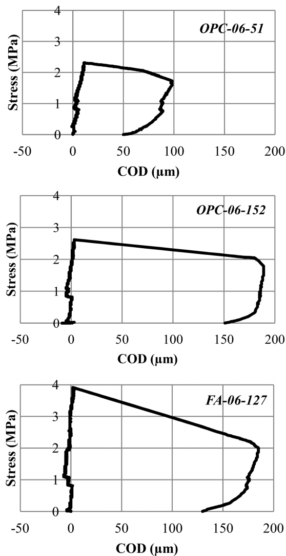
Fig. 2 Tensile stress-COD curves of each specimen.
