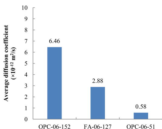
Fig. 15 Comparison of diffusion coefficients perpendicular to the crack wall.
