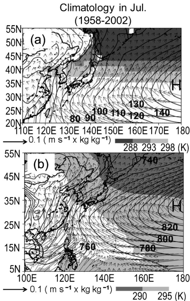
FIG. 8. Spatial distribution of the climatological geopotential height (contour; gpm) and moisture flux ( qV ; \text{m s}^{-1} \text{ kg kg}^{-1} ) at (a) 1000 and (b) 925 hPa in July. Shadings in (a) and (b) represent SST (K) and air temperature at 925 hPa, respectively. A larger domain ( 5^{\circ} – 55^{\circ}\text{N} , 100^{\circ}\text{E} – 180^{\circ} ) is used in (b).
