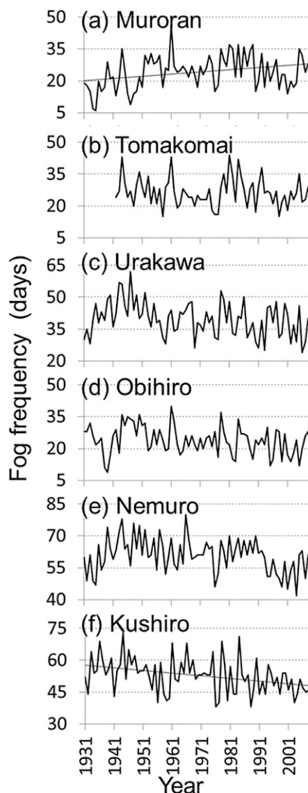
FIG. 3. Interannual variation in summer (JJA) FF (days) at (a) Muroan, (b) Tomakomai, (c) Urakawa, (d) Obihiro, (e) Nemuro, and (f) Kushiro from 1931 to 2010. In (a) and (f) the linear trend on the basis of the 99% confidence level is indicated by thin straight lines.
