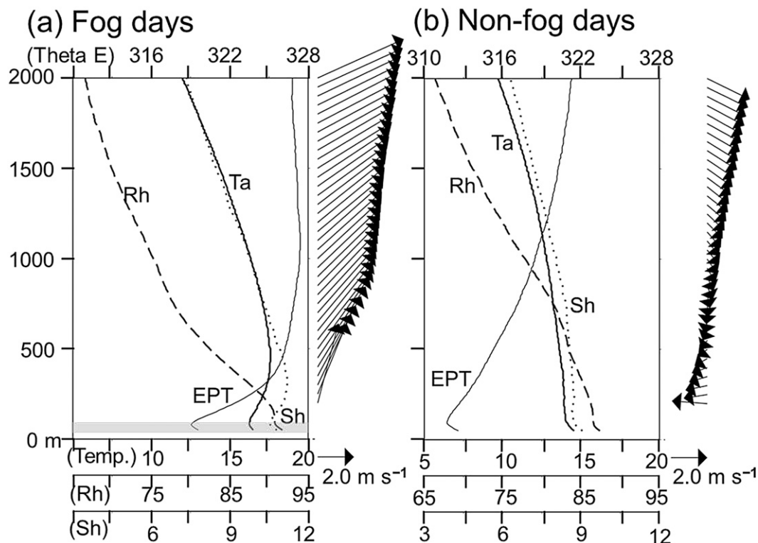
FIG. 7. Composite of vertical profile of temperature [ T_a ( ^{\circ}\text{C} ); thick black line], relative humidity [ R_h (%); dashed line], specific humidity [ Sh ( \text{g kg}^{-1} ); dotted line], equivalent potential temperature [EPT (K); gray thick line], and horizontal wind ( \text{m s}^{-1} ; arrows) at Nemuro for (a) FDs and (b) NFDs. Gray shading in (a) indicates a shallow moist layer.
