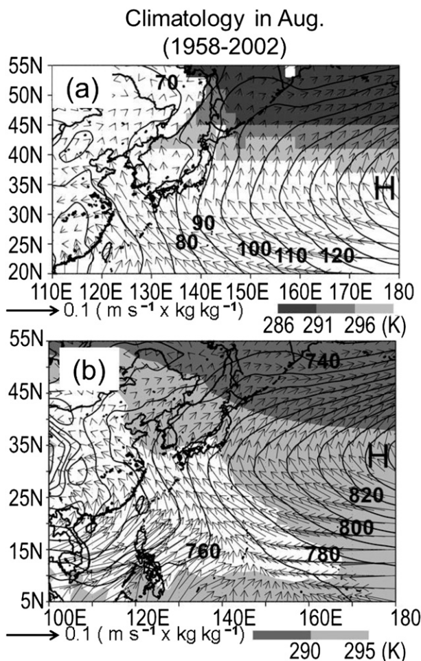
FIG. 10. As in Fig. 8, but for August.
