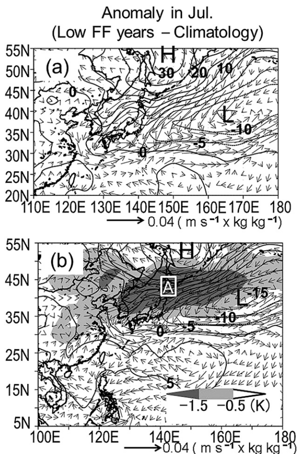
FIG. 9. (a) Low-FF years and climatological differences in geopotential height (gpm) and qV ( \text{m s}^{-1} \text{ kg kg}^{-1} ) at 1000 hPa in July. (b) As in (a), but at 925 hPa; a larger domain ( 5^{\circ} – 55^{\circ} N, 100^{\circ} E– 180^{\circ} ) is used in (b). Light shading and dark shading in (b) indicate temperature anomalies greater than -0.5 and -1.5 K, respectively. The open square in (b) shows domain A, as described in section 5.
