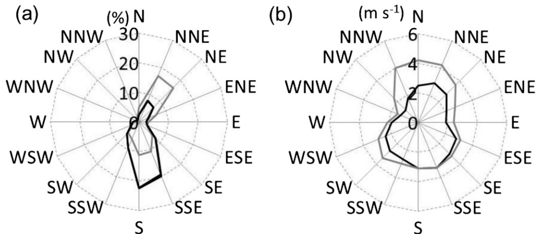
FIG. 6. (a) Frequency of wind direction and (b) mean wind speed for each wind direction at Kushiro for FDs (black curve) and NFDs (gray curve).
