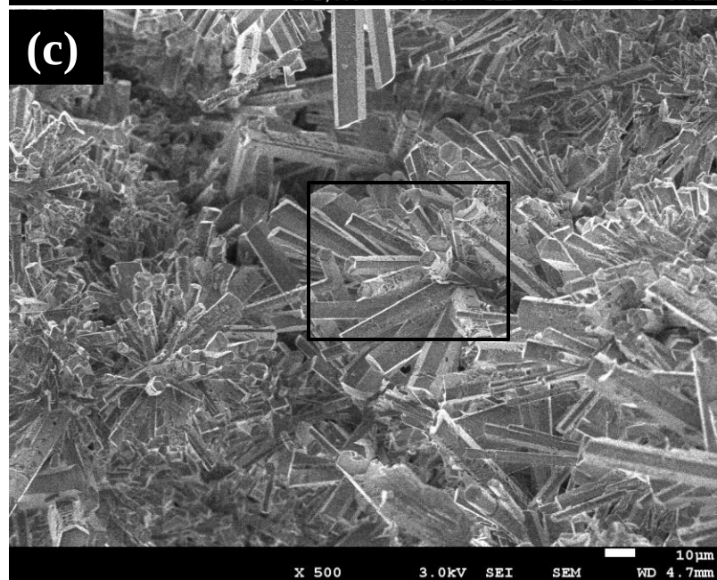
Fig. 6 SEM images of combustion-synthesized \beta -SiAlON powders obtained with 12 mass% (a) KCl, (b) \text{MgCl}_2 , and (c) \text{CaCl}_2 . (d) Enlarged image of the area enclosed in a square in (c).
