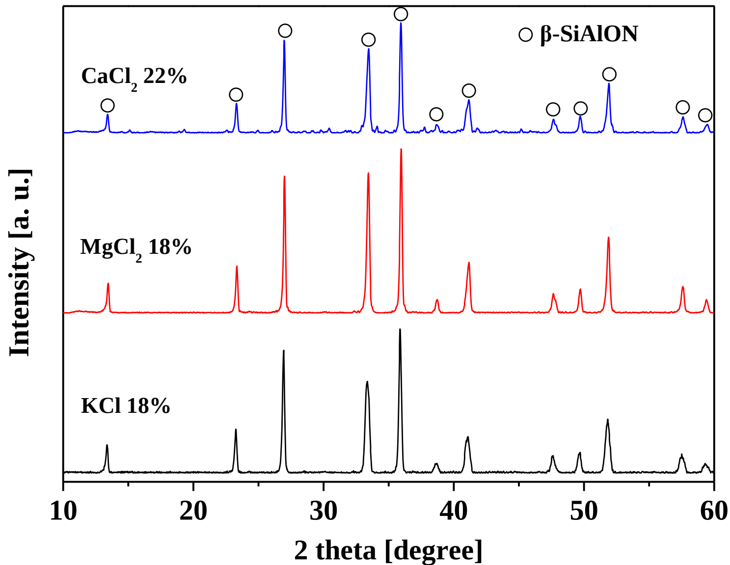
Fig. 2 XRD patterns of combustion-synthesized \beta -SiAlON ( z = 1 ) obtained with optimized amounts of KCl, MgCl 2 , and CaCl 2 (mass%).
