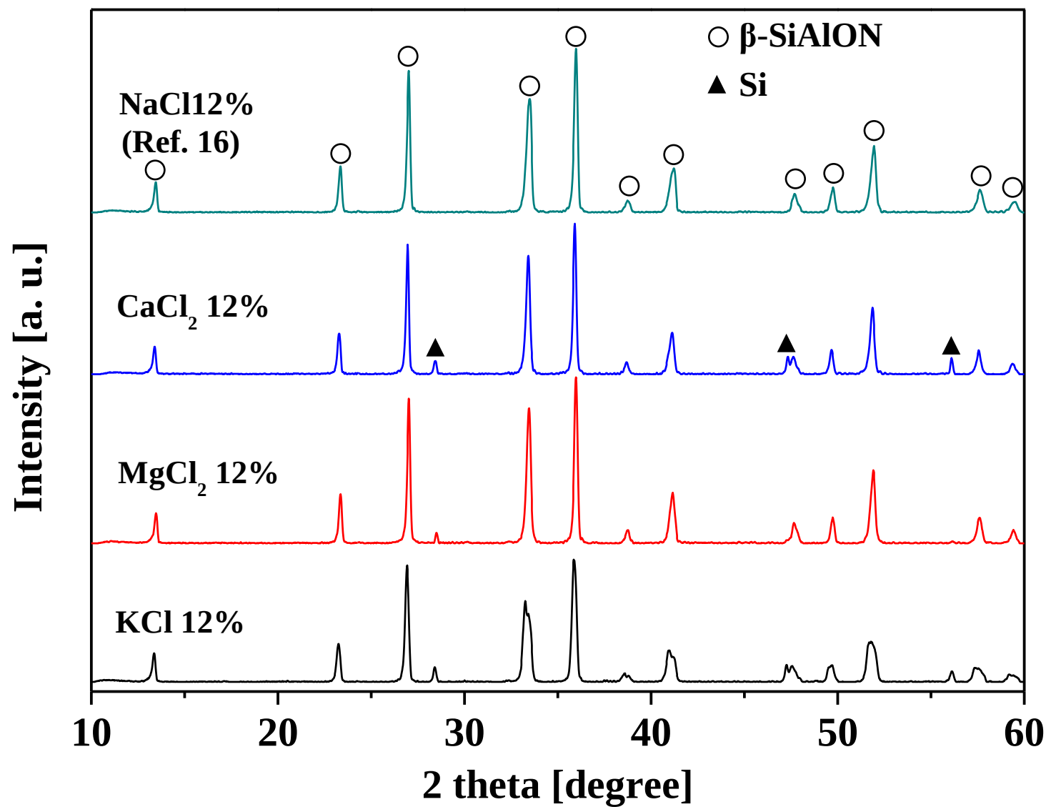
Fig. 1 XRD patterns of combustion-synthesized \beta -SiAlON ( z = 1 ) obtained with the addition of 12 mass% KCl, \text{MgCl}_2 , or \text{CaCl}_2 (this work), or the addition of 12 mass% NaCl (previous work).
