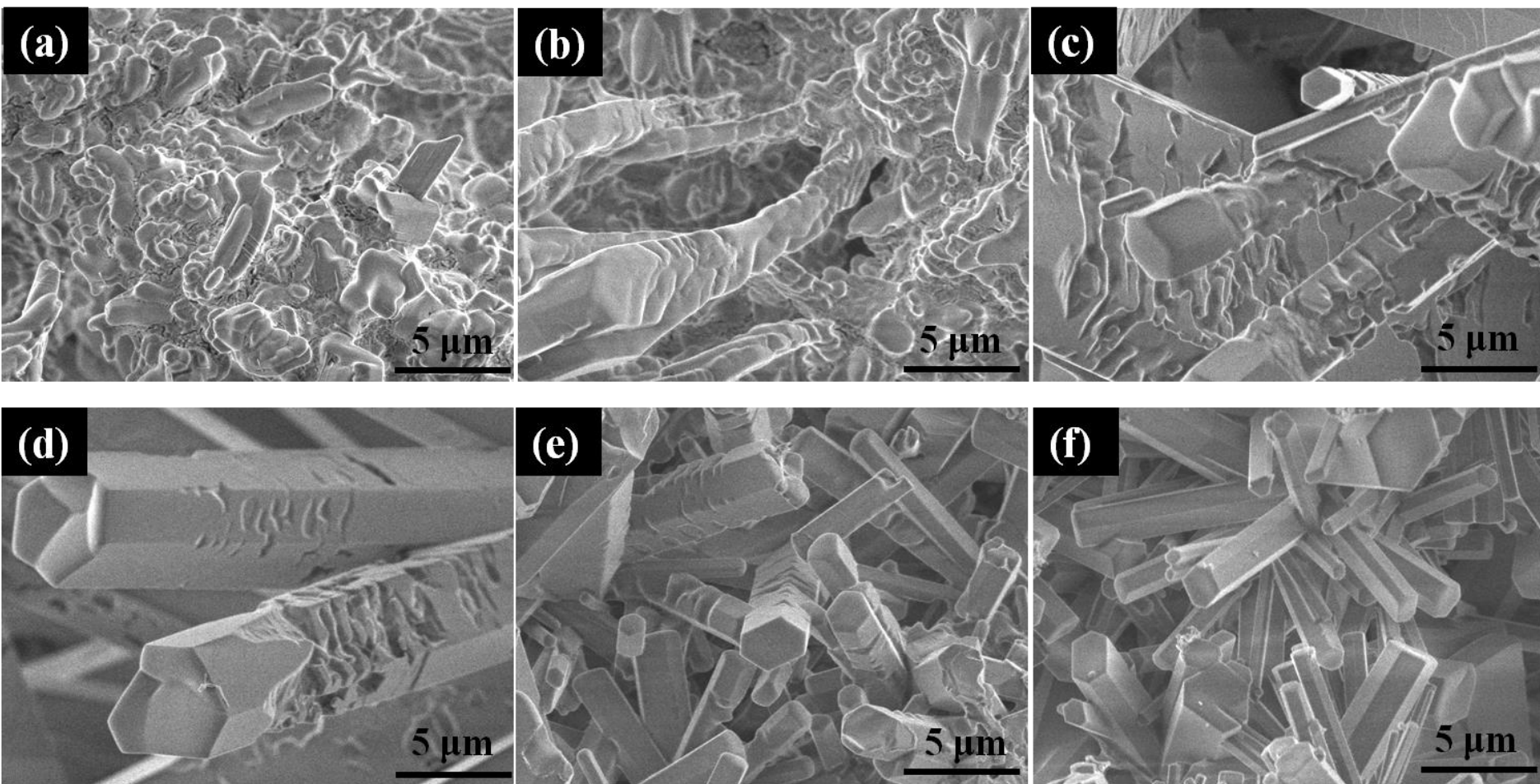
Fig. 8 SEM images of combustion-synthesized \beta -SiAlON powders obtained using (a, b) 22 mass% \text{CaCl}_2 and (c-f) 12 mass% \text{CaCl}_2 .
