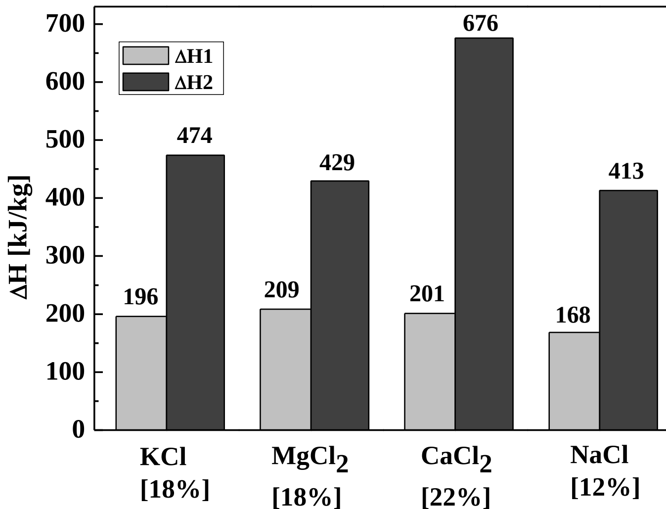
Fig. 4 Change in enthalpy of raw materials ( \Delta H , kJ/kg) for the addition of optimized amounts of KCl (18 mass%), MgCl 2 (18 mass%), and CaCl 2 (22 mass%), along with \Delta H for NaCl is listed here, which were calculated from their absorbed heat values corresponding to the two exothermic processes.
