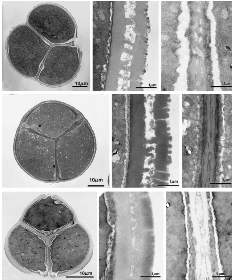
Fig. 4. TEM micrographs of Rhododendron pollen. A-C) Rhododendron schlippenbachii (Sarwar & Takahashi s.n.); D-F) R. japonicum (Takahashi 3998); G-I) R. tsusiophyllum (Sawada s.n.). Whole tetrad (A, D, G); apocolpial exine showing thick canalized tectum with supratectal fine gemmae-pila, thick columellae, thick foot layer and thin endexine (B); in septum, tectum fragmentary, two foot layer of adjacent grains sometimes connected by columellae, endexine thick (C); apocolpial exine showing canalized thick tectum with supratectal fine gemmae-pila, thick columellae, thick foot layer and thin endexine (E); in septum, tectum lacking, two foot layer of adjacent grains connected by thin or rudimentary columellae, endexine thick (F, I); apocolpial exine showing thick tectum, columellae, thick foot layer and endexine with (endo) cracks (H).
