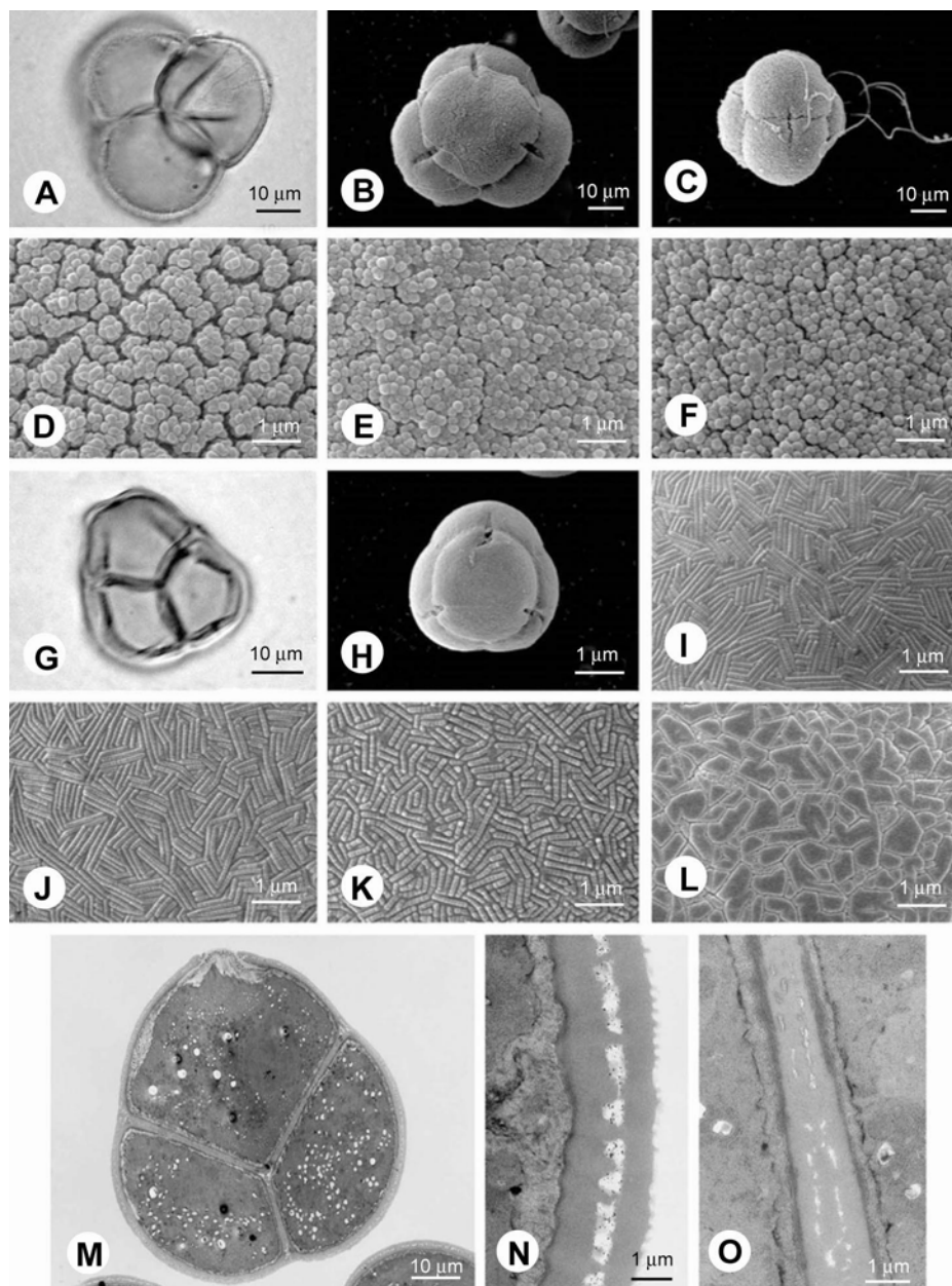
Fig. 5. LM, SEM and TEM pollen micrographs of Therorhodion (A-F) and Menziesia (G-O). A, B) Therorhodion camtschaticum (Takahashi et al. 5836); C) T. redowskianum (Yoshimura & Hara s.n.); D) T. camtschaticum (Takahashi et al. 5836); E, F) T. redowskianum (Yoshimura & Hara s.n.). G) Menziesia pentandra (Takahashi 2687); H) M. multiflora (Takahashi 767); I, J) M. cilicalyx (Tateishi & Hoshi 13689); K) M. multiflora (Takahashi 767); L) M. pentandra (Takahashi 2687); M-O) M. pentandra (Takahashi 2687). Pollen tetrads at polar view (A, B, G, H); pollen tetrads at equatorial view showing aperture (C); micrographs with apocolpial exine sculpture details (D, E, I, K, L); micrograph with mesocolpial exine sculpture details (F, J); whole tetrad (M); apocolpial exine showing tectum with narrow straight-edged striae, columellae, foot layer and thin undulated endexine (N); septum with tectum, and well defined columellae and foot layer of two adjacent grains (O).
