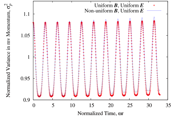
Fig. 4 Time evolution of variance \sigma_p^2 = \langle \mathbf{p}^2 \rangle - \langle \mathbf{p} \rangle^2 in mechanical momentum \hat{\mathbf{p}} = -i\hbar\nabla - q\mathbf{A} for initial speed of v_0 = 5 , E = 10^{-4} , and B = 1 with L_B = \infty or L_B = 10^4 .
