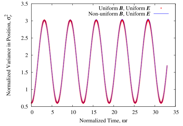
Fig. 3 Time evolution of variance in position \sigma_r^2 = \langle \mathbf{r}^2 \rangle - \langle \mathbf{r} \rangle^2 for initial speed of v_0 = 5 , E = 10^{-4} , and B = 1 with L_B = \infty or L_B = 10^4 .
