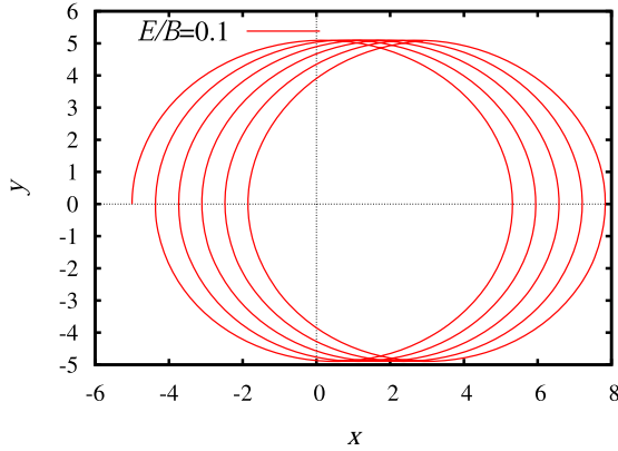
Fig. 2 Time evolution of the expectation of position \langle \mathbf{r} \rangle for \mathbf{r}_0 = (-5, 0) , m\mathbf{v}_0 = (0, 5) , B = 1 and E = 0.1 . Since normalized period of gyration is 2\pi , the drift speed (\langle x(2\pi) \rangle - \langle x(0) \rangle) / 2\pi is close to E/B = 0.1 .
