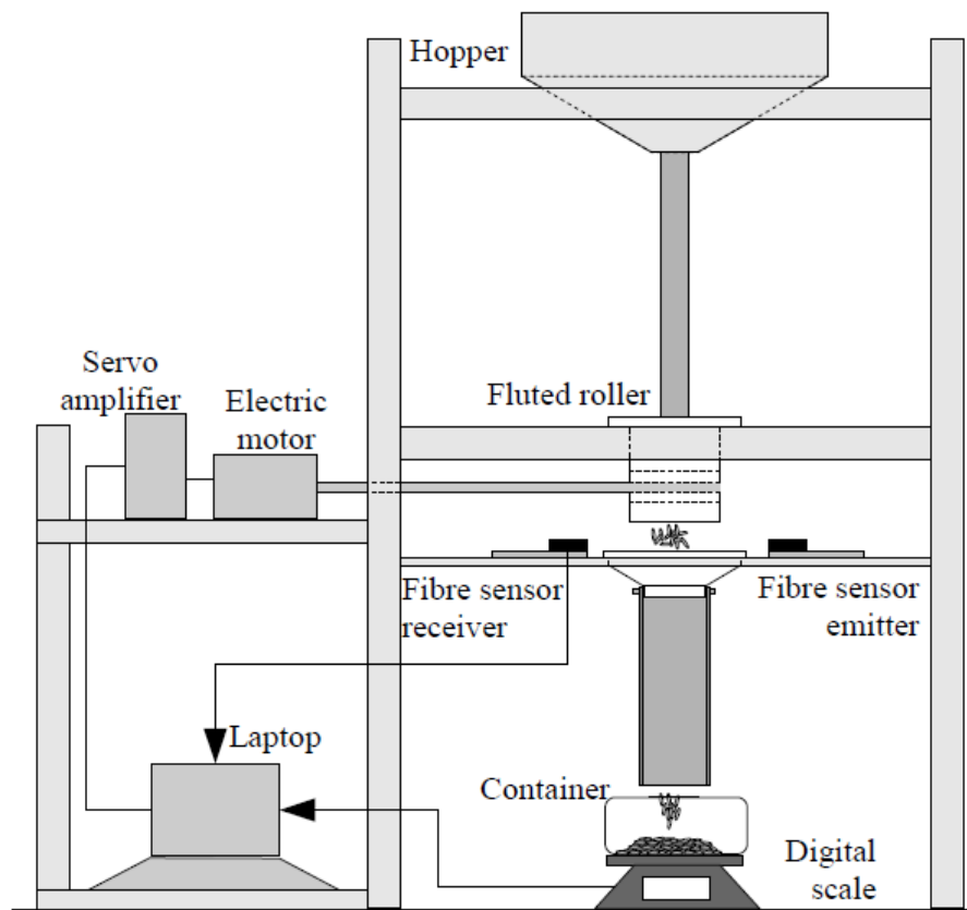
Figure 2. Indoor apparatus which resembles the mass flow of seeds in grain drill
