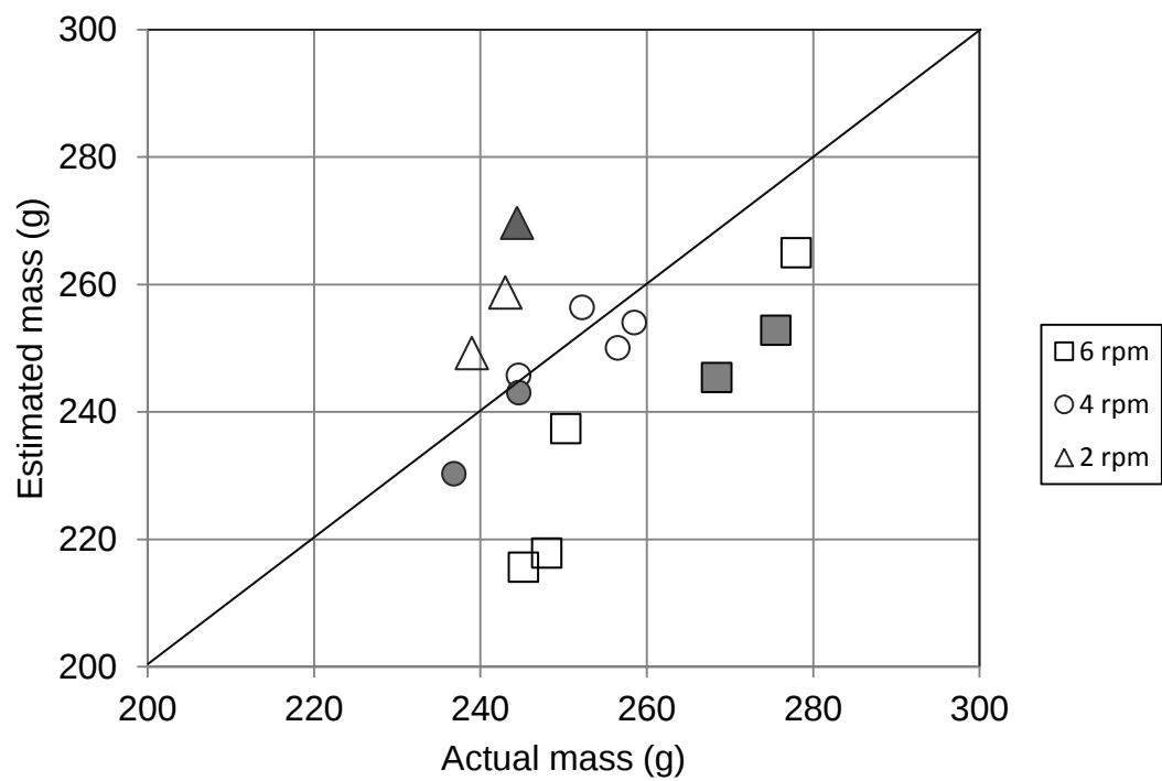
Figure 7. Actual mass measured manually by scale versus estimated mass using the regression model of each entire trial. Solid markers represent the trials whose data were used in modelling.
