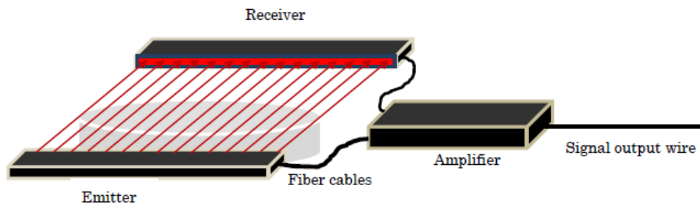
Figure 1. Sketch of the components of the digital fibre sensor (amplifier, emitter, receiver, and fibre cables). The beam of light from the emitter toward the receiver covering the area in which seeds fall
