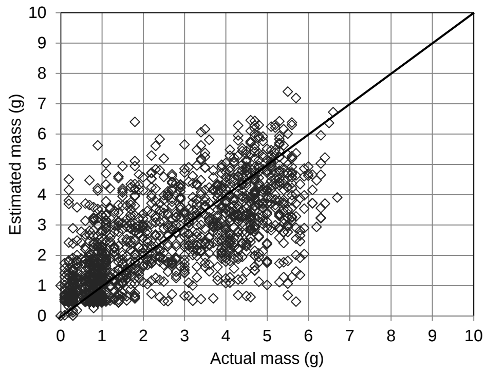
Figure 6. Actual mass measured manually by scale versus estimated mass using the regression model for 1903 clumps when the time interval was 0.8 s
