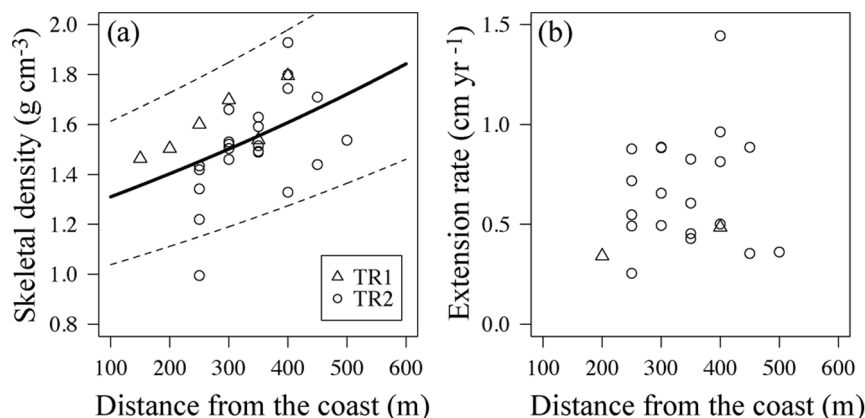
Figure 4. Relationships between (a) skeletal density and (b) extension rate and distance from the coast at TR1 (triangle) and TR2 (circles) in the Todoroki Estuary. Solid and dotted lines indicate the mean curve and 95% prediction intervals, respectively. doi:10.1371/journal.pone.0088790.g004
