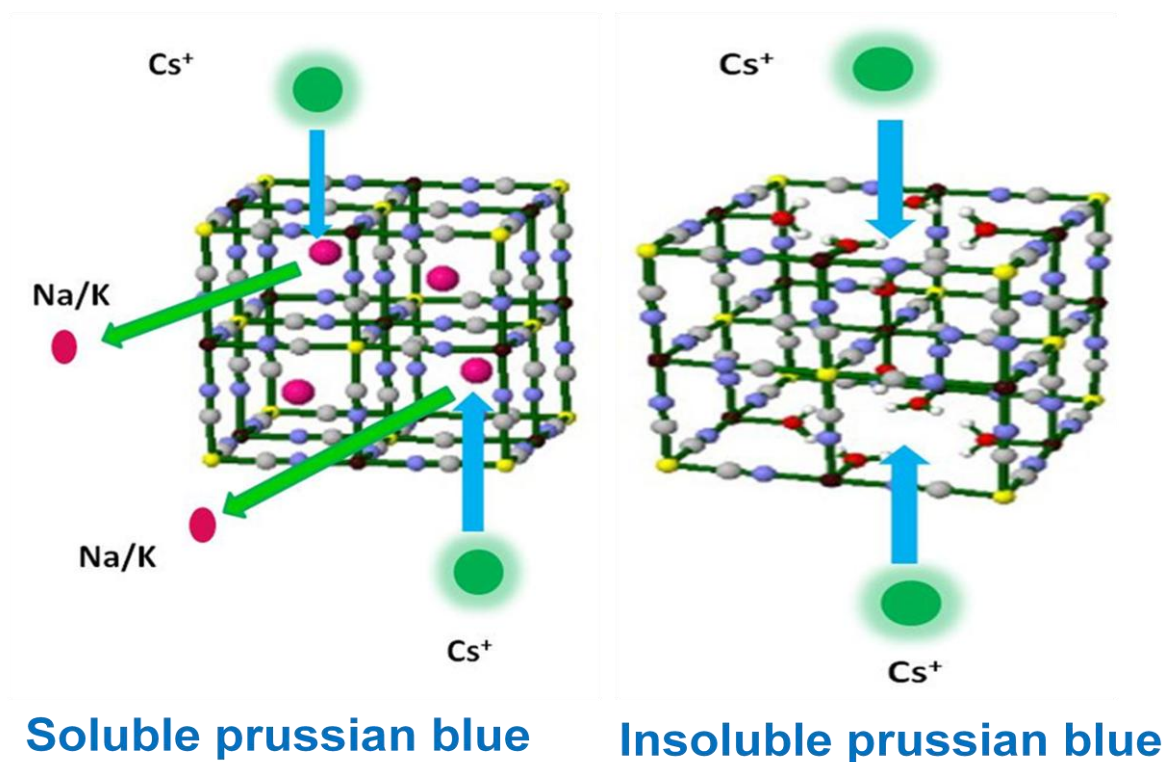
Figure 1-1 Schematic representation of cesium uptake by soluble and insoluble PB
