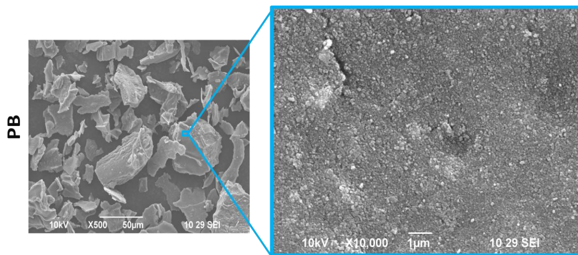
Figure 3-1 SEM images of PB crystals
