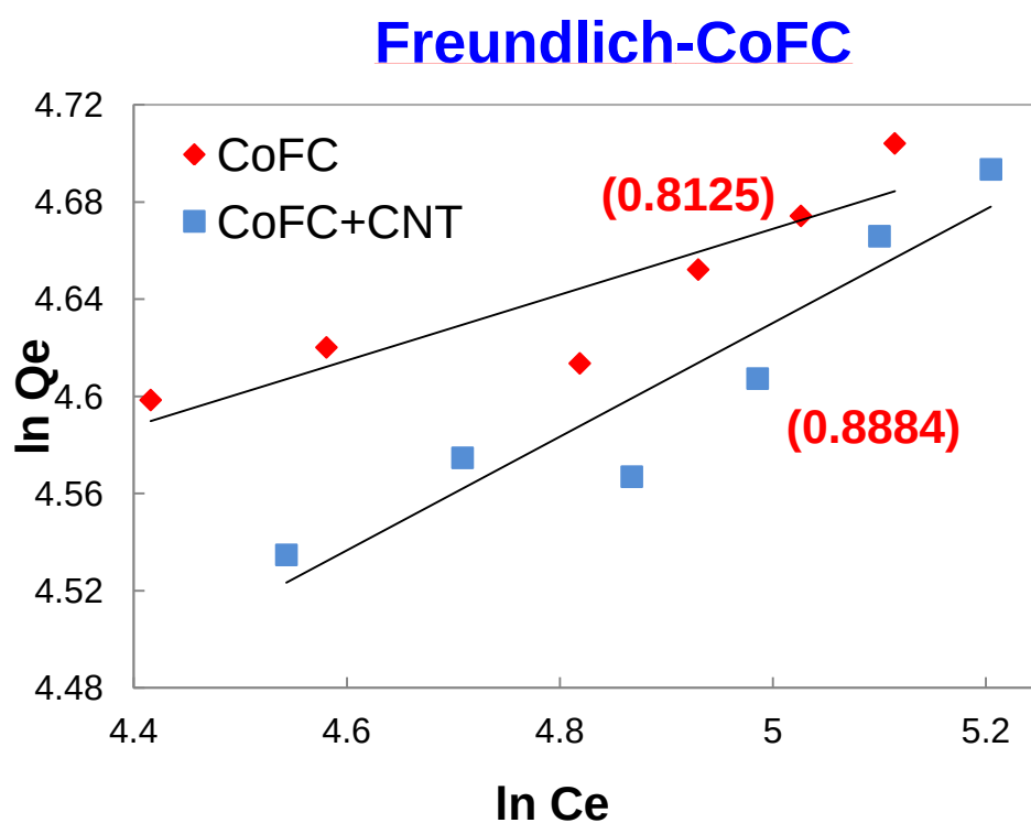
Figure AII-3. Linear plots of Langmuir and Freundlich isotherm model of cesium adsorption by CoFC and CoFC+CNT beads
