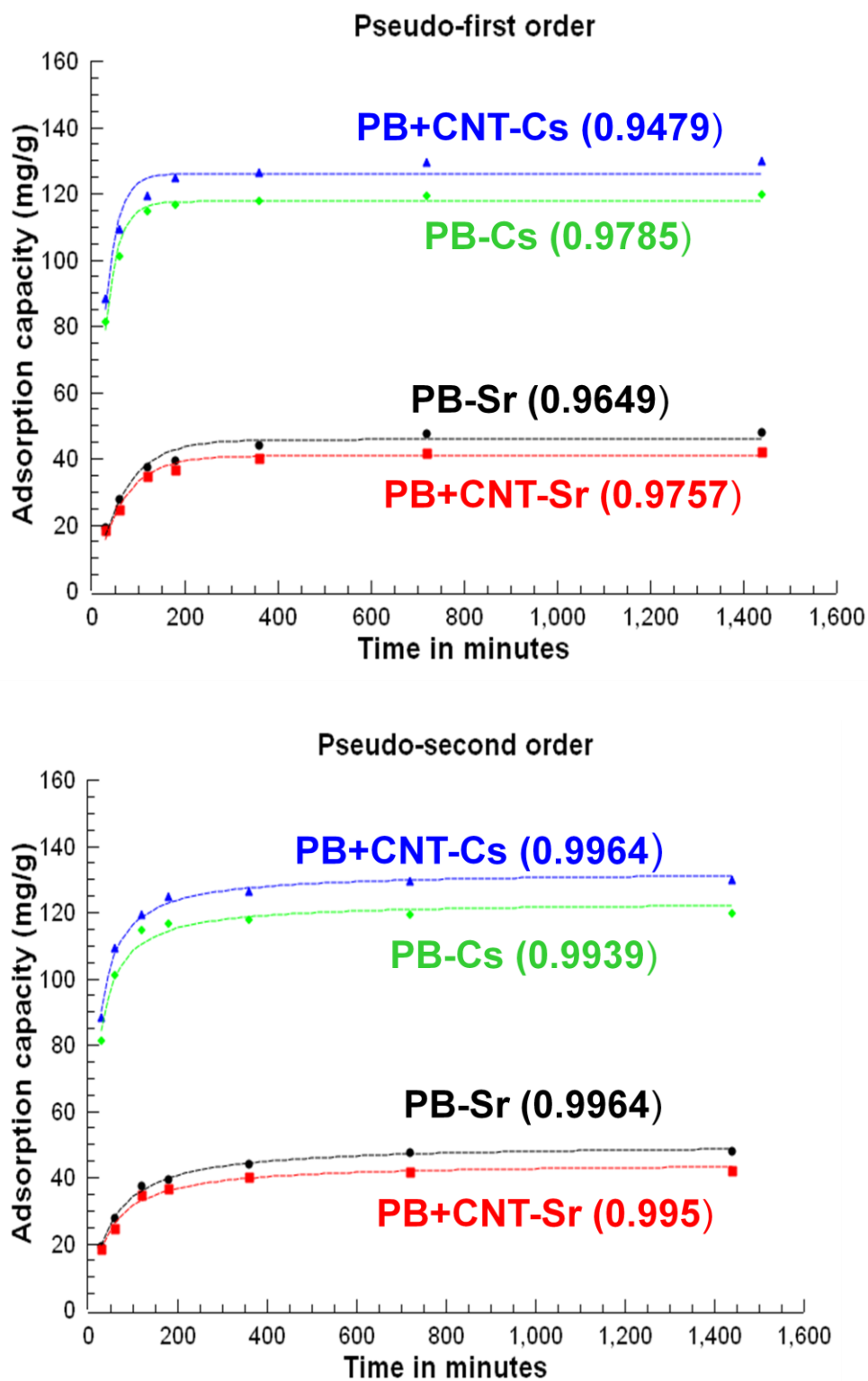
Figure AII-7. Non linear plots of kinetic model of cesium and strontium adsorption by PB and PB+CNT beads
