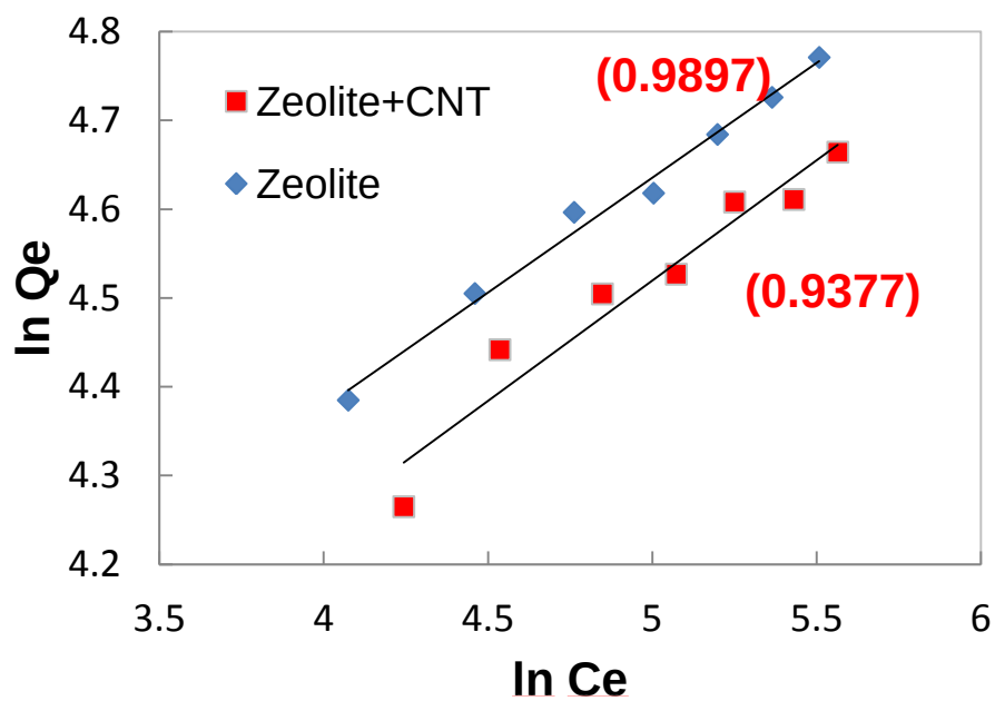
Figure AII-5. Linear plots of Langmuir and Freundlich isotherm model of cesium adsorption by Zeolite and zeolite+CNT beads
