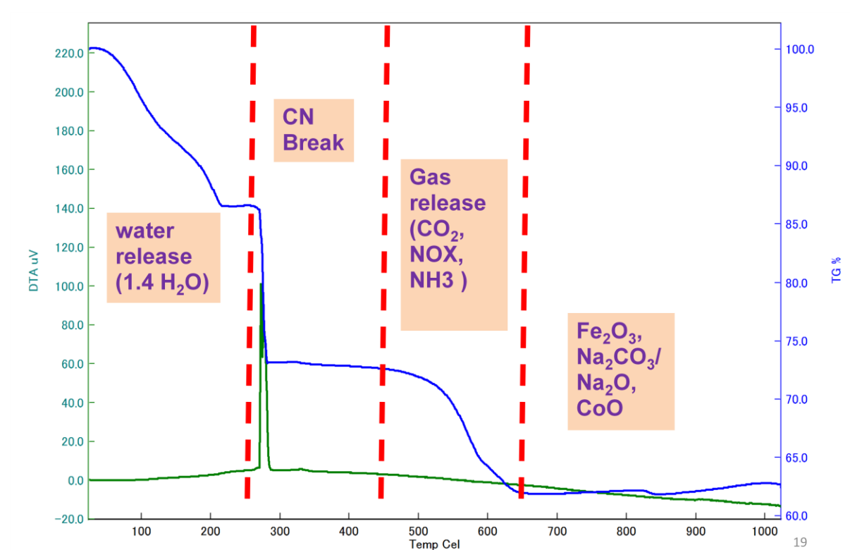
Figure 3-4 TGA thermogram of CoFC
