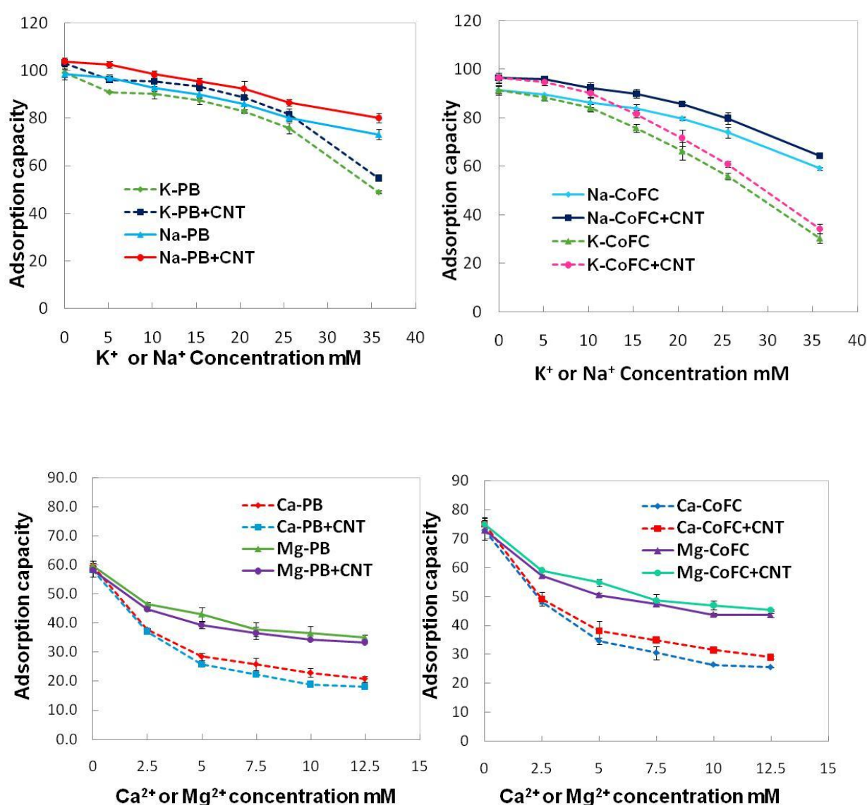
Figure 3-26 Effect of competitive ions on adsorption of cesium and strontium ions
