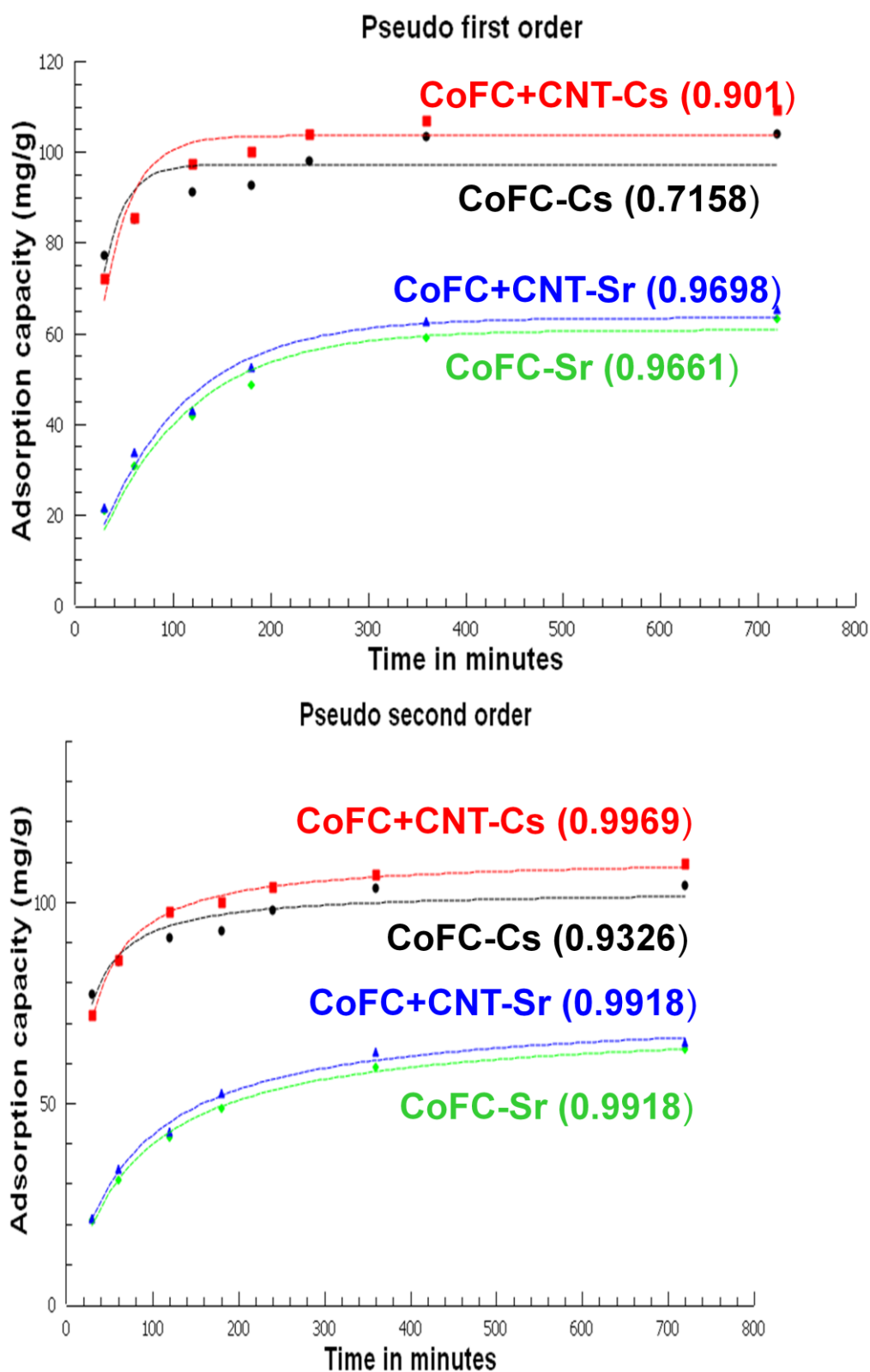
Figure AII-8. Non linear plots of kinetic model of cesium and strontium adsorption by CoFC and CoFC+CNT beads
