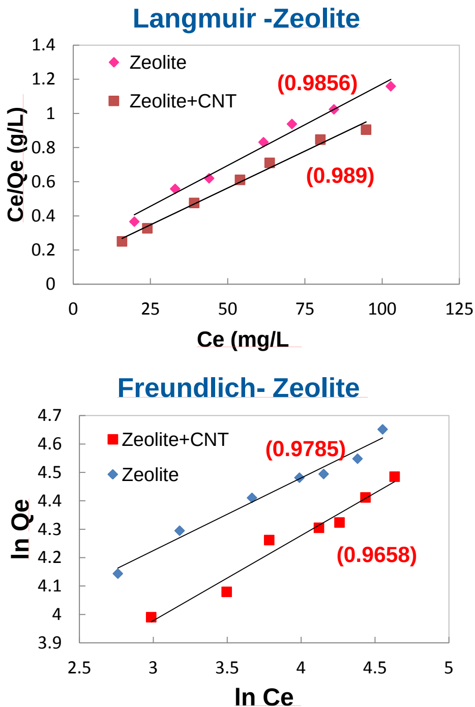
Figure AII-6. Linear plots of Langmuir and Freundlich isotherm model of strontium adsorption by Zeolite and zeolite+CNT beads
