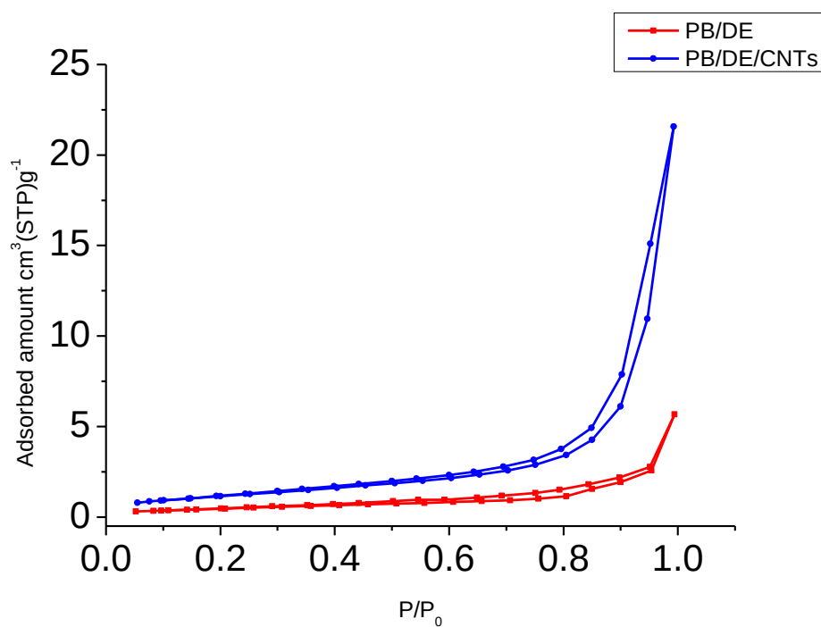
Figure 2-13. Nitrogen adsorption isotherms of Prussian blue/diatomite and CNTs-network/Prussian blue/diatomite samples.
