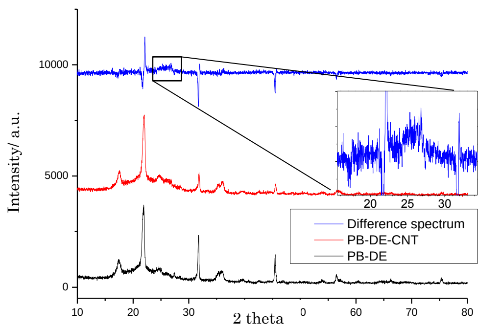
Figure 2-12. The powder X-ray diffraction patterns of Prussian blue/diatomite and CNTs-network/Prussian blue/diatomite samples
