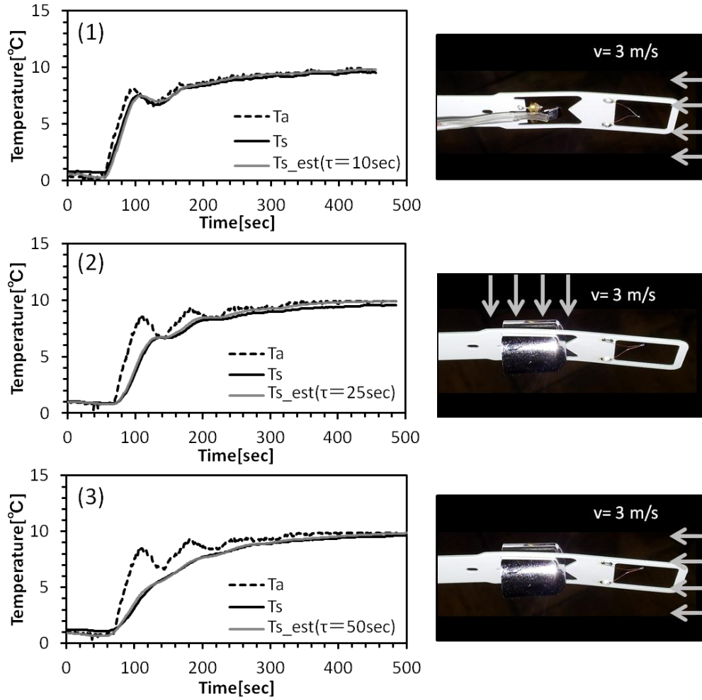
Fig. 2.6. Temperature profiles of the RS-06G RH sensor in response to a stepwise change in air temperature in a chamber (left), and photo showing the three different measurement conditions (right). Dashed lines show applied air temperature, black lines show the change in the sensor's surface temperature, and gray lines show estimated sensor temperatures; i.e., air temperature data filtered with Eq. (5) using the indicated value of \tau .
