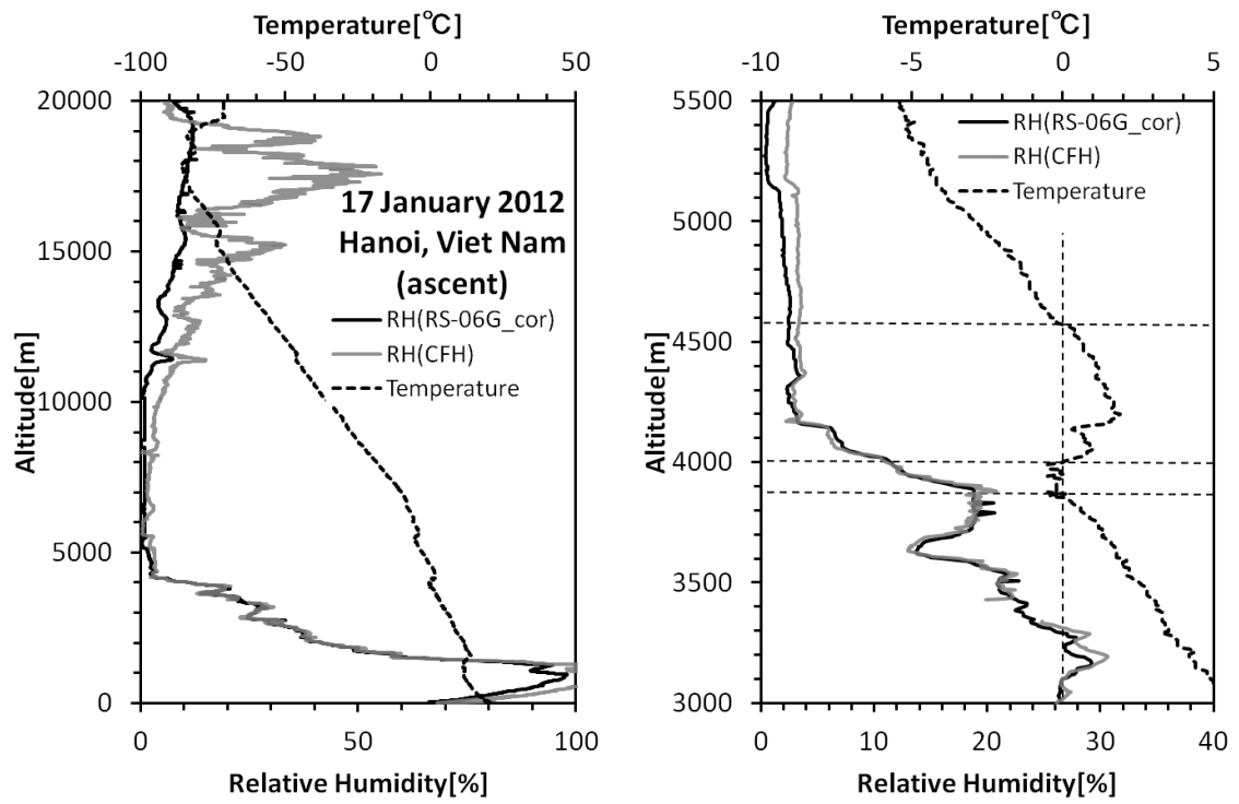
Fig. 2.12. As in Fig. 2.2, but for the RS-06G RH profiles with the new correction applied.
