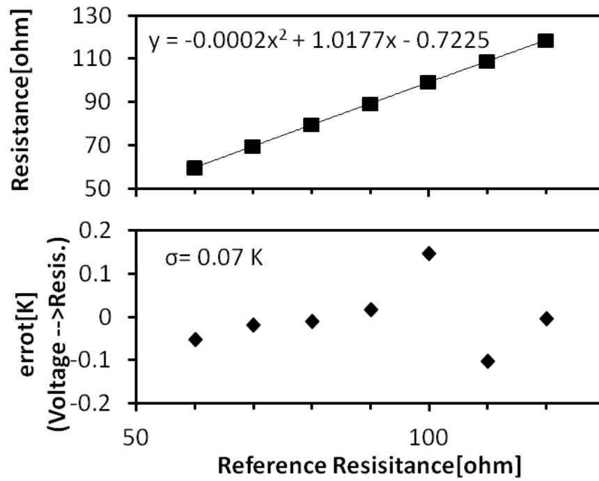
Fig. 3.6 Relationship between the reference resistance and the resistance measured by the developed circuit (top panel), and the error derived from the calibration fit (bottom panel). This error is converted from the resistance unit into temperature unit by using the relationship shown in Fig.3.7.
