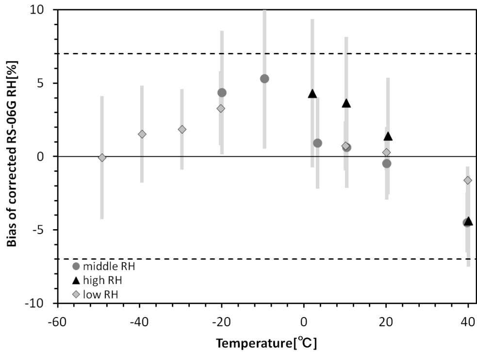
Fig. 2.11. Expected biases in the RS-06G RH measurements during a tropospheric balloon ascent based on the temperature and RH dependence of the sensor material and the thermal lag of the RH sensor. The results are indicated by gray squares (for < 30\% RH), dark gray circles (for 30\% to 70\% RH), and black triangles (for > 70\% RH) show that there remains a wet bias ( < 5\% RH) at -40 to +10 °C. Vertical light gray bars represent the uncertainty ( k = 2 ). Dashed lines show \pm 7\% RH, which indicate the manufacturer's specifications.
