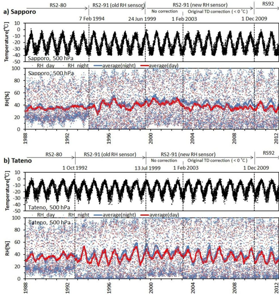
Fig. 2.1. Time series of temperature (top panels, black) and relative humidity (RH) (bottom panels, red and blue) at 500 hPa at Sapporo (a) and Tateno (b), using the original IGRA data. Dots represent the 12-hourly daily RH data and solid lines represent 4-month running averages, to improve the presentation, for the daytime (red) and nighttime (blue) measurements.
