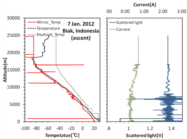
Fig. C.4 A profile of the 4th sounding taken at Biak, Indonesia on 7 January 2012 (daytime, 17:27LT).
