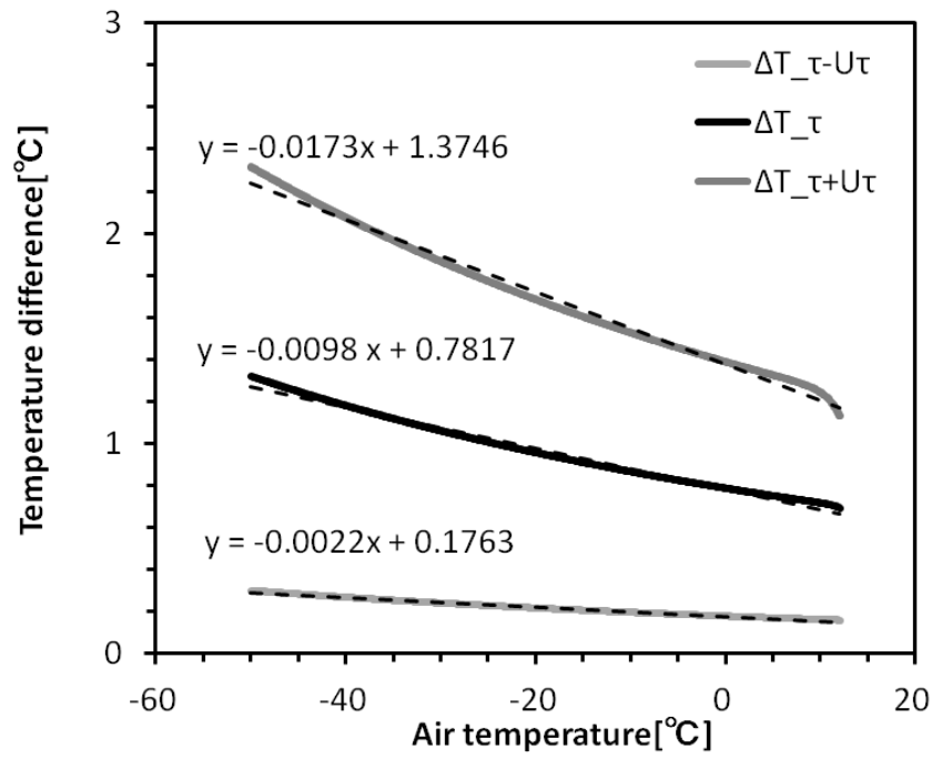
Fig. 2.8. Temperature difference shown in the right panel of Fig. 2.7 against the ambient air temperature shown in the left panel of Fig. 2.7. Dotted lines show the linear fit.
