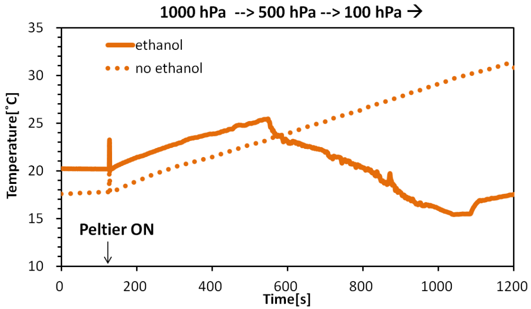
Fig. 3.5 Effect of the ethanol cooling in a pressure-controlled chamber. Solid line indicates the heatsink temperature when the ethanol cooling is used, and dashed line indicates the case where the ethanol is not used. The Peltier current starts to flow at 100 sec. The air pressure is reducing gradually (the approximate values shown at the top). Ethanol starts to be pushed out at ~500 sec for the solid curve case.
