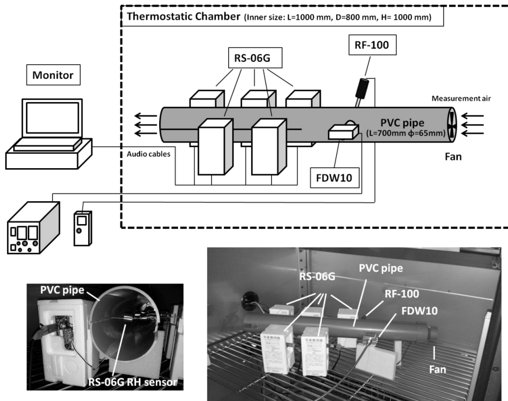
Fig. 2.3. Experimental setup in the thermostatic chamber. The bottom left picture shows the sensor probe of the RS-06G in the PVC pipe. The bottom right picture shows the five RS-06G radiosondes and the two reference instruments set in the PVC pipe.
