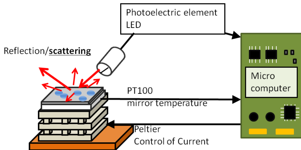
Fig. 3.1 Schematic of the measurement principle of the chilled-mirror hygrometer developed in this study.
