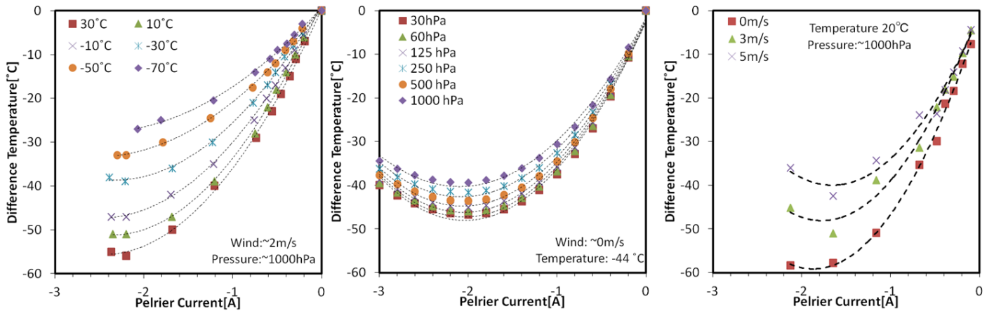
Fig. 3.3 Cooling capability of the Peltier device used in this study. Shown are the temperature differences between the cold side of the Peltier device and the ambient air against the Peltier current under various conditions obtained in a thermostatic chamber. The panels panel show the dependence on (a) air temperature, (b) air pressure, and (c) the airflow rate.
