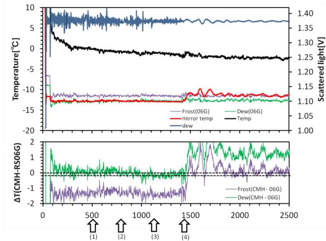
Fig. 3.14 Time series of the mirror temperature and dew/frost point temperature calculated from the Meisei RS-06G air temperature and RH in the laboratory. The RH from RS-06G is corrected by a dry bias of 2.5%RH constant which is probably due to sensor aging (Shimizu et al, 2007). Several months passed after this sensor packing is opened. Differences between the mirror temperature and the frost point temperature (purple line) and dew point temperature are shown (green line).
