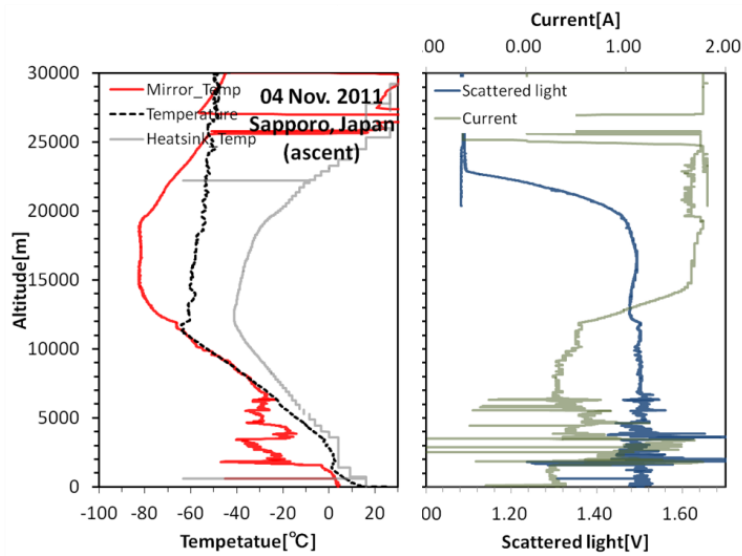
Fig. C.2 A profile of the 2nd sounding taken at Sapporo, Japan on 4 November 2011 (daytime, 14:01LT).
