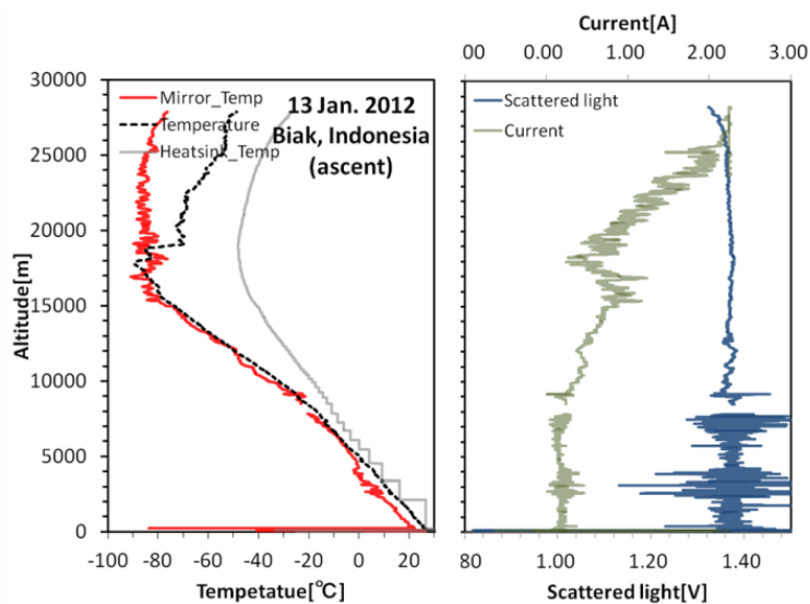
Fig. B.6 A profile of the 6th sounding taken at Biak, Indonesia on 13 January 2012 (daytime, 15:49LT)..
