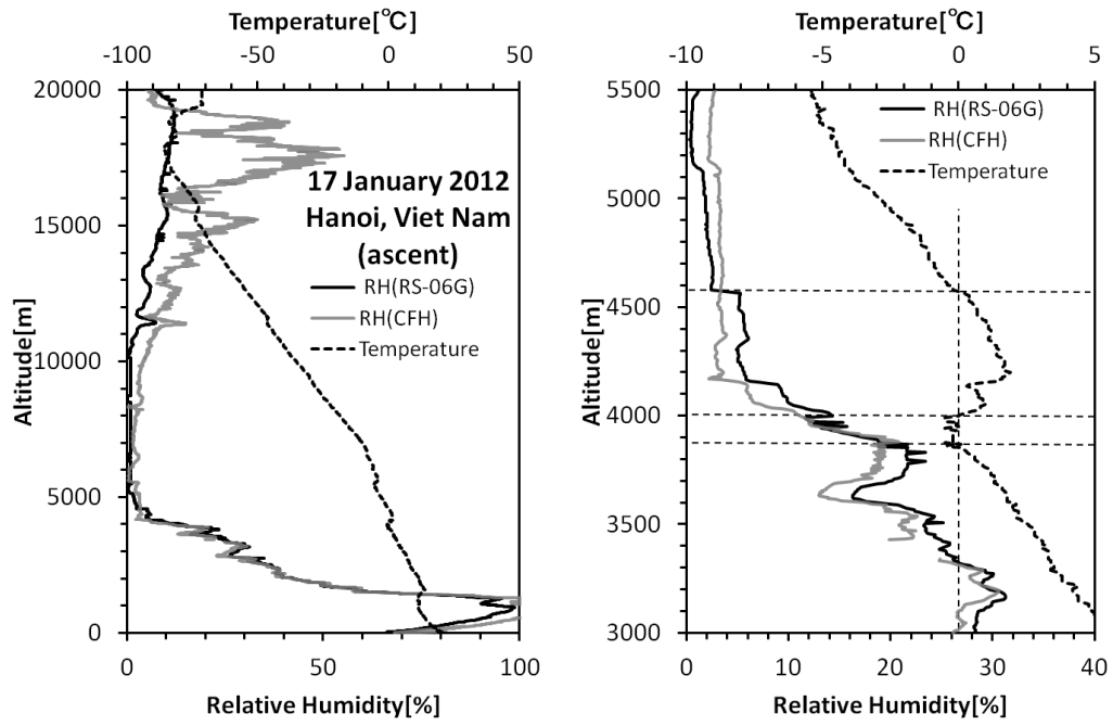
Fig. 2.2. Simultaneous daytime RH profiles from the Meisei RS-06G radiosonde (black) and the CFH (gray) at Hanoi, Viet Nam (21.01°N, 105.80°E). Dashed curves show air temperature measured with the RS-06G. Left panel shows profiles for the whole troposphere, while the right panel shows the region around 0 °C.
