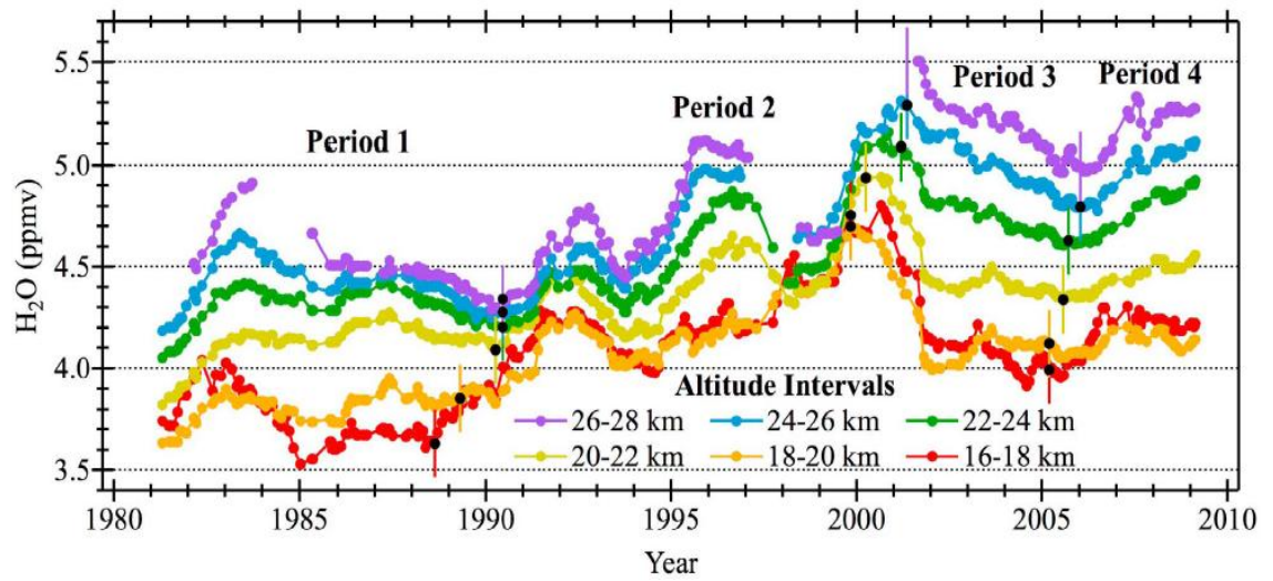
Fig. 1.4 Moving averages of the 2 km water vapor mixing ratio averages in each of the six altitude layers at Boulder, USA measured with the National Oceanic and Atmospheric Administration (NOAA) Frost Point Hygrometer (FPH). The averaging window had a width of \pm 1 year and a threshold of 12 data points to compute an average. (Hurst et al, 2011)
