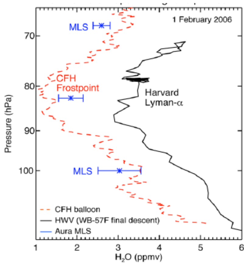
Fig. 1.5 Comparison of water vapor mixing ratios from balloon-borne CFH (red) and airborne HWV (black), and the AURA/MLS (blue) near San Jose, Costa Rica (10°N, 84°W) on 1 February 2006. (Fahey et al. 2009)
