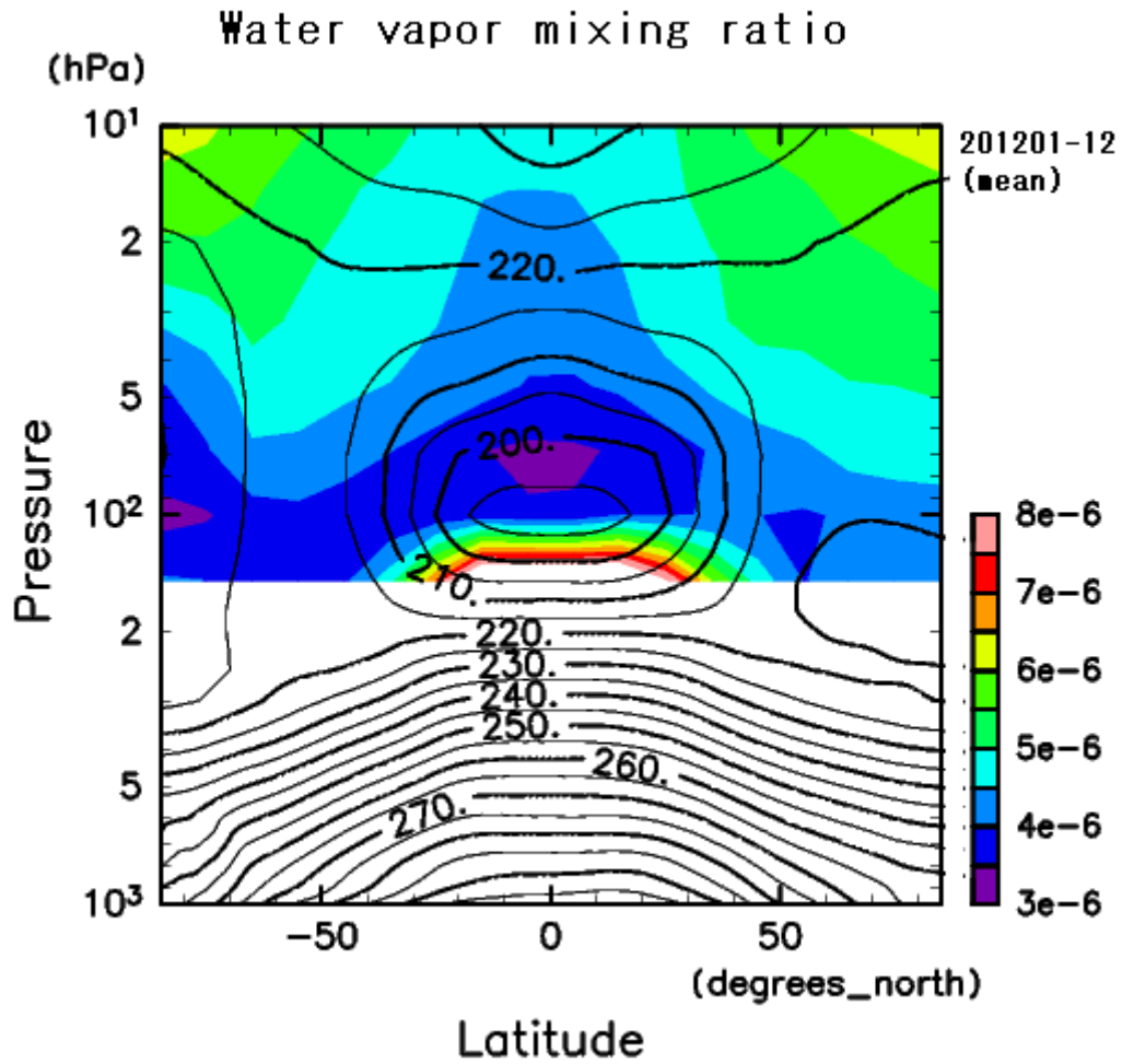
Fig.1.2 Height-latitude cross-sections of the annual mean temperature (contours) and water vapor mixing ratios at 10-147 hPa (color shades) in 2012 as obtained from a reanalysis dataset (ERA-interim) and a satellite data (GozMmlpH 2 O, the H 2 O dataset merged with the HALOE (Halogen Occultation Experiment), the ACE-FTS (Atmospheric Chemistry Experiment - Fourier Transform Spectrometer) and the Aura MLS), respectively.
