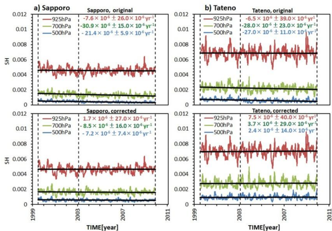
Fig. 2.14. As for Fig. 2.13, but for specific humidity.
