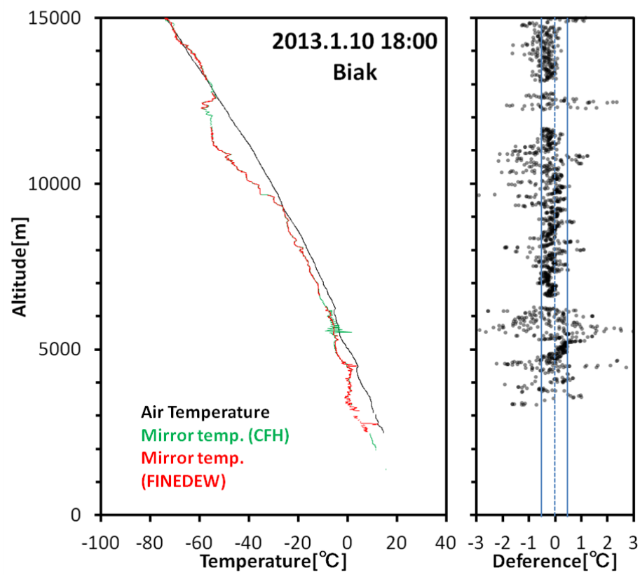
Fig. 3.11 Comparison with the CFH (left), and the difference temperature (right) for the 7th sounding taken at Biak, Indonesia on 10 January 2013.
