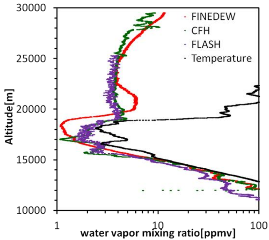
Fig. 3.12 Comparison with the CFH (green line) and FLASH-B (purple line) taken at Biak, Indonesia on 10 January 2012. Water vapor mixing ratio converted from the frost point temperature observed by the developed hygrometer (red), CFH (green), water vapor mixing ratio observed by FLASH-B (purple), and saturation mixing ratio estimated from air temperature (black) are shown.
