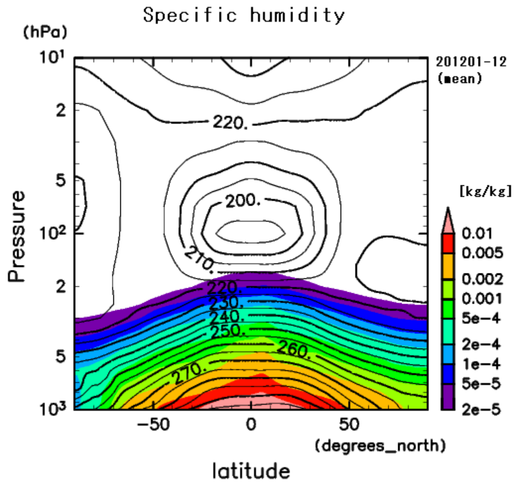
Fig.1.1 Height-latitude cross-sections of the annual mean temperature (contours) and specific humidity in the troposphere (color shades) in 2012 as obtained from a reanalysis dataset (ERA-interim, Dee et al., 2011).
