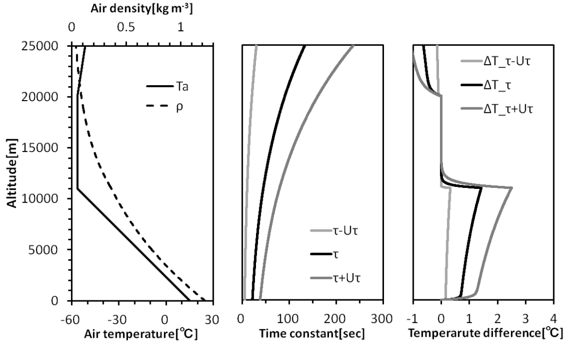
Fig. 2.7. (left) Temperature and density profiles from the U.S. standard atmosphere. (center) The time constant calculated by Eq. (2.9). The black line indicates the value derived from C' = 307 \text{ kg m}^{\frac{1}{2}} \text{ s}^{-2} \text{ K}^{-1} . The light and dark lines indicate the expanded uncertainties, i.e., \tau - U_\tau and \tau + U_\tau . The difference between the RH sensor temperature and ambient air temperature for the three conditions.
