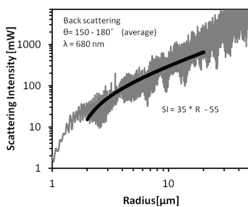
Fig. 3.17 Theoretical relationship between the particle radius and the backscattering intensity, assuming the Mie scattering process. Black line indicates a linear fit.
