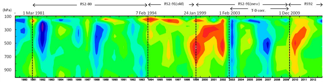
Fig. 2.15. Time series of anomalies of specific humidity in July for each year at 42.75^{\circ}\text{N} , 141^{\circ}\text{E} (the closest grid to the Sapporo station), using a reanalysis dataset (ERA-interim, Dee et al. 2011). The anomaly is with respect to the average for the whole period at each level. Dashed lines represent the change points in instruments.
