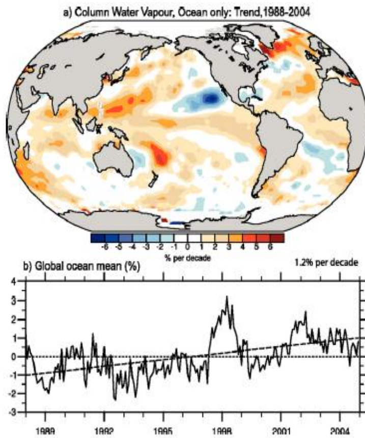
Fig 1.3 Linear trends in precipitable water (total column water vapor) in % per decade(top) and monthly time series of the anomalies over the global ocean (bottom) from SSM/I (Trenberth et al., 2005)
