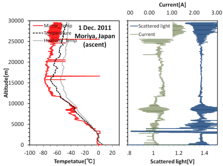
Fig. C.3 A profile of the 3rd sounding taken at Moriya, Japan on 1 December 2011 (nighttime, 17:41LT).
