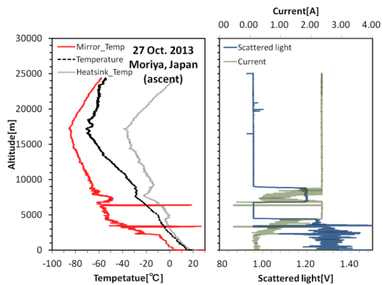
Fig. B.9 A profile of the 9th sounding taken at Moriya, Japan on 27 October 2013 (daytime, 9:10LT).
