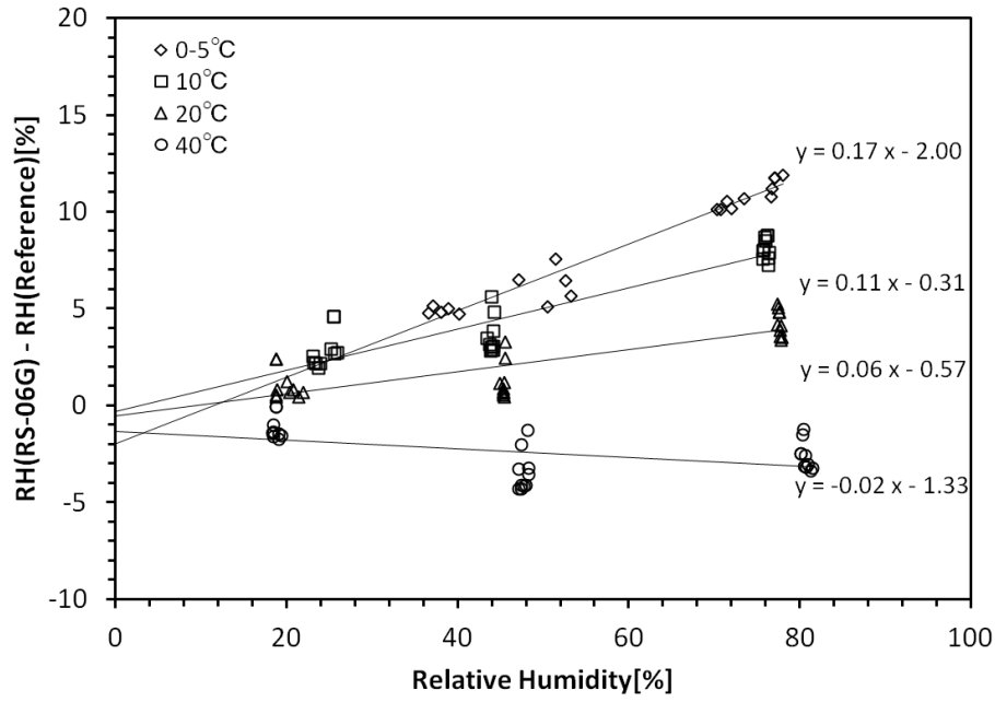
Fig. 2.5 RH dependence of the RS-06G RH measurements under different temperature conditions. The RH difference between the reference and the uncorrected RS-06G RH_0 is indicated by the rhomboids (for 0 to +5° C), squares (for +10 °C), triangles (for +20 °C), and circles (for +40 °C). The lines are linear fits for each temperature group.
