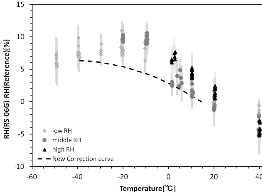
Fig. 2.9. As in Fig. 2.4 (top), but corrected by Eq. (2.16) for a modeled thermal lag effect. The dashed line represents the correction curve extrapolated up to +14.5 °C. Vertical light gray bars represent the estimated magnitude of uncertainty from the thermal lag effect. The marks indicate the value derived from C' = 307 \text{ kg m}^{\frac{1}{2}} \text{ s}^{-2} \text{ K}^{-1} and the upper and lower limits of the light gray vertical bars indicate the uncertainty derived from Eq. (2.13).
