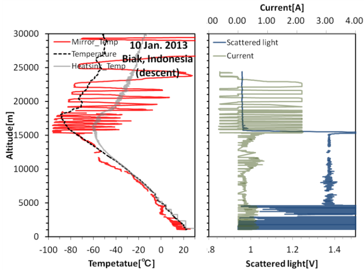
Fig. B.7 A profile of the 7th sounding taken at Biak, Indonesia on 10 January 2013 (daytime, 18:00LT).
