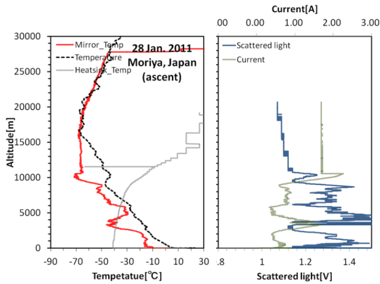
Fig. C.1 A profile of the 1st sounding taken at Moriya, Japan on 28 January 2011(daytime, 14:30LT).
