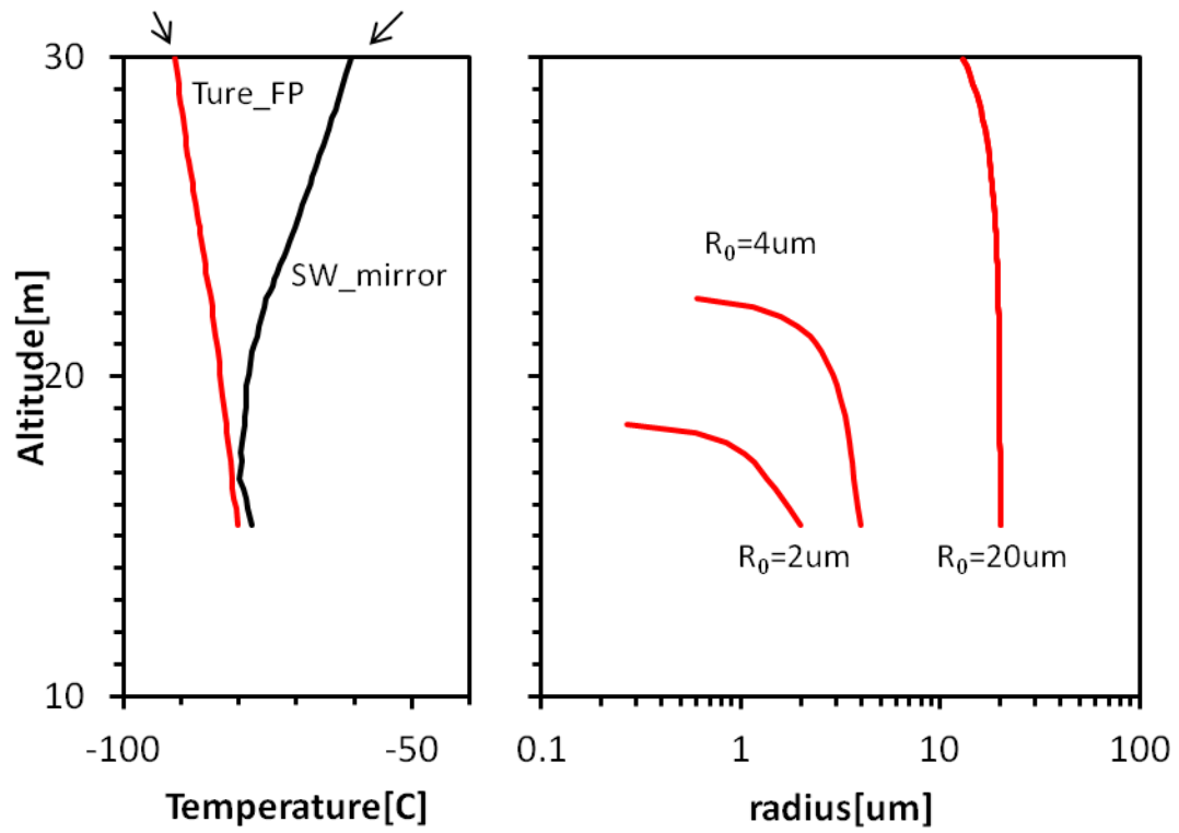
Fig. 3.21 Evaporation rate of a condensate on the mirror calculated with a simple model, assuming that the ice crystal is spherical shape. See text for the details.
