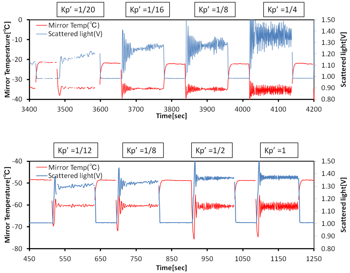
Fig. 3.8 An example of the ultimate sensitive method for T = -20\text{ }^{\circ}\text{C} (top), and for T = -50\text{ }^{\circ}\text{C} (bottom)
