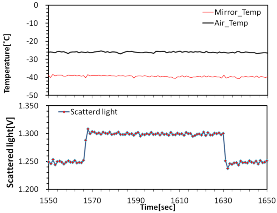
Fig. 3.19 Response of the scattered light intensity for the step functions of the target level of the scattered light intensity (1.25 --> 1.30 --> 1.25). Time series of air temperature and mirror temperature (top) and intensity of scattered light(bottom). For these cases, the stabilization time is within 3 sec.
