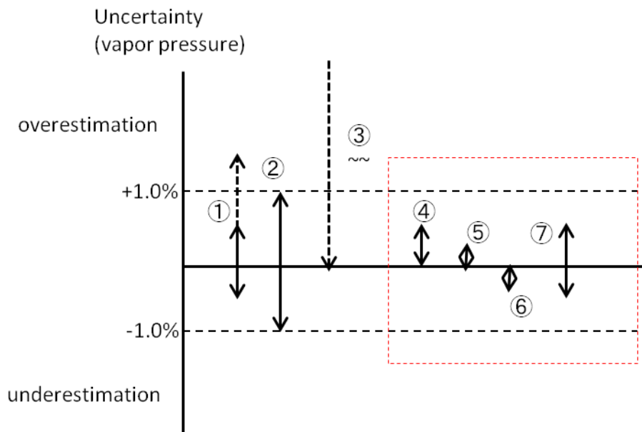
Fig. 3.18 Sources of the measurement uncertainty and its degree. The degree indicates the error of the vapor pressure calculated from the frost point temperature. (1) the mirror temperature measurement, (2) the stability and response of the PID controller, (3) the contamination error by cloud/rain droplet, (4) the ambiguity of the condensate phase, (5) aerosol effects, (6) curvature effect, (7) the uncertainty of the vapor equation s.
