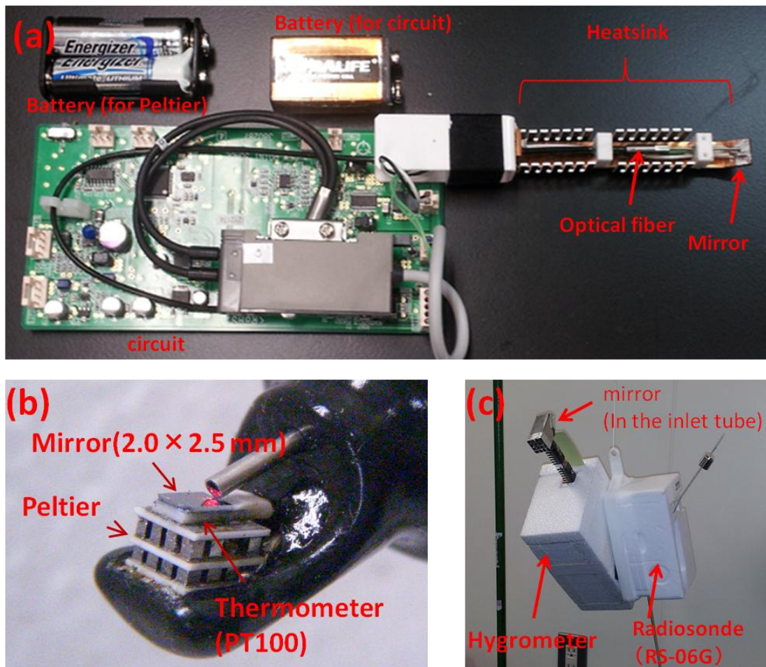
Fig. 3.2 The instrument developed in this study. (a) the sensor probe and electrical circuit, (b) a close-up of the mirror and the Peltier device part, and (c) the flight configuration with the RS-06G radiosonde at the development phase (3)
