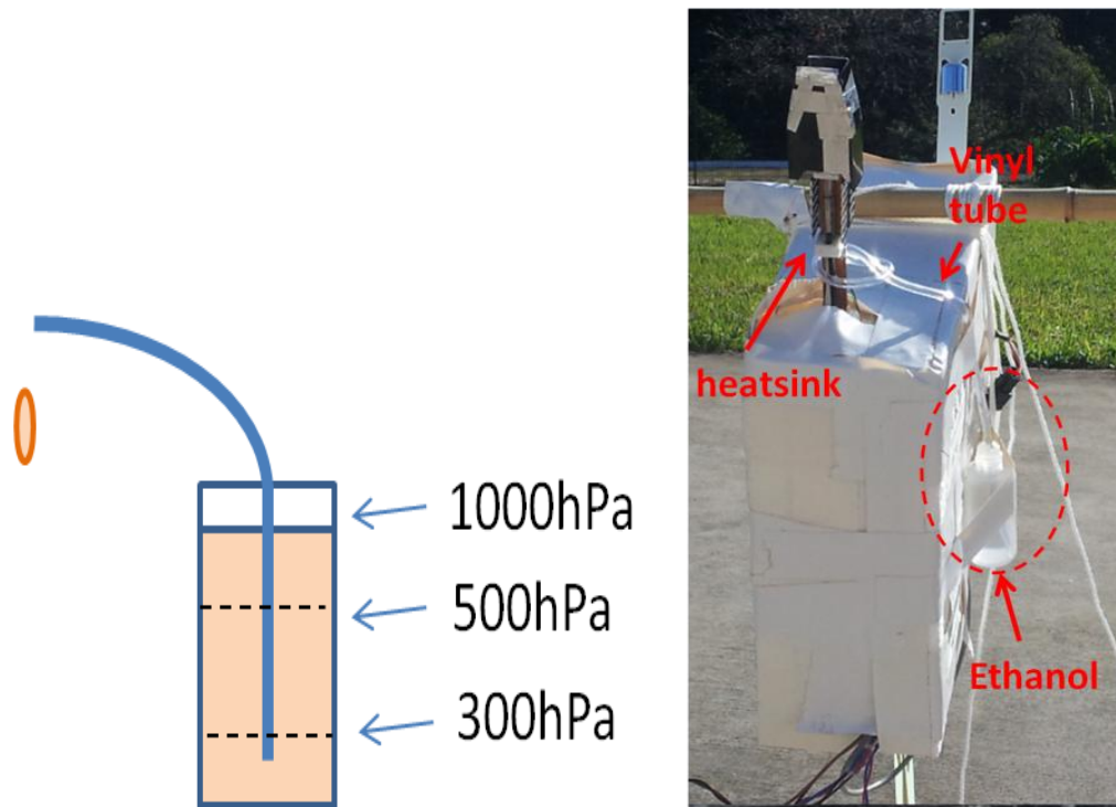
Fig. 3.4 Ethanol bottle for the heatsink cooling. The ethanol is pushed out by the air expansion in the top of bottle in low-pressure conditions.
