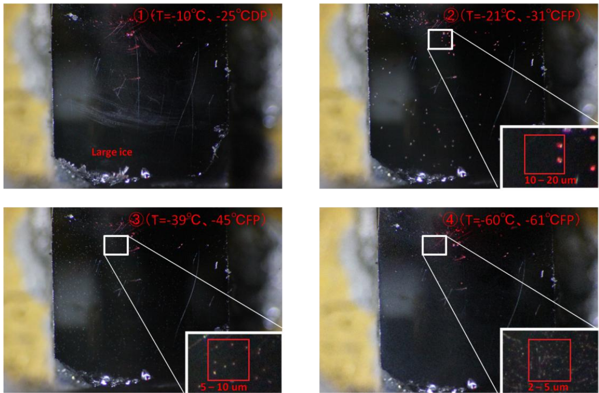
Fig. 3.16 Condensates on the mirror at temperatures of -10, -20, -40, -60°C in the thermostatic chamber.
