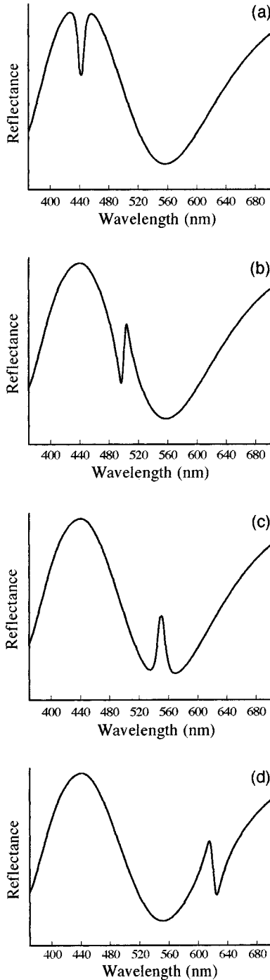
FIG. 2. Illustrative reflection spectra calculated for a ZnSe/MgS SL with the 1700-Å total thickness on GaAs. The exciton peak position was hypothetically assumed to be at (a) 440 nm, (b) 500 nm, (c) 555 nm, and (d) 620 nm to show the change of the exciton features by the position relative to the multiple reflection in the film.
