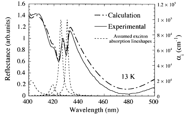
FIG. 3. Reflection spectrum measured on a ZnSe/MgS SL on GaAs (solid line) and its theoretical fit (dot-dashed line). The four peaks (dashed lines) are the exciton absorptions assumed for the theoretical fit.
