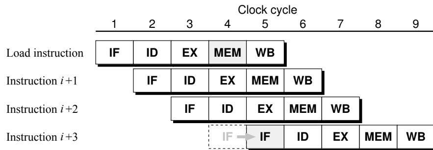
Figure 2.7: Structural hazard
