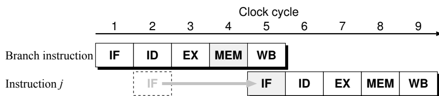
(a) Branch instruction without delayed execution
