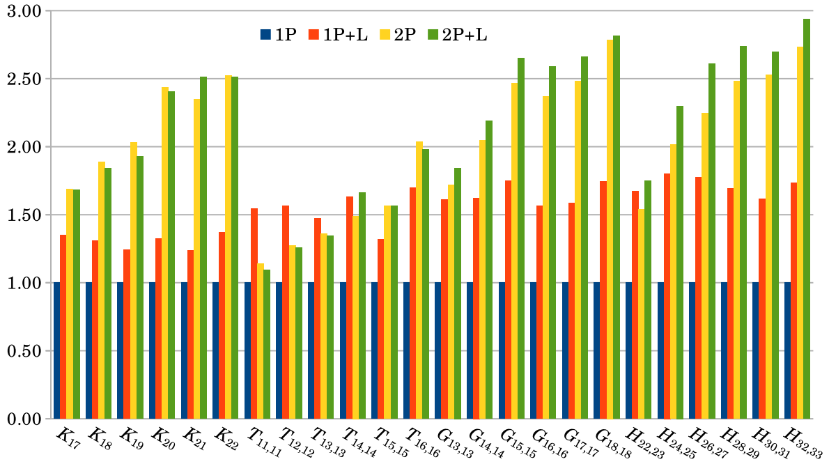
Figure 5.5: Speed ratio for path enumeration
