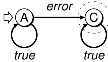
Figure 4.5: Property graph for invariant checking
