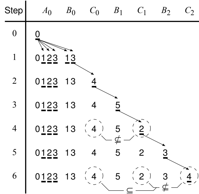
Figure 4.4: Depth-first checking
