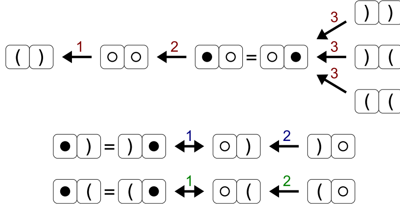
Figure 5.11: Data dependency
