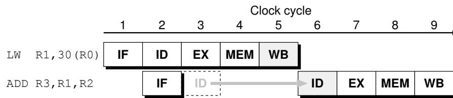
(a) ADD one cycle after LW
