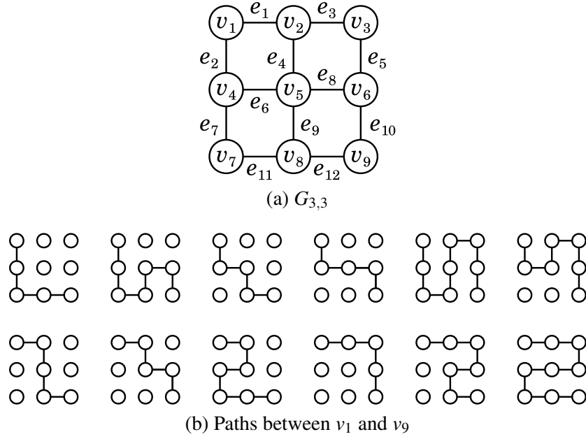
Figure 2.4: Path enumeration on G_{3,3}
