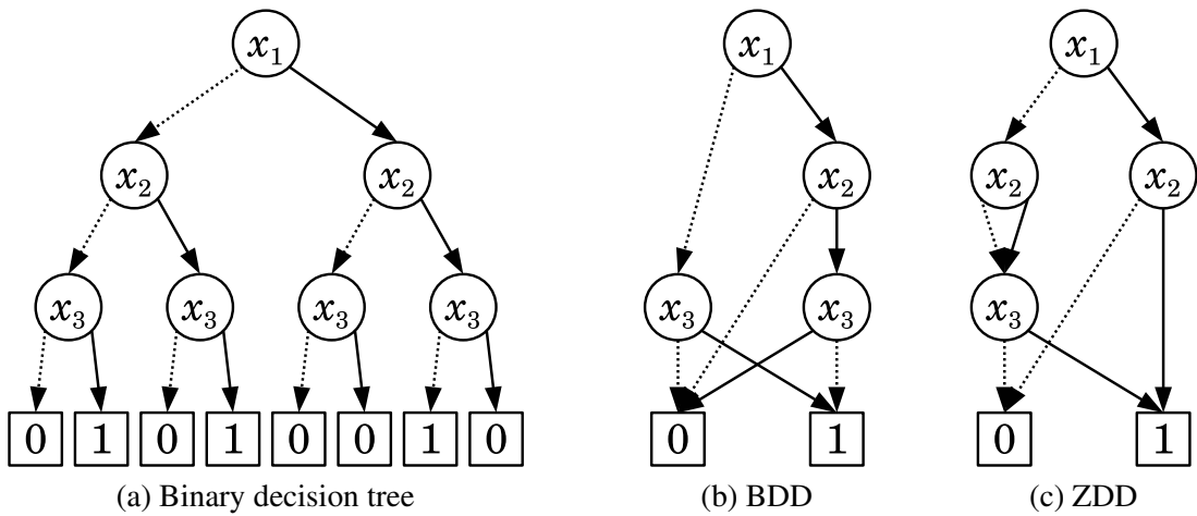
Figure 2.1: Diagrams for f(x_1, x_2, x_3) = x_1x_2\bar{x}_3 + \bar{x}_1x_3
