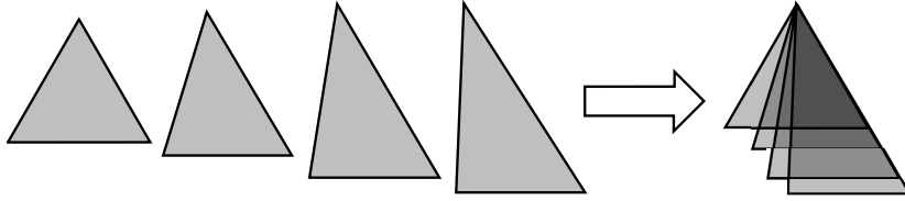
Figure 3.1: Multiplexing the parse trees of AIVF coding into a single tree.
