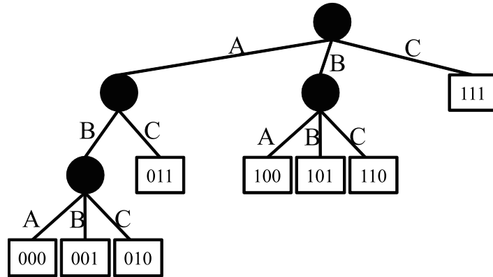
Figure 2.4: Parse tree of the STVF coding for string BABCBABBBABCBAC. The squares and the circles indicate leaves and internal nodes, respectively. The numbers in squares are assigned codewords.
