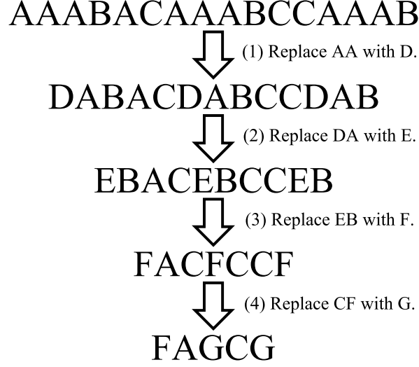
Figure 5.1: Example of Re-Pair algorithm. It repetitively replace the most frequent bigram into a new symbol.
