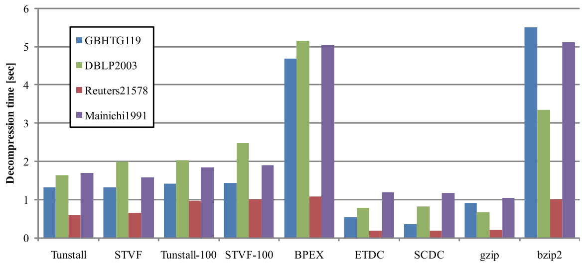
Figure 4.4: Decompression times.
