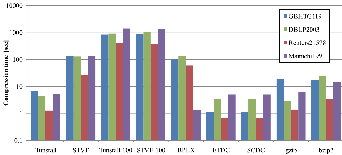
Figure 4.3: Compression times.
