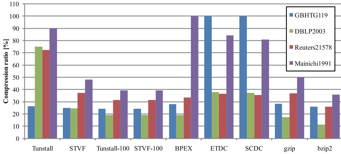
Figure 4.2: Compression ratios.
