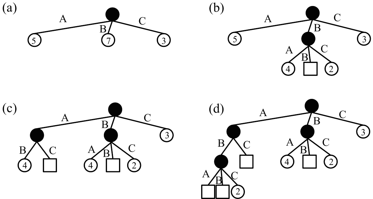
Figure 2.5: The first four iterations of the construction process of the parse tree. The black circles indicate internal nodes. Only leaves are assigned codewords.
