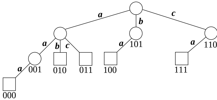
Figure 2.1: Parse tree for method in Section 2.3.1. A circle indicates an internal node and a square does a leaf.
