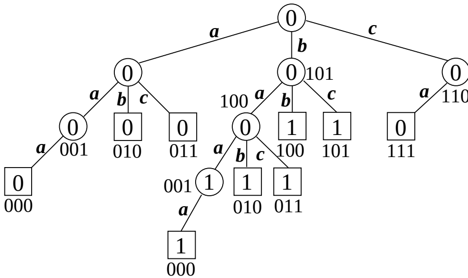
Figure 3.2: An example of VMA tree. This is an integrated tree obtained by multiplexing the trees shown in Figures 2.1 and 2.2. The number written in each node indicates the value of T_n(n) .
