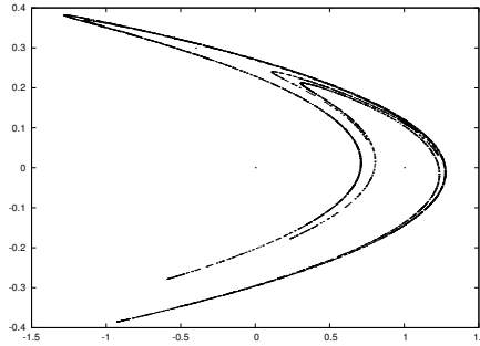
FIGURE 1. The orbits of Hénon map (1) whose initial point is (0, 0) and parameters 1.4 and -0.3 .
