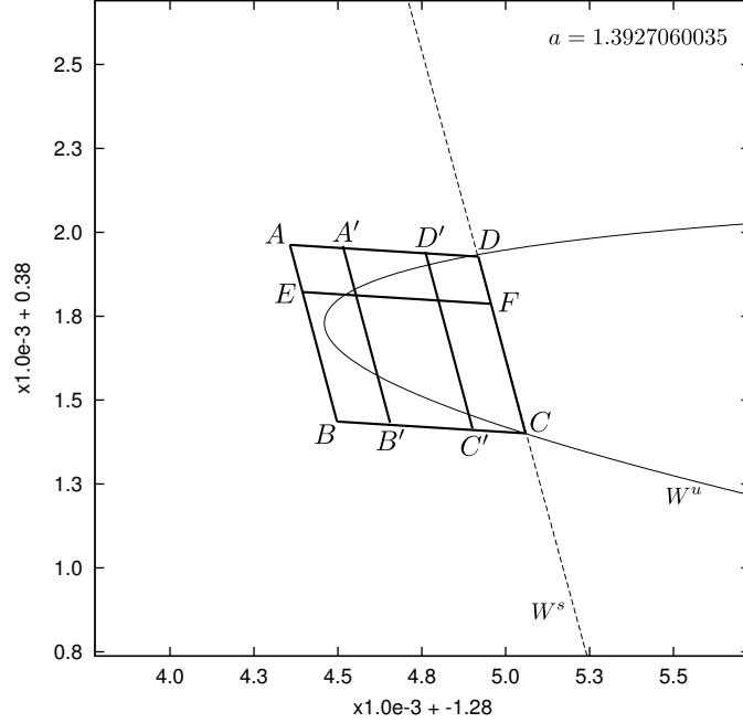
FIGURE 1. The parameters of map (1) are a = 1.3927060035 and b = -0.3 . The points D and C are homoclinic points: the intersections of the stable and unstable manifolds for the saddle periodic point. The parallelogram ABCD includes the segment of the unstable manifold from D to C . The lines AD , EF , and BE are parallel to each other. The lines AB , DC , B'C' , and D'E' are parallel to each other. In ABCD there is a periodic saddle point of period 13.
