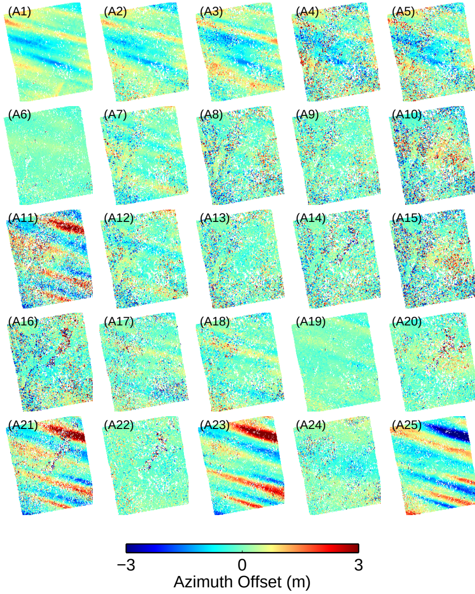
Figure 4.5: Azimuth offsets of ascending orbit data. Details of each pair are listed in Table 4.1.
