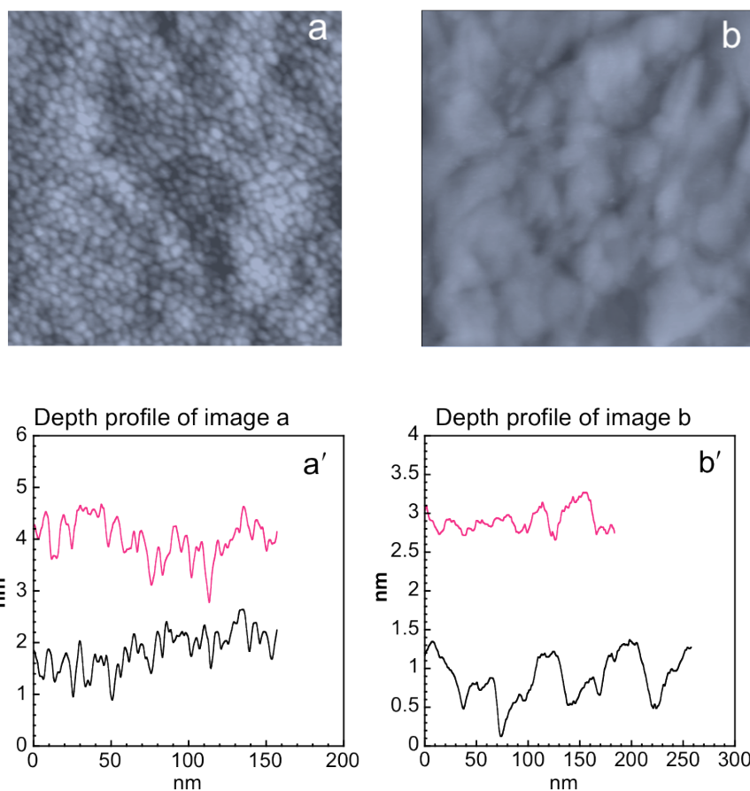
Figure 4.3 STM images of (a) PdPt(sp) and (b) Sn/PdPt(sp) electrodes. a' and b' are the depth profile of image a & b, respectively. The scan size is 200 \times 200 nm. A tip bias voltage of typically 800 mV and a tunneling currents of 300 pA were used.
