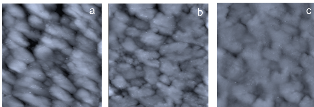
Figure 3.6 STM images of (a) Pd, (b) as-prepared Sn/Pd, and (c) pretreated Sn/Pd electrodes. The scan size is 200 nm x 200 nm. A tip bias voltage of typically 800 mV and a tunneling currents of 300 pA were used.
