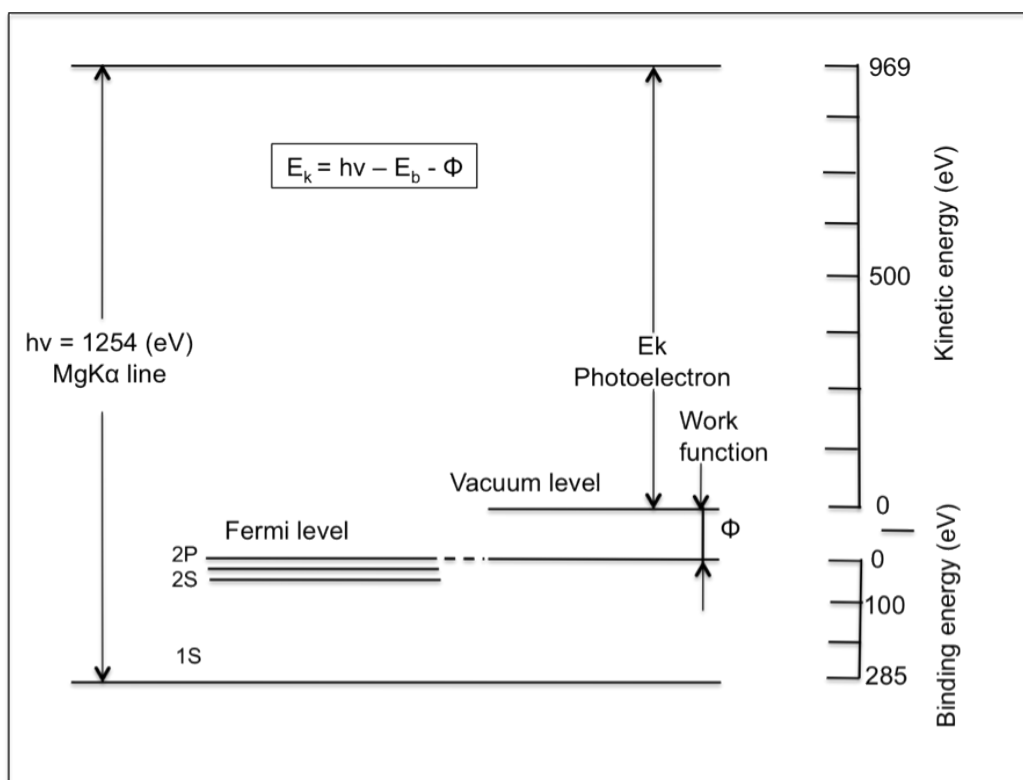
Figure 2.3 Energy diagram of photoelectron emission on carbon atom in XPS.
