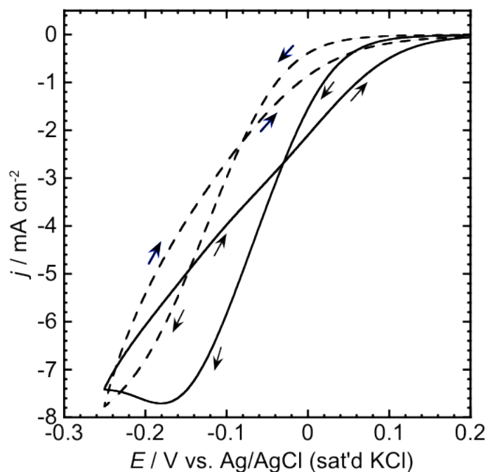
Figure 3.3 Cyclic voltammograms of (dashed curve) as-prepared Sn/Pd, and (solid curve) pretreated Sn/Pd electrodes in 0.01 M NaNO 3 + 0.1 M HClO 4 at the scan rate of 0.01 V s -1 . The tin coverage was 0.89. Electrochemical pretreatment was conducted at -0.35 V for 60 s.
