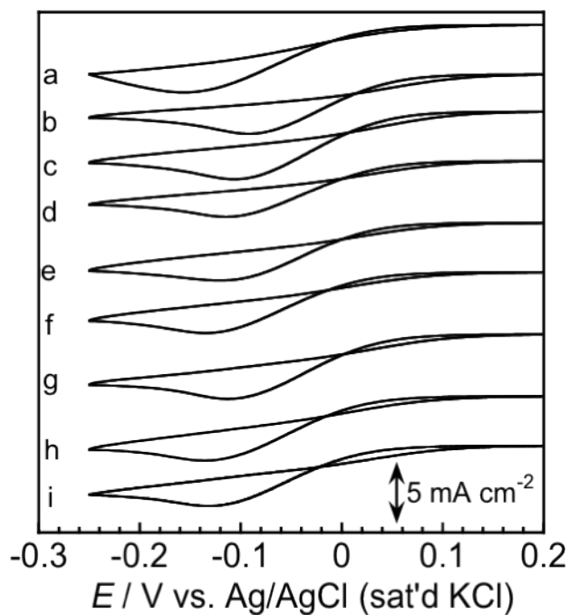
Figure 4.14 CVs for reduction of nitrate on Sn/PdPt electrodes in 0.01 M \text{NaNO}_3 + 0.1 M \text{HClO}_4 . Surface composition (Pd/Pt): (a) 0, (b) 18/82 (c) 28/72, (d) 30/70, (e) 35/65, (f) 40/60, (g) 51/49 (h) 61/39 and (i) 100/0. The Sn coverage was 0.80-0.90 and the scan rate was 0.01 \text{ V s}^{-1} .
