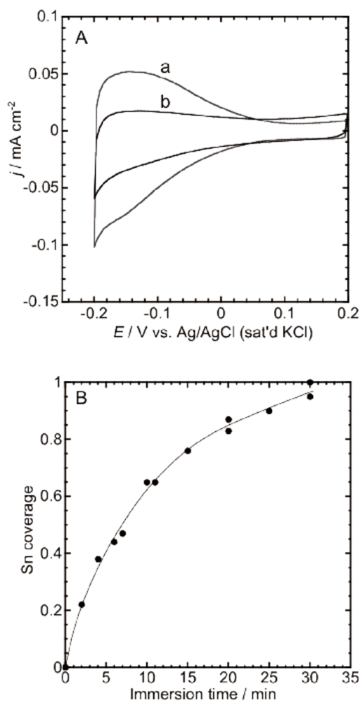
Figure 5.3 (A) CVs of PtRh electrodes in 0.1 M \text{HClO}_4 at a scan rate of 0.05 \text{ V s}^{-1} (a) before and (b) after the immersion in 0.1 M \text{HClO}_4 solution containing 0.12 mM \text{SnCl}_2 for 20 mins. The surface composition of Pt/Rh was 24/76. (B) Plot of immersion time dependence Sn coverage on Sn/PtRh electrodes.
