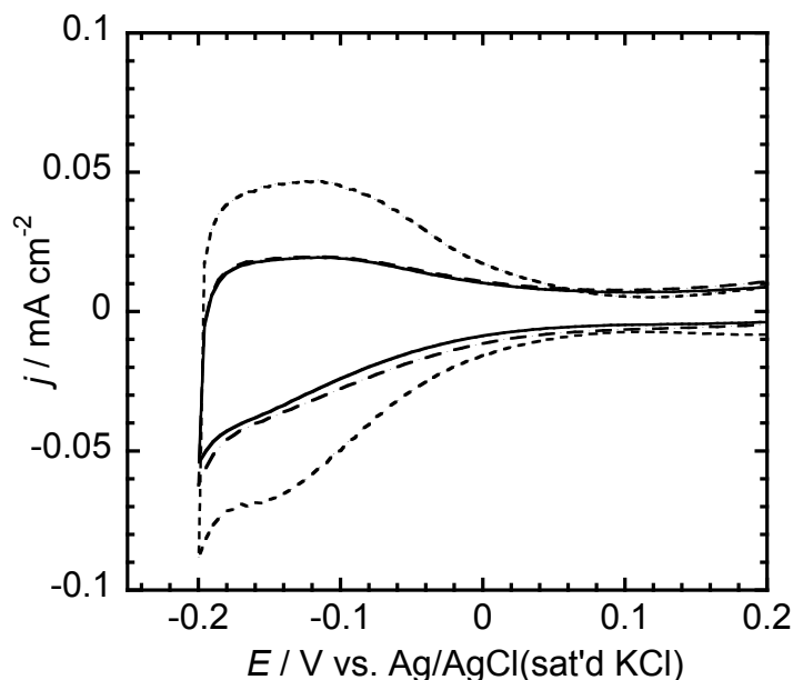
Figure 5.9 Cyclic voltammograms of (dotted curve) PtRh, (dashed curve) as-prepared Sn/PtRh, and (solid curve) pretreated Sn/PtRh electrodes in 0.1 M HClO 4 at the scan rate of 0.05 V s -1 . Tin was adsorbed by immersing a PtRh electrode in a 0.12 mM SnCl 2 solution for 15 min. The tin coverage was 0.78. The electrochemical pretreatment was conducted at -0.35 V for 60 s.
