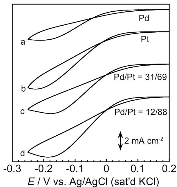
Figure 4.7 Reduction of nitrate in 0.01 M NaNO 3 + 0.1 M HClO 4 on Sn modified (a) Pd, (b) Pt, (c ) PdPt (Pd/Pt = 31/69) and (d) PdPt (Pd/Pt = 12/88) electrodes. The Sn coverage was 0.80-0.82 and the scan rate was 0.01 V s -1 .
