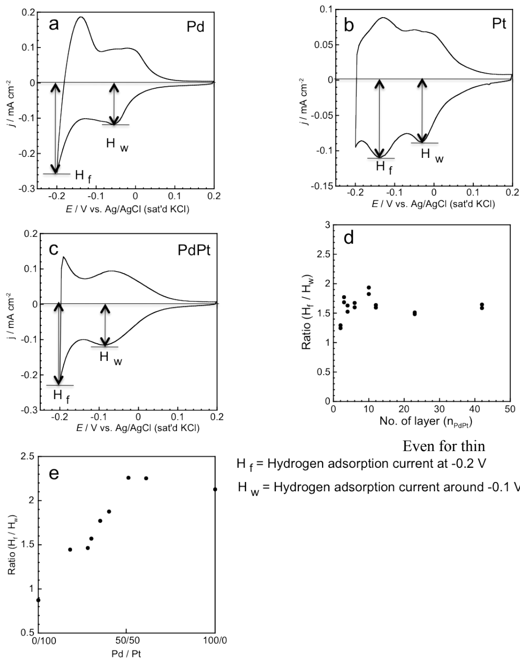
Figure 4.11 Cyclic voltammograms of Pd (dep), Pt (dep) and PdPt(dep, Pd/Pt = 31/69) in 0.1 M HClO 4 at a scan rate of 0.05 V s -1 . (d) Thickness dependence hydrogen adsorption behavior (Pd/Pt = 30/70) and (e) and composition dependence adsorption behavior of PdPt(dep) electrodes.
