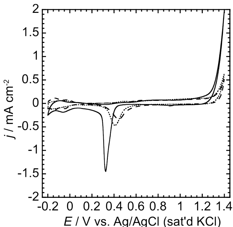
Figure 4.1. Cyclic voltammogram Pd (solid line) , Pt (dash line) and PdPt (dot line) in 0.1 M HClO 4 . Scan rate: 50 mV s -1 . The surface composition of Pd/Pt was 30/70.
