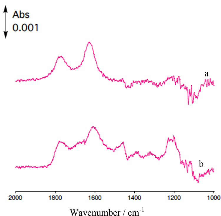
Figure 5.8 The SEIRA spectra of \text{NO}_3^- on (a) Sn/Rh ( \theta_{\text{Sn}} = 0.45 ) (b) Sn/PtRh ( \theta_{\text{Sn}} = 0.93 ) electrodes in 0.1 M \text{HClO}_4 . The adsorption was conducted at 0.2 V. The surface composition was Pt/Rh = 43/57.
