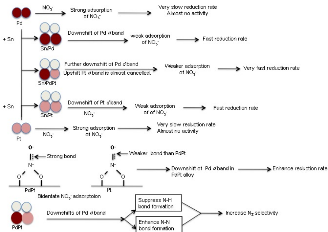
Scheme 6.2: Schematic representation of PdPt electrodes for nitrate reduction and \text{N}_2 selectivity.
