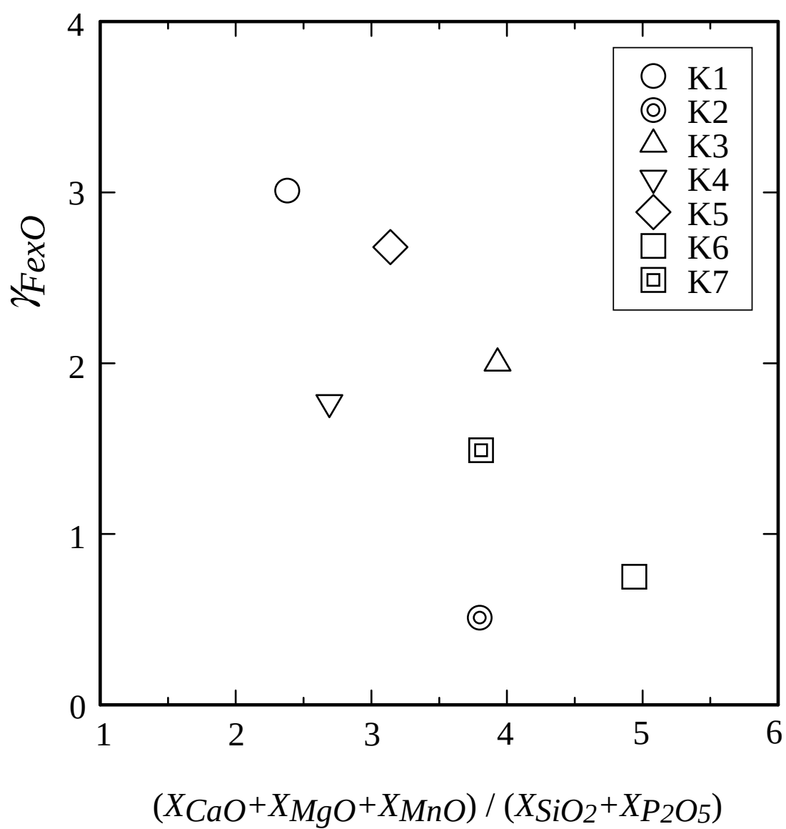
Figure 3.7 Activity coefficient of FeO as the function of (X_{\text{CaO}} + X_{\text{MgO}} + X_{\text{MnO}}) / (X_{\text{SiO}_2} + X_{\text{P}_2\text{O}_5}) at 1673K.
