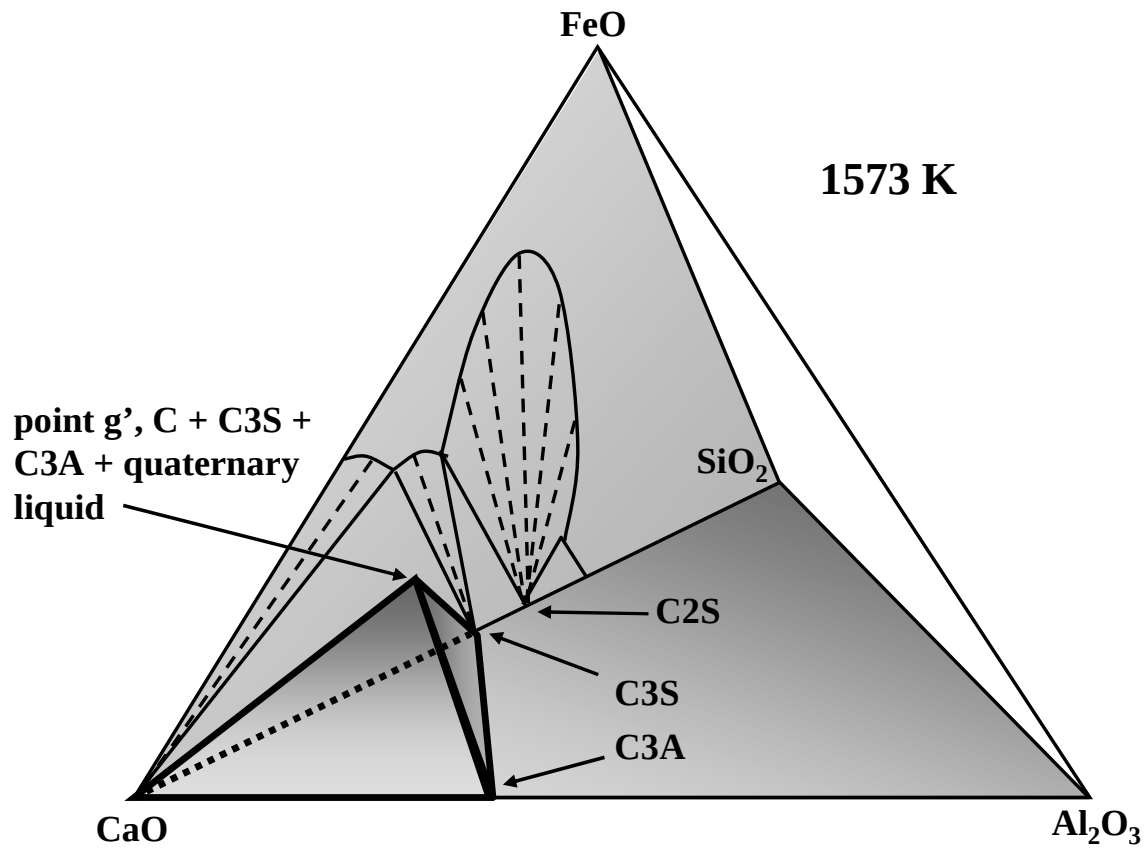
Figure 2.3(a) A schematic illustration of the iso-thermal tetrahedron of the system CaO - SiO 2 - Al 2 O 3 - FeO at 1573 K, showing 4-phase assemblage of C + C3S + C3A + quaternary liquid.
