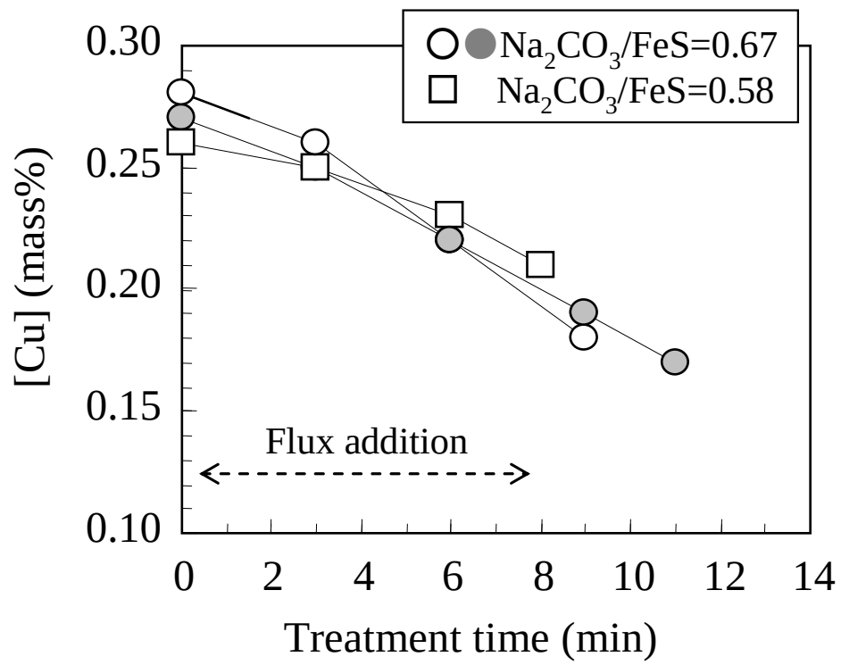
Figure 6.9 Change of [Cu] with treatment time with the addition of \text{Na}_2\text{CO}_3 and FeS fluxes at 3-ton hot metal experiment.
