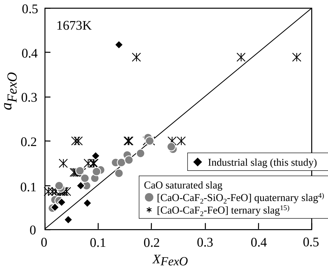
Figure 3.11 Activities of FeO as the function of X_{FeO} for heterogeneous slags at 1673K.
