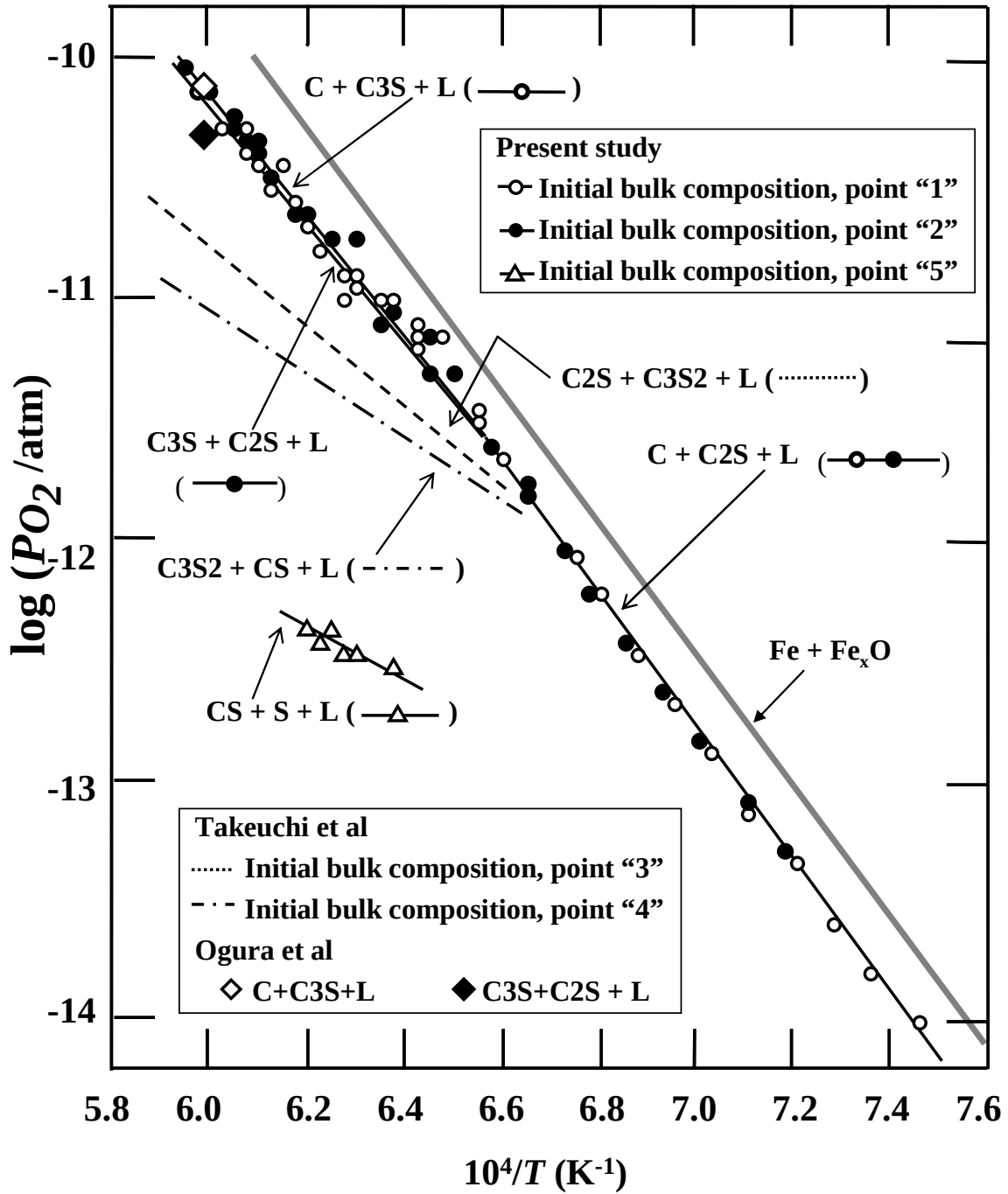
Figure 2.9 Relation between \log P_{O_2} and 1/T in comparison with the literature data for three-phase assemblages of C + C3S + L and C3S + C2S + L by Ogura et al 12) , for C2S + C3S2 + L (line C) and C3S2 + CS + L (line D) by Takeuchi et al 3) , and for Fe + Fe x O by Spencer and Kubaschewski 11) , and Hoshino and Iwase 9) .
