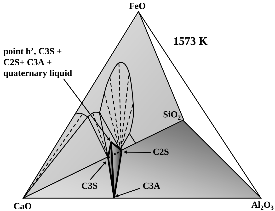
Figure 2.3(b) A schematic illustration of the iso-thermal tetrahedron of the system CaO - SiO 2 - Al 2 O 3 - FeO at 1573 K, showing 4-phase assemblage of C3S + C2S + C3A + quaternary liquid.
