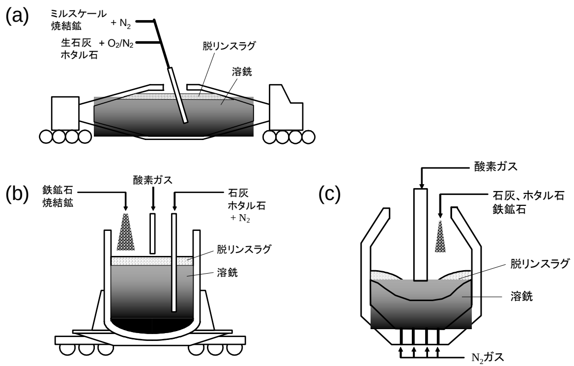
Figure 1.4 溶銑脱リン設備
