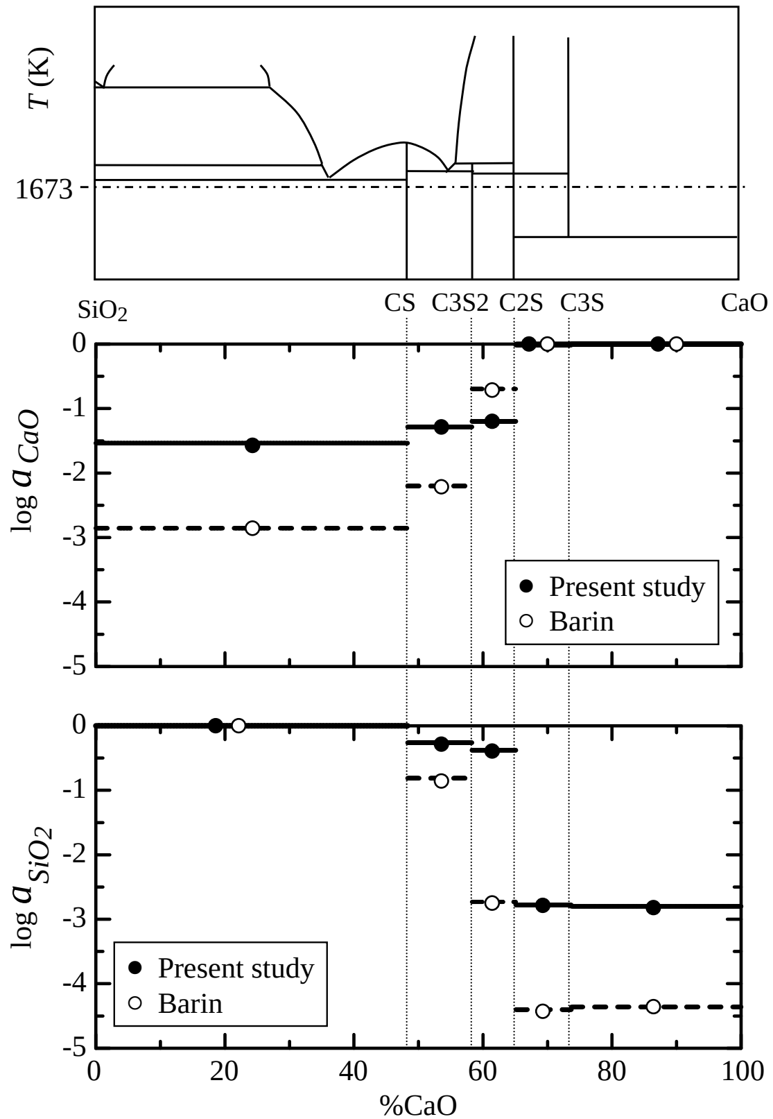
Figure 2.12 Activities of \text{SiO}_2 and \text{CaO} derived from graphical integration in this study in comparison with the literature data 13) derived from the free energy of formation of double oxides from oxides.
