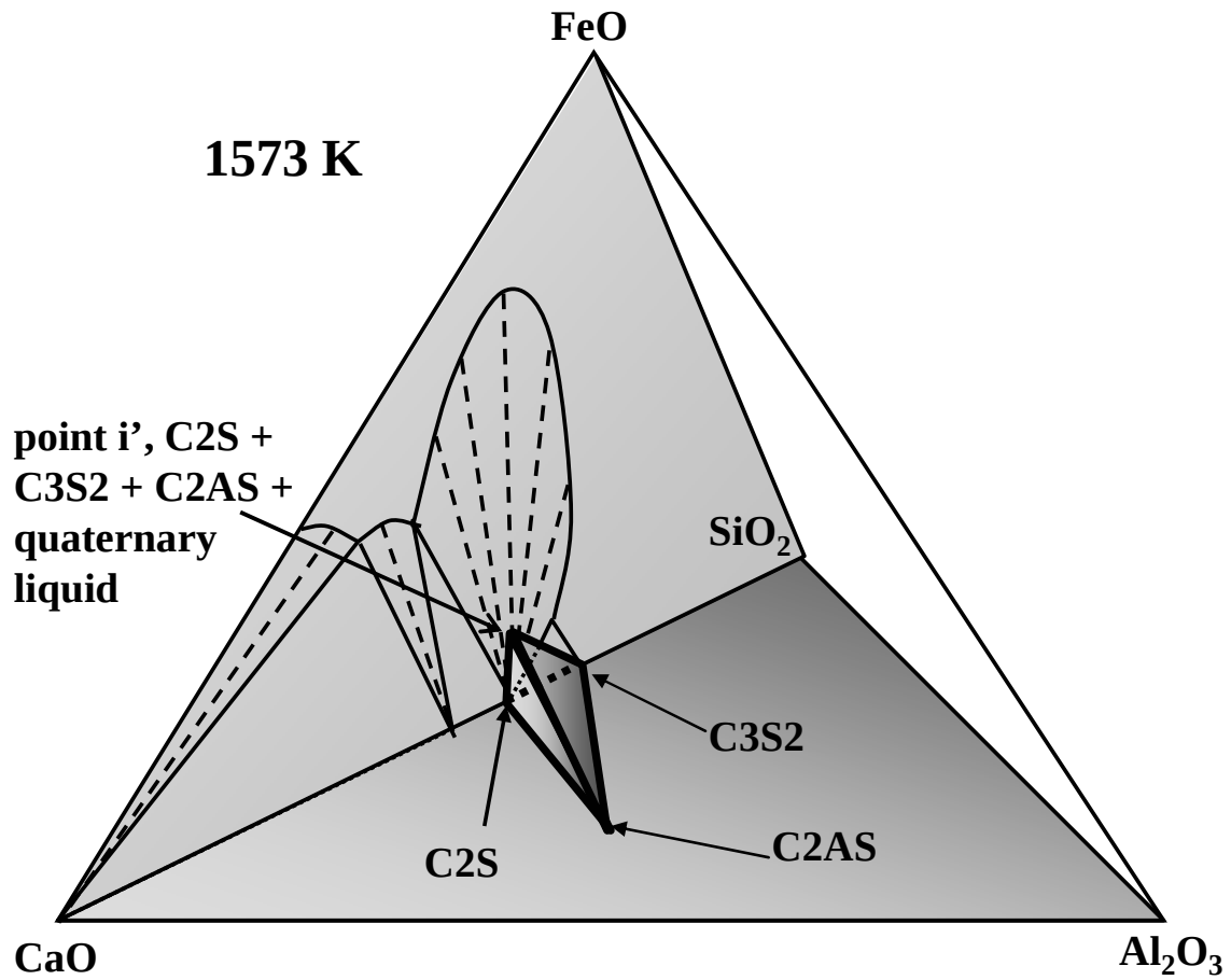
Figure 2.3(c) A schematic illustration of the iso-thermal tetrahedron of the system CaO - SiO 2 - Al 2 O 3 - Fe x O at 1573 K, showing 4-phase assemblage of C2S + C3S2 + C2AS + quaternary liquid.
