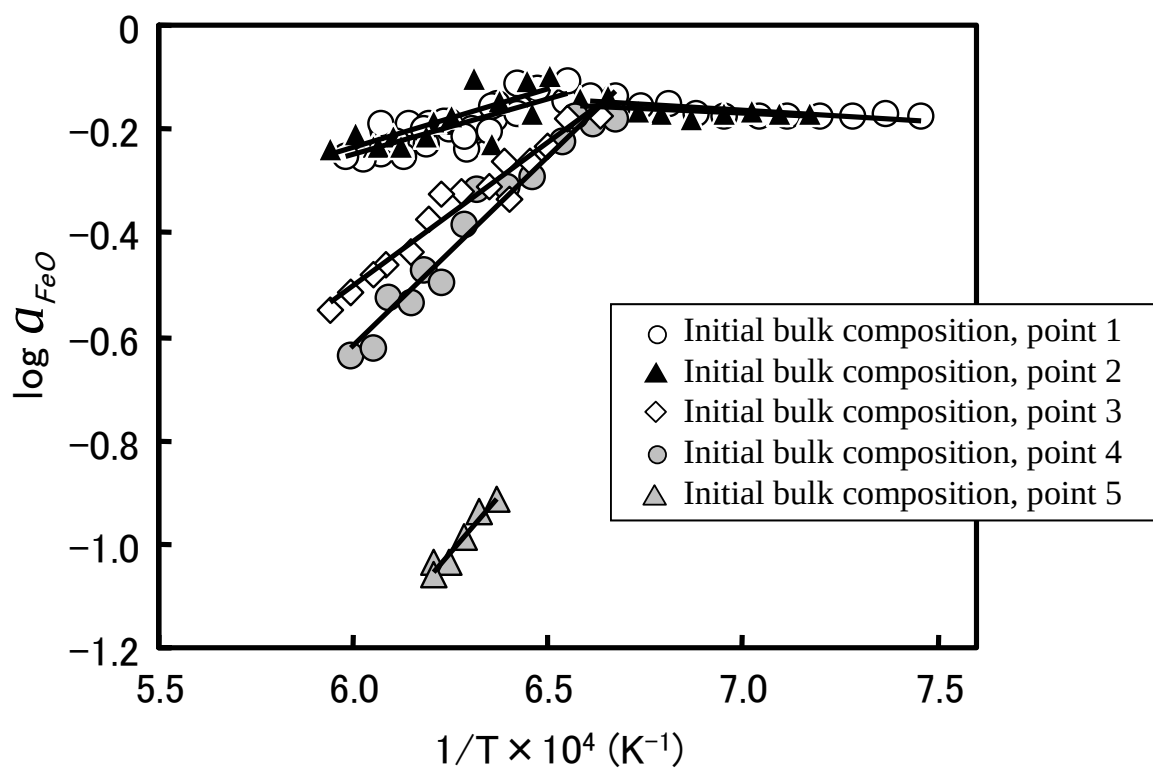
Figure 2.10 Relation between the activities of FeO and reciprocal temperature for three-phase assemblages in [CaO-SiO 2 -Fe x O] ternary slag .
