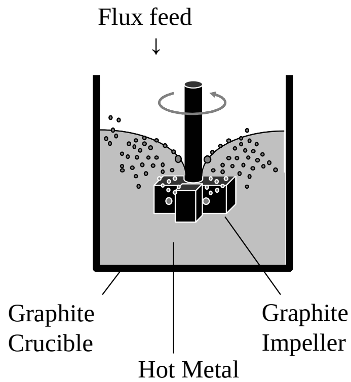
Figure 5.1 Experimental setup.
