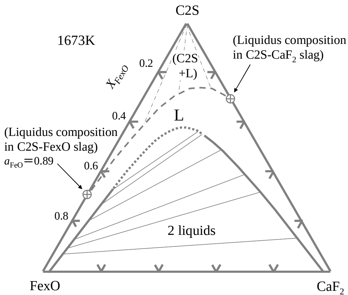
Figure 3.14 Phase diagram of the C2S- \text{CaF}_2 -FexO pseudo-ternary system at 1673K. 18)
