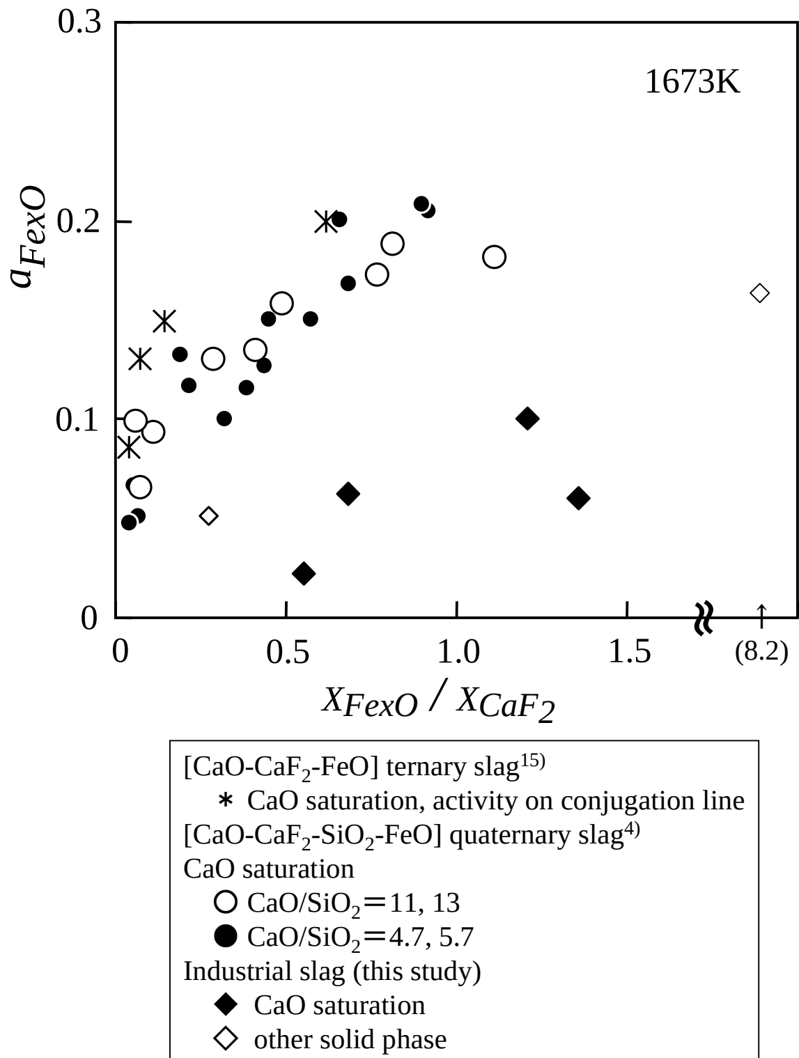
Figure 3.13 Activities of FeO as the function of X_{FeO} / X_{CaF_2} for heterogeneous slags at 1673K.
