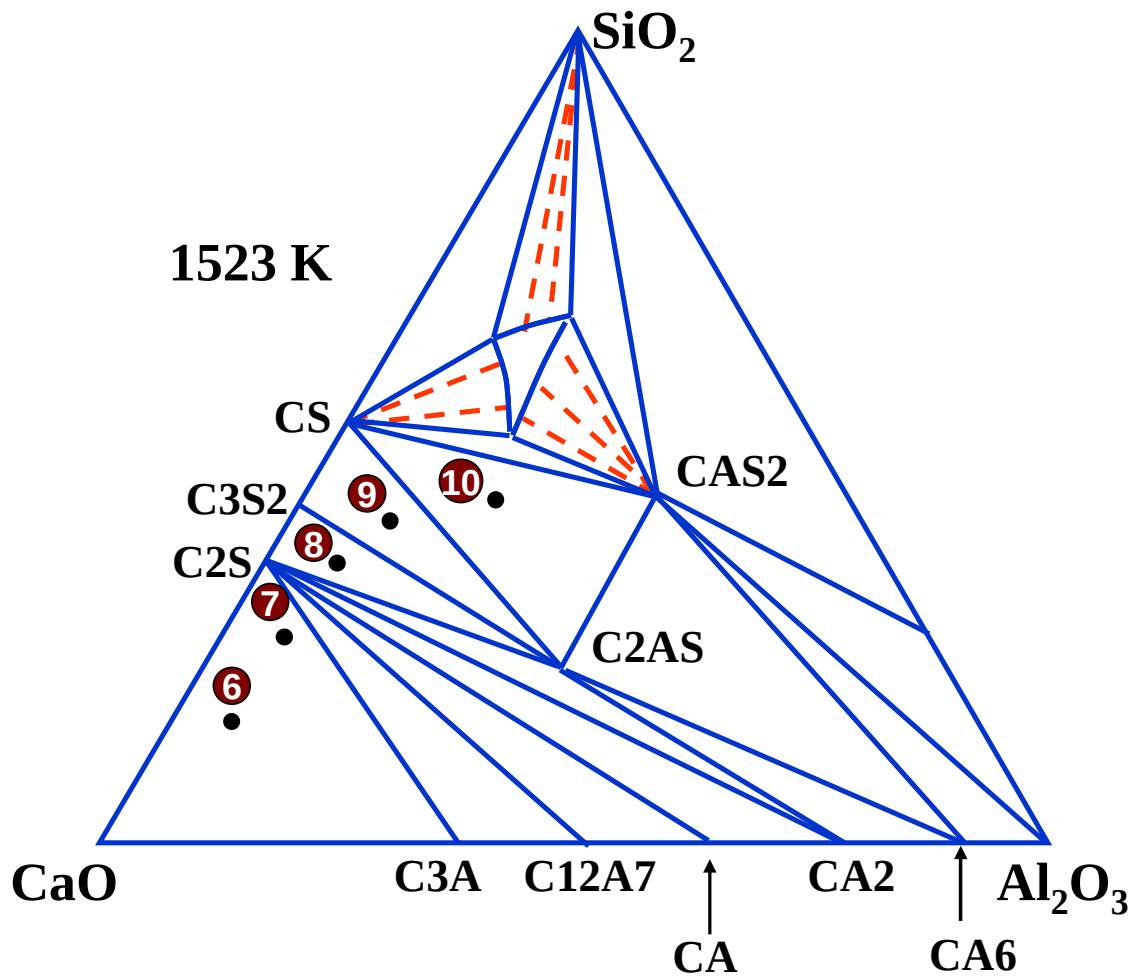
Figure 2.2(b) Iso-thermal section of the phase diagram of the system \text{CaO} - \text{SiO}_2 - \text{Al}_2\text{O}_3 at 1523K drawn on projection of the phase diagram given by Muan and Osborn 1) . Compositions are given by pct by weight.
