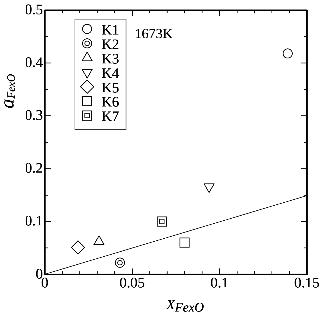
Figure 3.5 Activities of FexO as the function of X_{FexO} at 1673K.
