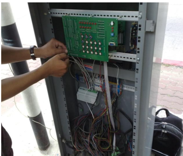
Picture 5.2 the Installed Traffic Controllers at the Intersections
