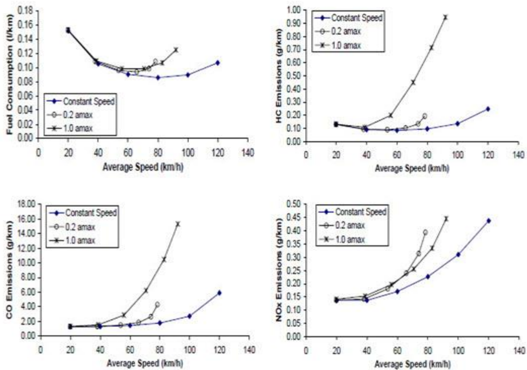
Figure 2.11 Impact of Level of Acceleration in HC Emission Rate as a Function of Average Speed (Distance = 4.5 km, Deceleration Rate for Single-Stop Cycles = -0.5 m/s 2 )
