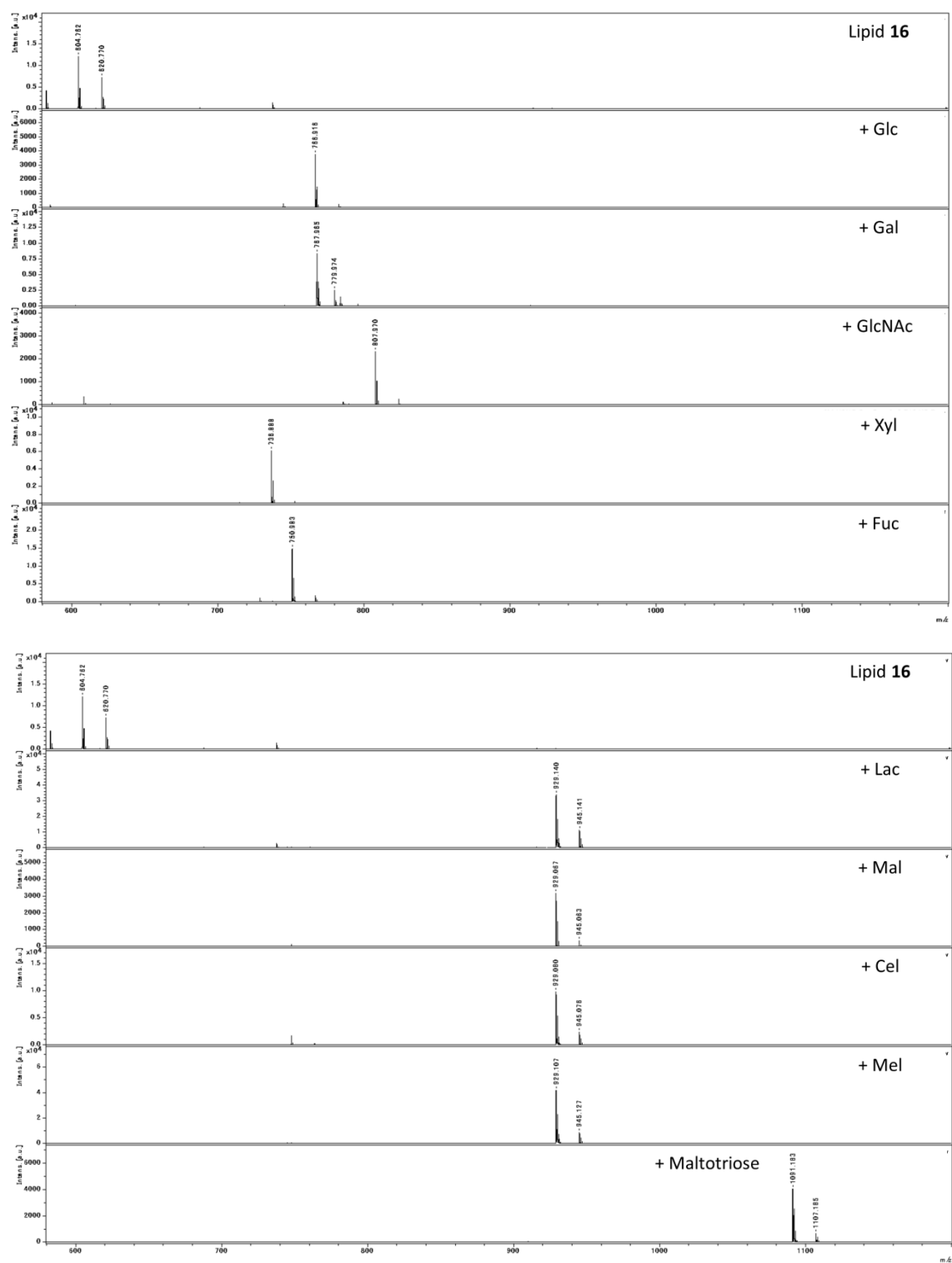
Fig. 3-2-12. MALDI-TOF MS spectra of conjugated products using compound 16
