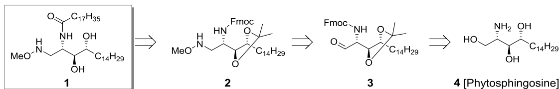
Figure 2-2-1. Design and retrosynthetic analysis of ceramide derivative 1
