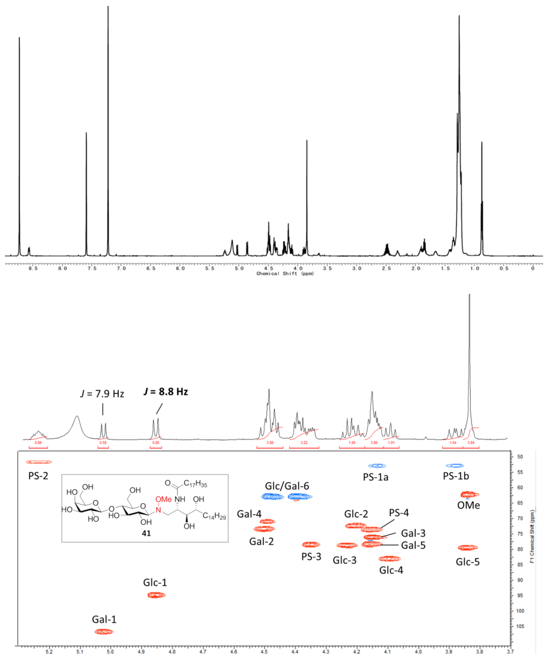
Fig. 3-2-1. NMR spectra of the conjugated product 41
