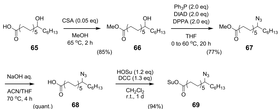
Scheme 5-2-1. Synthesis of succinimidyl 12-N 3 -octadecanoate 69
