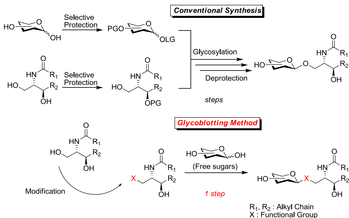
Fig. 2-1-1. Comparison of glycoblotting method with conventional method for synthesis of glycolipid derivatives.
