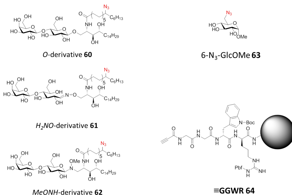
Fig. 5-2-1. Target compounds
