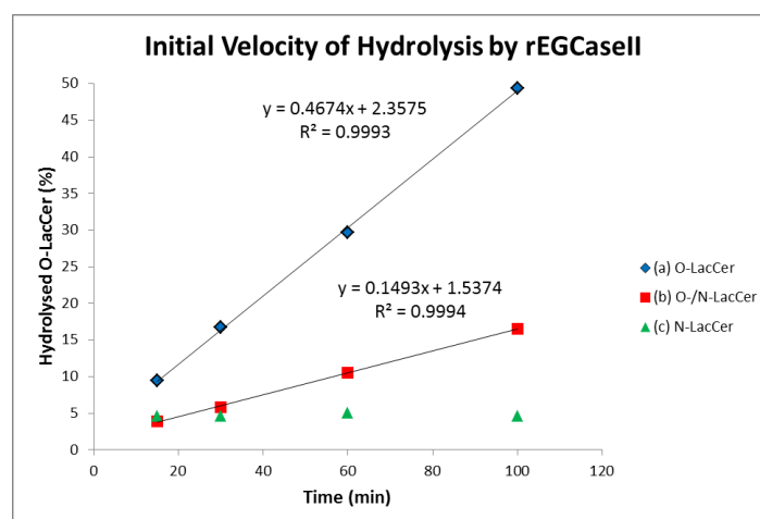
Figure 4-2-5. Inhibitory effect of lactosylceramide mimic 41 (N-LacCer) on the hydrolytic activity of recombinant EGCase II. Initial velocity of the hydrolysis of O-LacCer 53 was determined by quantitating lactose released from O-LacCer using modified Park and Johnson method (Supporting Information). ◆: O-LacCer (450 \mu M), ■: O-LacCer (450 \mu M) and N-LacCer (270 \mu M), ▲: N-LacCer (735 \mu M); Reaction condition: 20 mM AcOH buffer (pH 4.7), 0.4% Triton X-100, EGCase II (12 mU/mL), 37°C.
