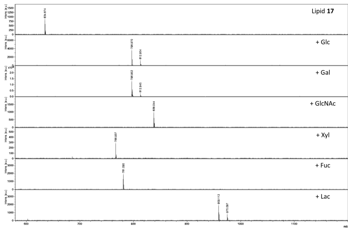
Fig. 3-2-9. MALDI-TOF MS spectra of conjugated products using compound 17
