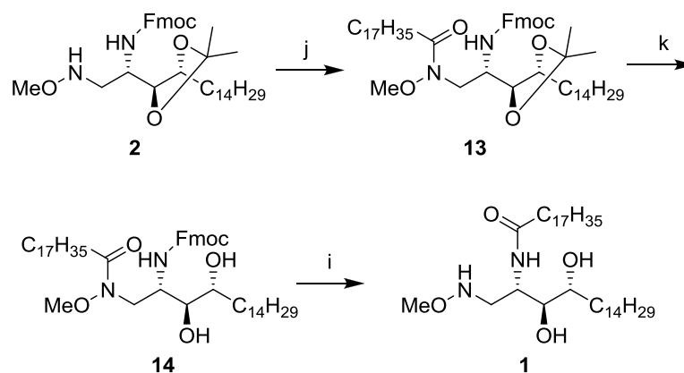
Scheme 2-2-2. Synthesis of ceramide derivative 1 via acyl migration reaction; j) \text{H}_{35}\text{C}_{17}\text{COOSu} , THF/pyr (2:1), 50 °C, 2 d, 82%; k) TFA, \text{CH}_2\text{Cl}_2/\text{H}_2\text{O} (10:1), RT, 30 min, 57%; i) piperidine, THF, RT, 3 h, 66%
