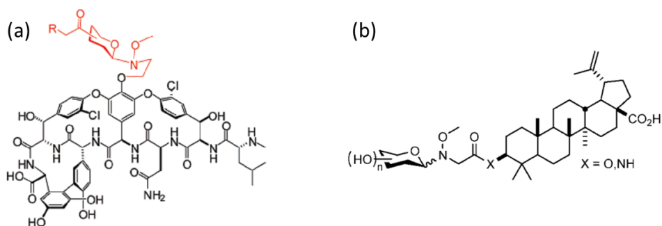
Fig. 1-5. Reported glycoconjugates synthesized by glycoblotting reaction
