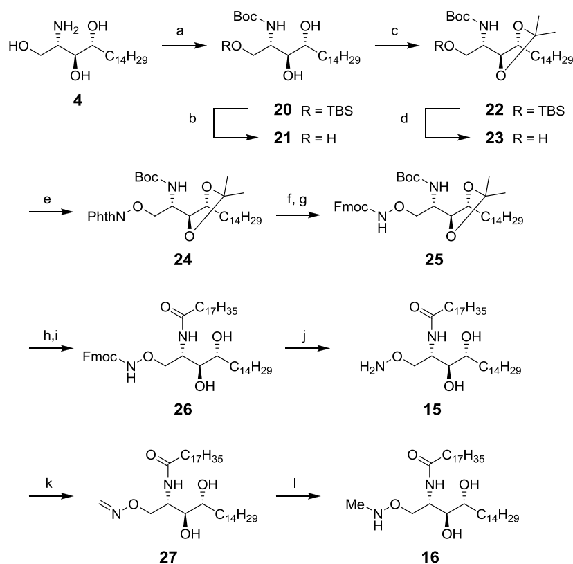
Scheme 2-2-3. Synthesis of ceramide derivative 15 and 16 . Reagents and conditions: a) Boc 2 O, NaHCO 3 , THF, RT, 3.5 h, quantitatively; b) TBSCl, imidazole, DCM, RT, 1 h, 92%; c) 2-methoxypropane, CSA, THF, RT, 2 h, 88%; d) TBAF, THF, RT, 2 h, 90%; e) HONPhth, Ph 3 P, DIAD, THF, 50 °C, 9 h, 95%; f) MeNH 2 , THF/MeOH, 7 h; g) FmocOSu, THF, RT, 9 h, 82%, 2 steps; h) TFA, DCM, H 2 O, RT, 40 min; i) H 35 C 17 COOSu, THF, RT, 2 d, 75%, 2 steps; j) piperidine, THF, RT, 6 h, 66%; k) HCHO, DCM, MeOH, AcOH, RT, overnight, 81%; l) NaBH 3 CN, AcOH/THF (4:1), RT, 1 h, 80%.
