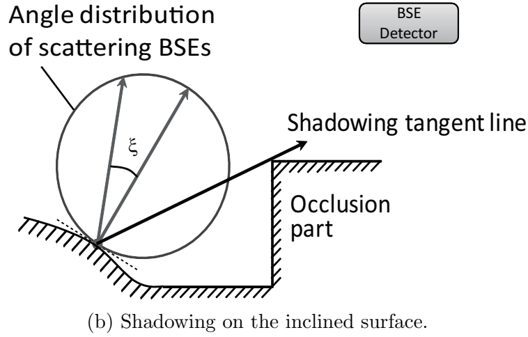
Figure 5.1: Shadowing effects. BSEs emitted in a direction below the shadowing tangent line are generally absorbed by the occlusion region and consequently are not collected by the detector.
