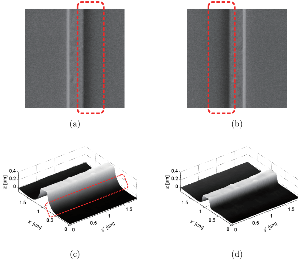
Figure 1.4: Shadowing effects in a line pattern: (a) original left image, (b) original right image, (c) reconstructed shape via the proposed variational method without de-shadowing, and (d) reconstructed shape via our proposed method with de-shadowing.
