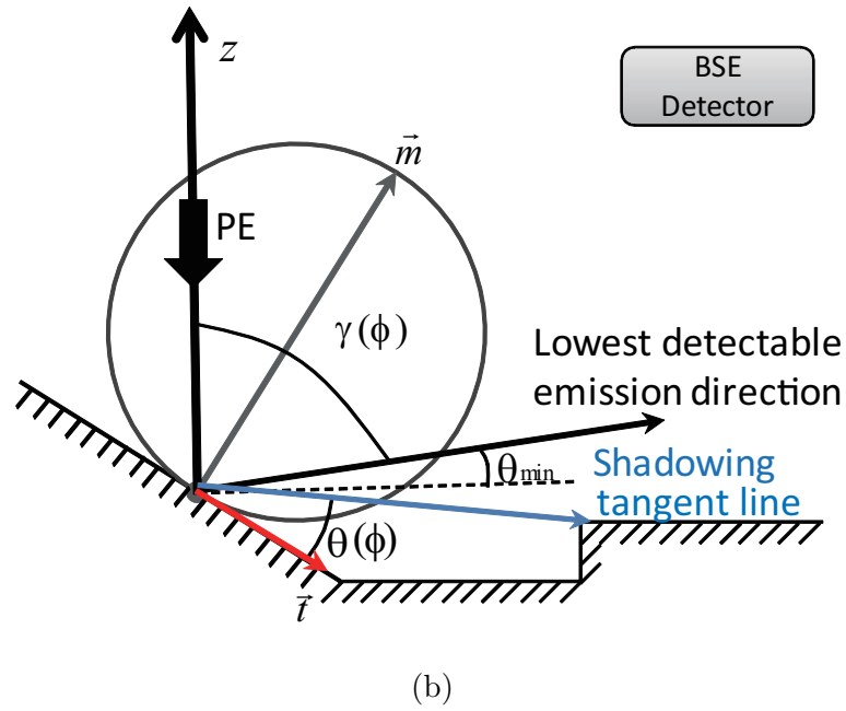
Figure 5.5: Zenith ranges in the presence of shadowing. (a) The upper limit of the zenith angle is up to the shadowing tangent line. (b) The upper limit of the zenith angle can only be up to the lowest detectable emission direction; electrons below this direction generally cannot be collected by a detector, which indicates no shadowing in fact.
