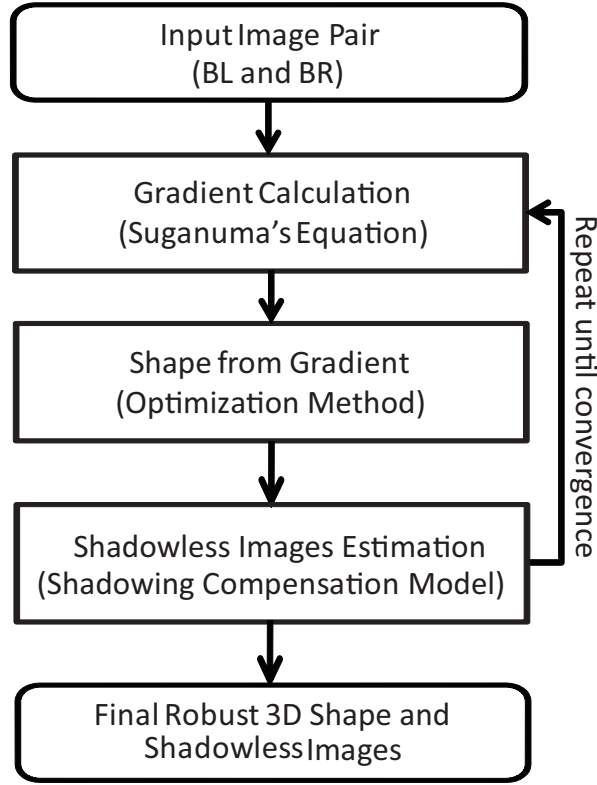
Figure 4.2: Iterative scheme for our proposed SEM photometric stereo.
