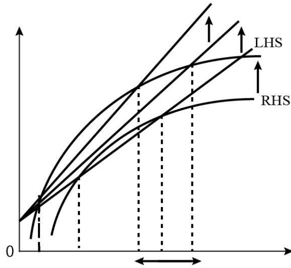
Figure 8: Effect of a change in \tau_1^r under 1+\gamma < \beta
