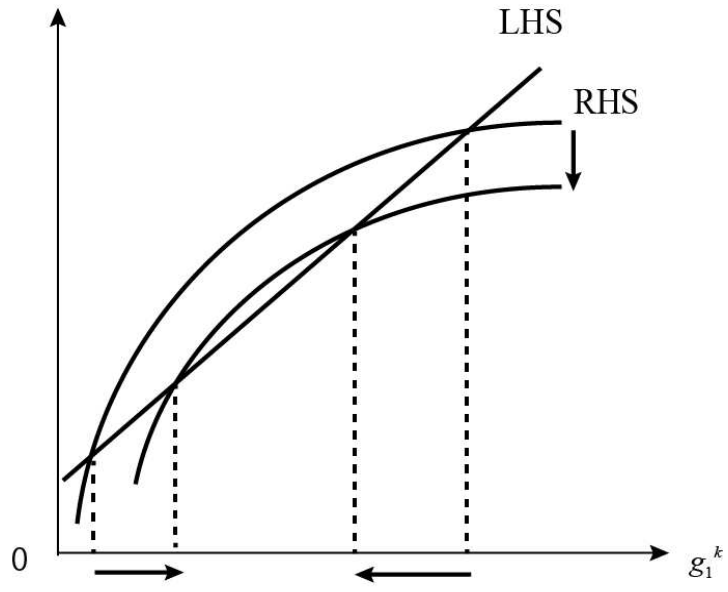
Figure 7: Effects of changes in \tau_1^e and \tau_1^w under 1+\gamma < \beta
