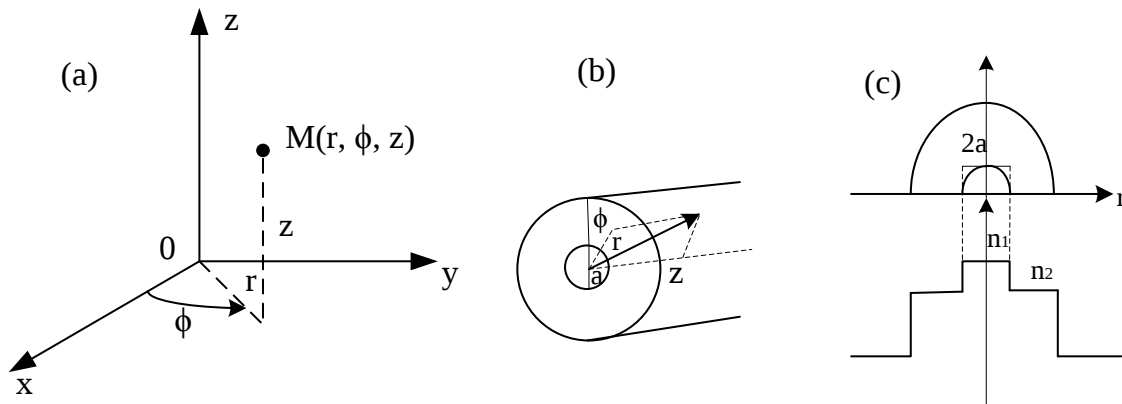
Fig. 2.3 (a) Cylindrical coordinate; (b) Geometry of a standard glass fiber; (c) The profile of its refractive index as a function of r .
