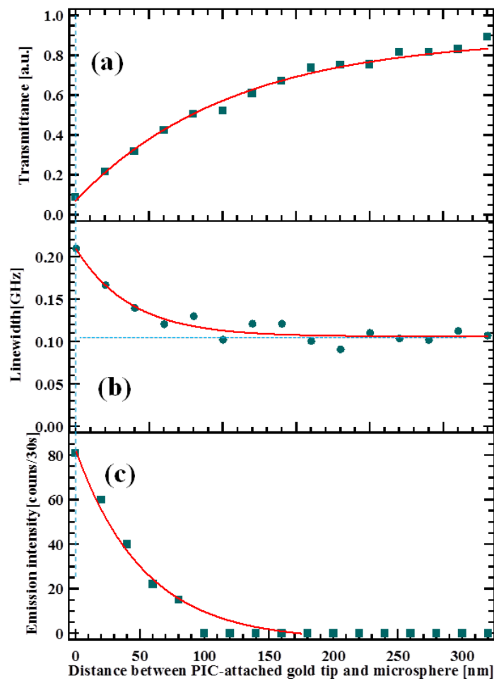
Fig. 5.5 (a) Transmittance, (b) linewidth of the resonant dip and (c) emission intensity at the apex of the PIC-attached Au-coated tip against the distance between the PIC-attached Au-coated tip and the microsphere surface.
