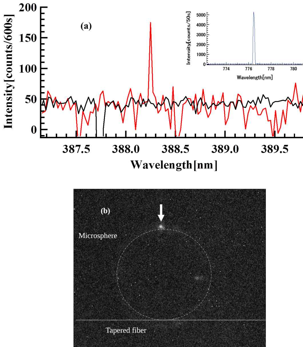
Fig. 4.4 (a): spectrum of SHG signal from the top of Au-coated tip and inset presents the spectrum of the scattered fundamental light. (b): CCD image of scattered light from an Au-coated tip via a tapered fiber coupled microsphere. White lines in the image indicate a microsphere and tapered fiber and an arrow indicate the scattered point of Au-coated tip.
