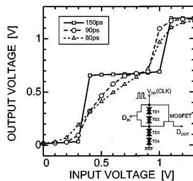
Fig. 11. Simulated input versus output characteristics of three-valued D-FF circuit for different clock rise time.
