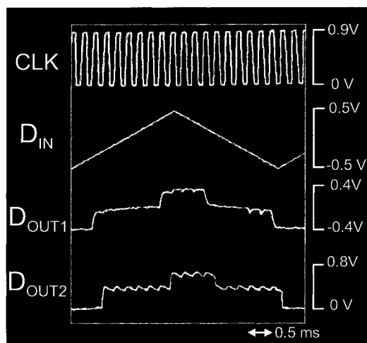
Fig. 10. Operation for three-valued shift register.
